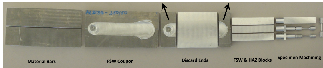
Figure 4-2: Specimen Manufacturing - Material Stock Thru Final Machining
