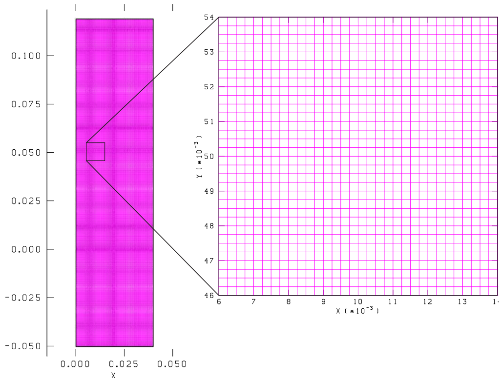
Figure 7: Computational mesh for uniform cell size=0.25 mm (Unit on axes: m).
