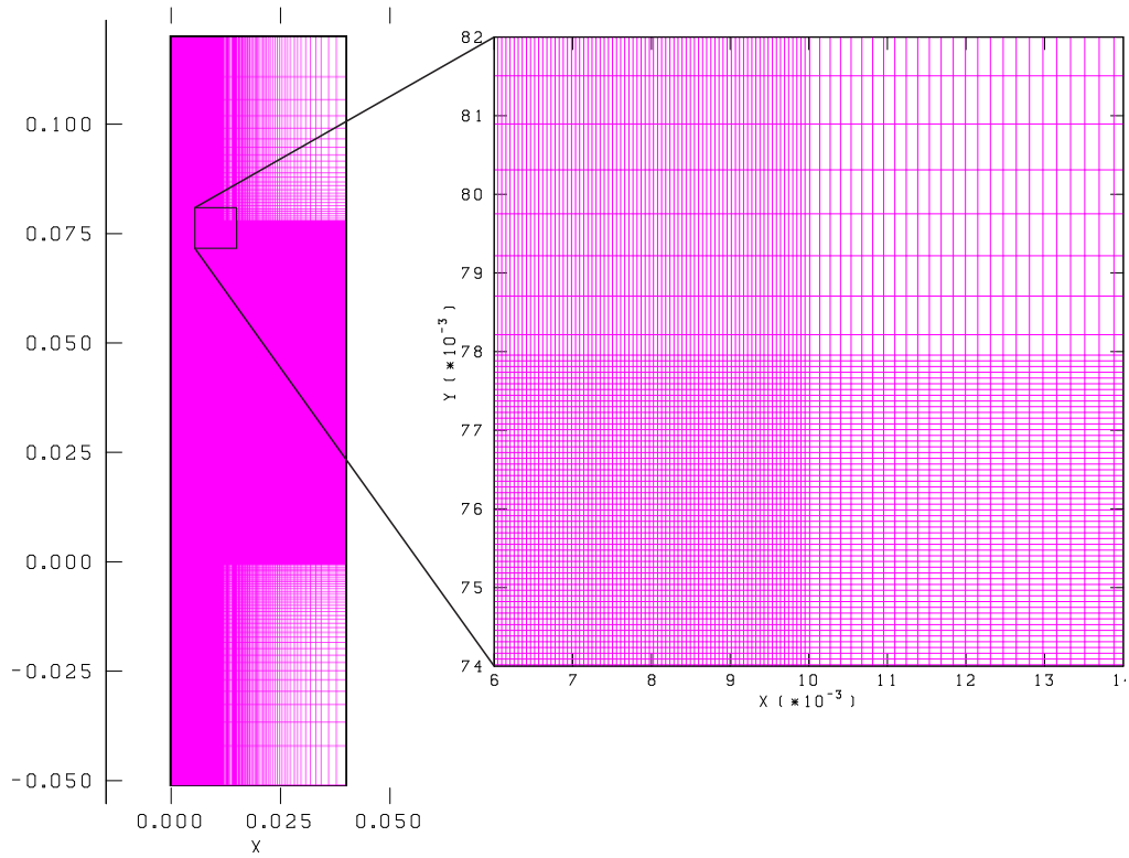
Figure 10: Computational mesh for graded cell size=0.15 mm (Unit on axes: m).
