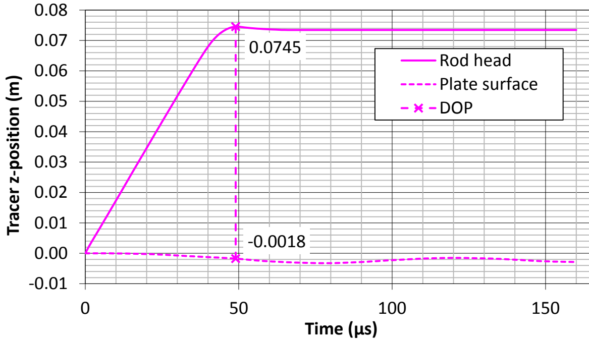
Figure 4: Calculation of DOP for the baseline case with V_{ROD}=3000 m/s.
