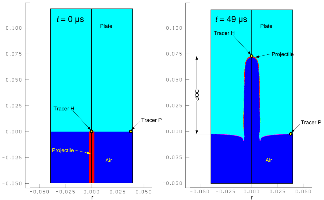
Figure 5: Simulation results at 0 and 49 μs for the baseline case with V_{ROD}=3000 m/s (Unit on axes is m).
