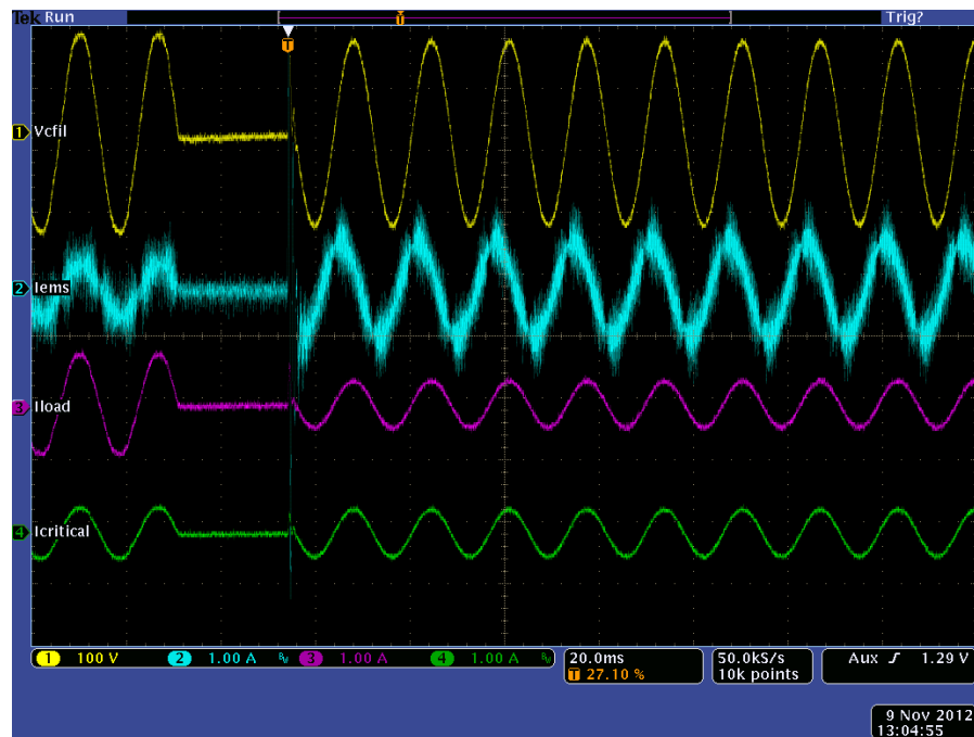
Figure 31. Experimental plots of the microgrid islanding and load shedding.
