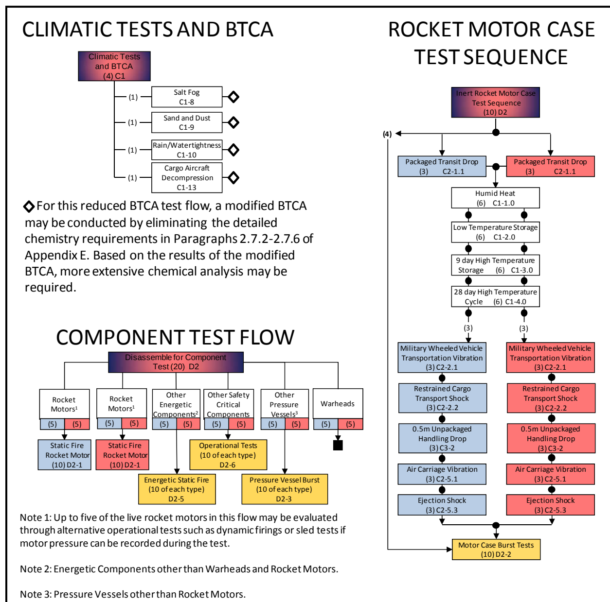
Figure B2-2. Detailed test flow charts for Analytical S3 Test Program with reduced BTCA.
