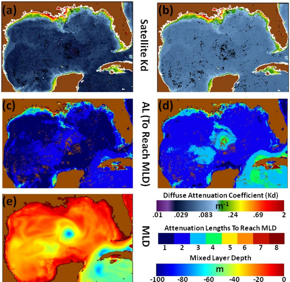
Figure 4. MODIS-Aqua 7-day-latest-pixel composites of (a) K_d at 490 nm and (b) K_d at 532 nm illustrating the satellite diffuse attenuation values coupled with the (e) MLD to determine the Attenuation Lengths at (c) 490 nm and (d) 532 nm necessary to reach the (e) MLD. This figure demonstrates a real-time capability for the utilization of space-borne LIDAR and how it is impacted by the ocean optical environment. A blue (490 nm) LIDAR, outperforms a blue-green (532 nm) LIDAR by penetrating deeper into the water column using less attenuation lengths --as exemplified by the deepening of the mixed layer (e) in the warm-core eddies clearly seen in the central Gulf.
