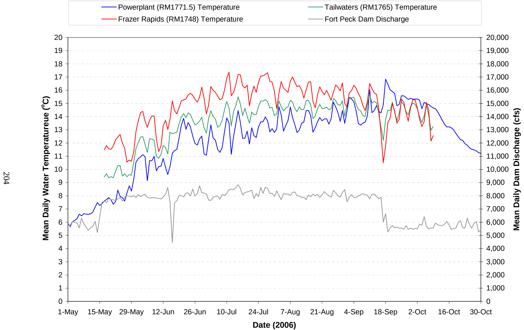
Plate 60. Mean daily water temperature monitored at the Fort Peck powerplant, Missouri River tailwaters, and Missouri River Frazer Rapids and the mean daily discharge of Fort Peck Dam from May through October during 2006.
