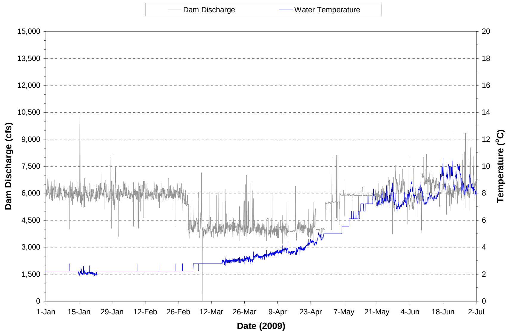
Plate 43. Hourly discharge and water temperature monitored at the Fort Peck powerplant on water discharged through the dam during the period January through June 2009.
