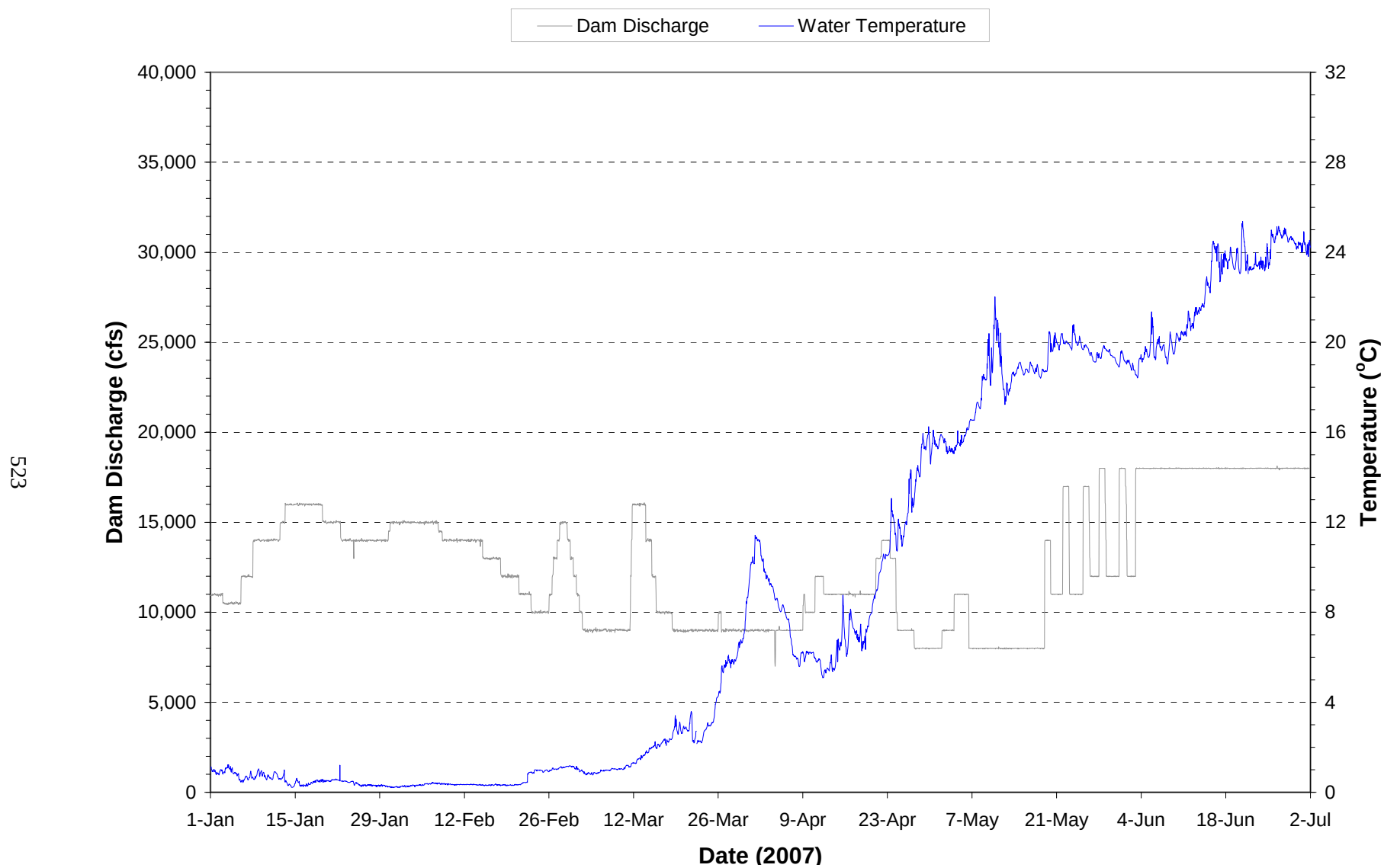
Plate 381. Hourly discharge and water temperature monitored at the Gavins Point powerplant on water discharged through the dam during the period January through June 2007.
