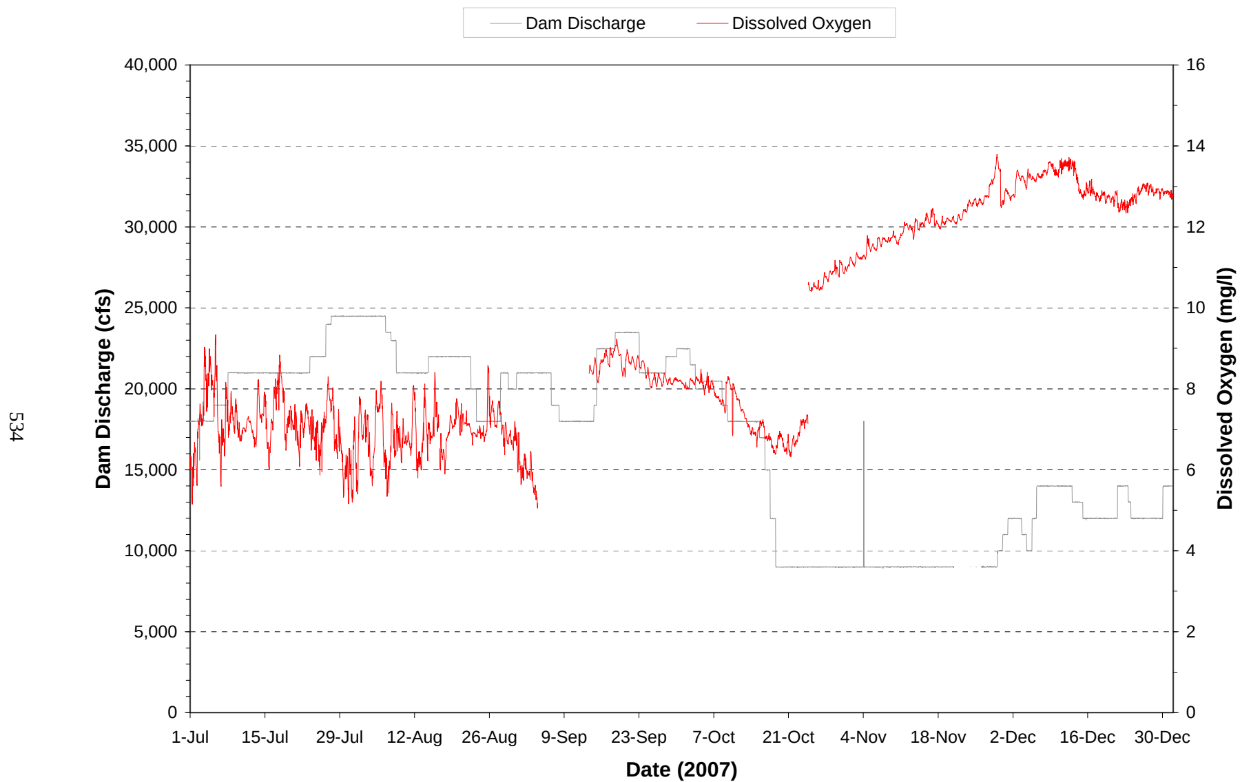
Plate 392. Hourly discharge and dissolved oxygen monitored at the Gavins Point powerplant on water discharged through the dam during the period July through December 2007. Note: Gaps in dissolved oxygen plot represents periods when monitoring equipment was not operational.
