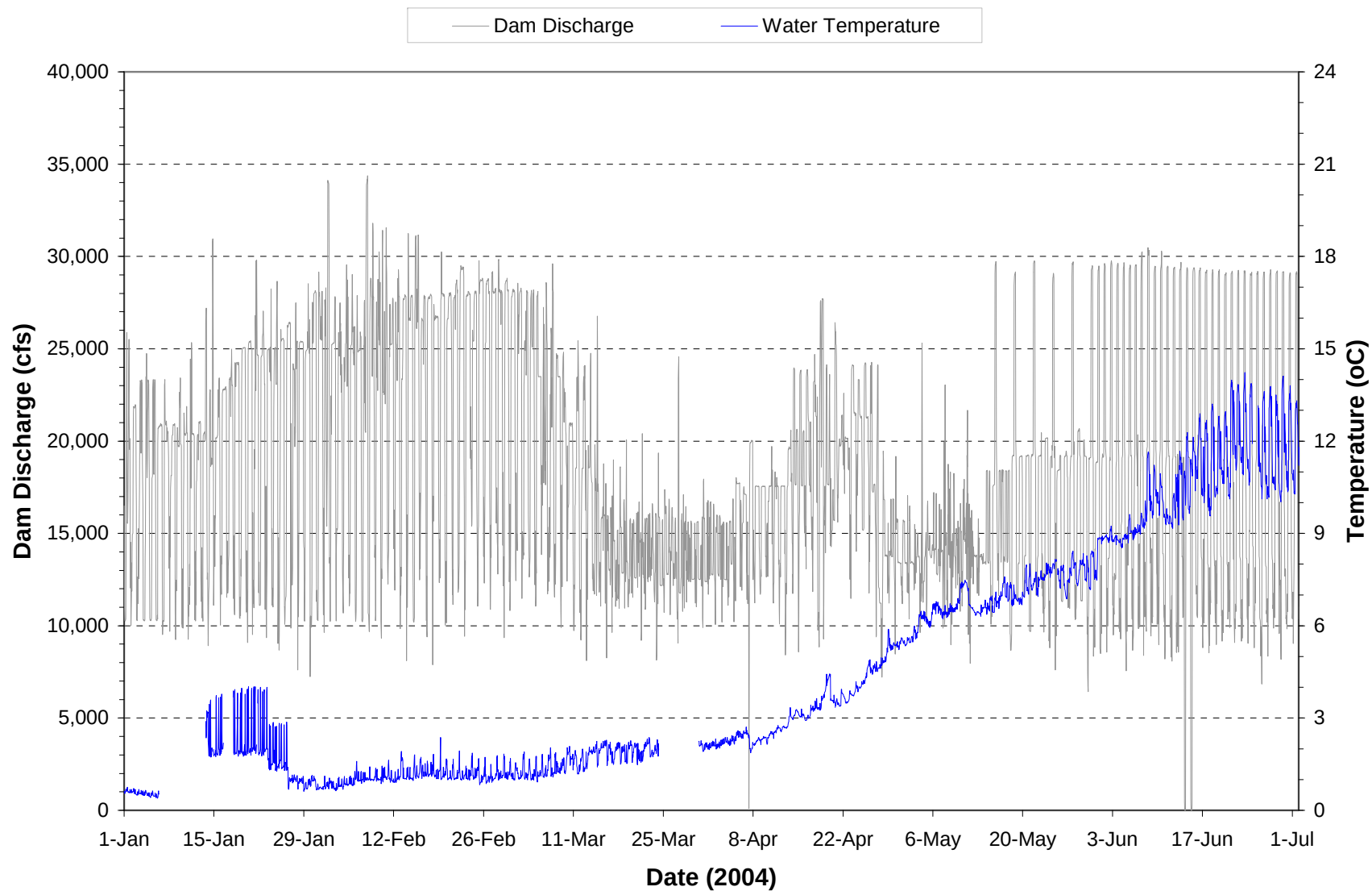
Plate 104. Hourly discharge and water temperature monitored at the Garrison powerplant on water discharged through the dam during the period January through June 2004.
