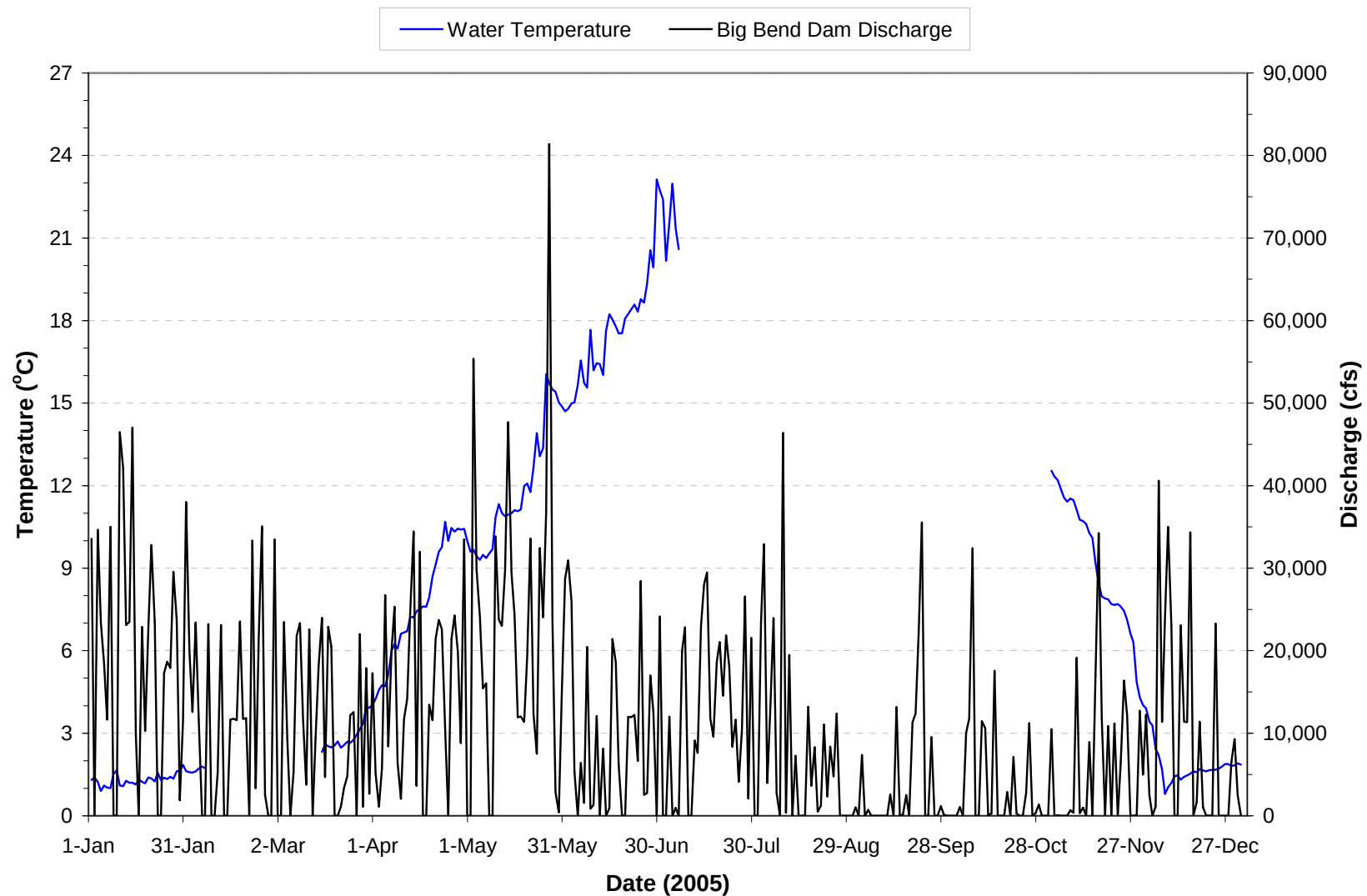
Plate 301. Mean daily water temperature and discharge of the Missouri River at Big Bend Dam (i.e., site BBDPP1) for 2005. Mean daily temperatures and discharges based on hourly measurements recorded on discharge through Big Bend Dam. (Note: Gaps in temperature plots are periods when monitoring equipment was not operational.)
