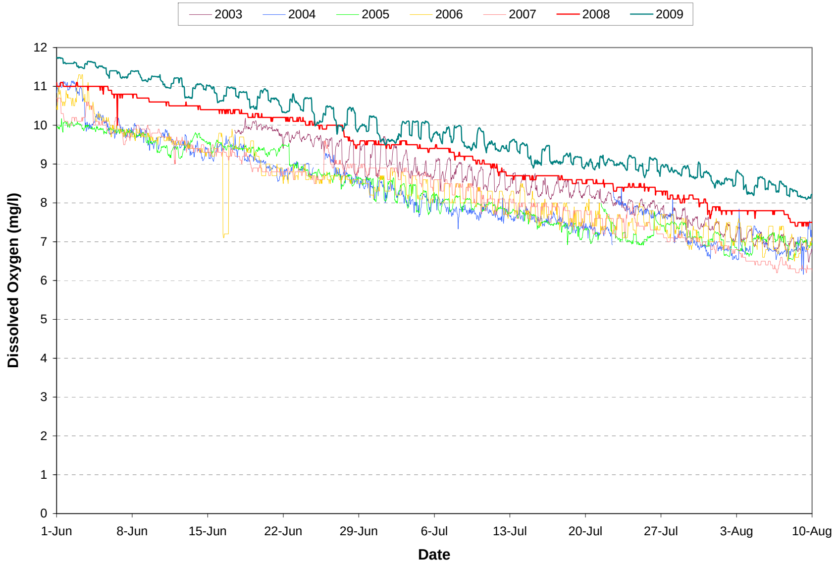
Plate 131. Hourly dissolved oxygen concentrations of water discharged through Garrison Dam during the period June through mid-August in 2003, 2004, 2005, 2006, 2007, 2008, and 2009.
