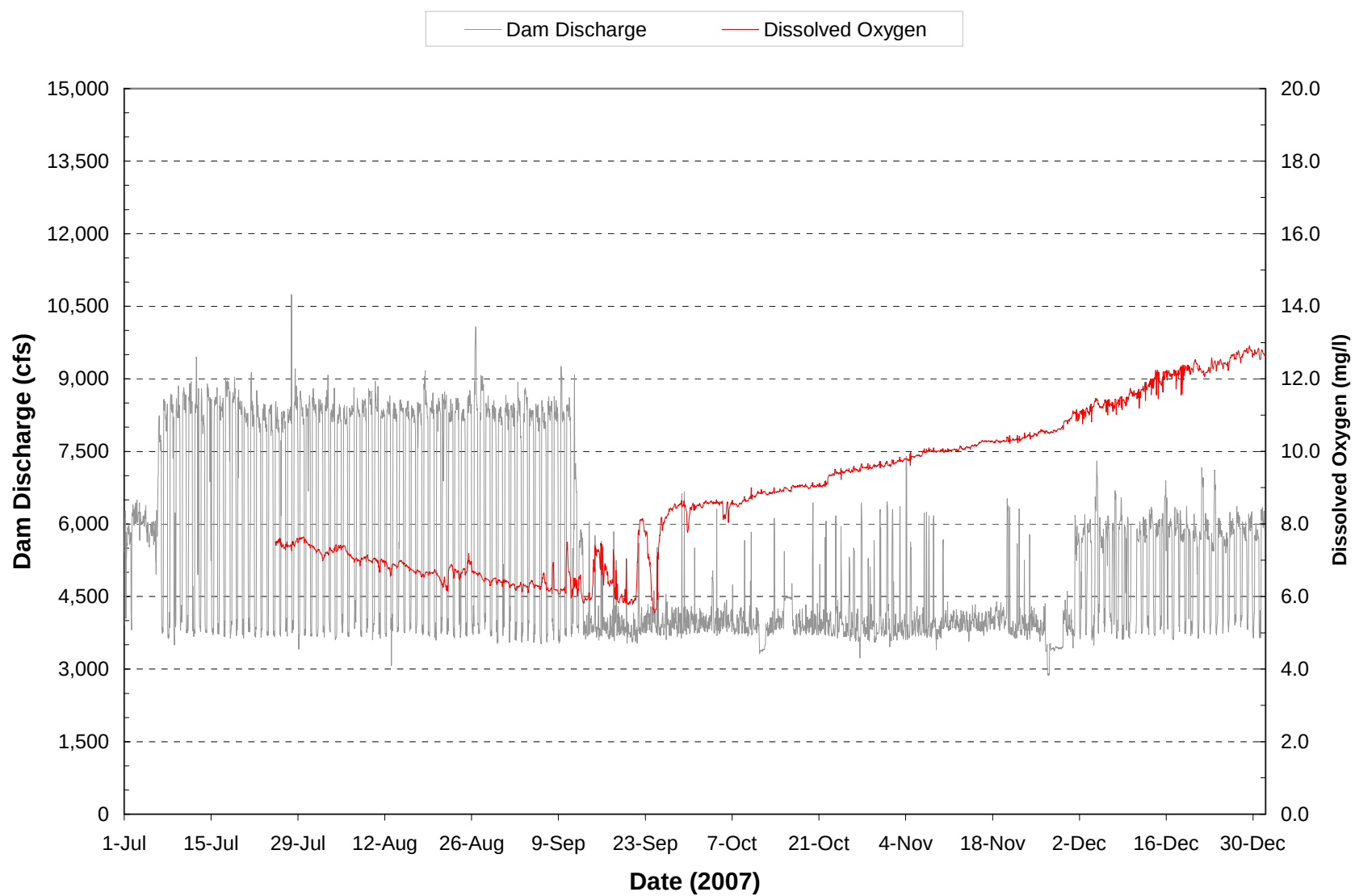
Plate 50. Hourly discharge and dissolved oxygen monitored at the Fort Peck powerplant on water discharged through the dam during the period July through December 2007. (Note: Gaps in dissolved oxygen plot represent periods when monitoring equipment was not operational.)
