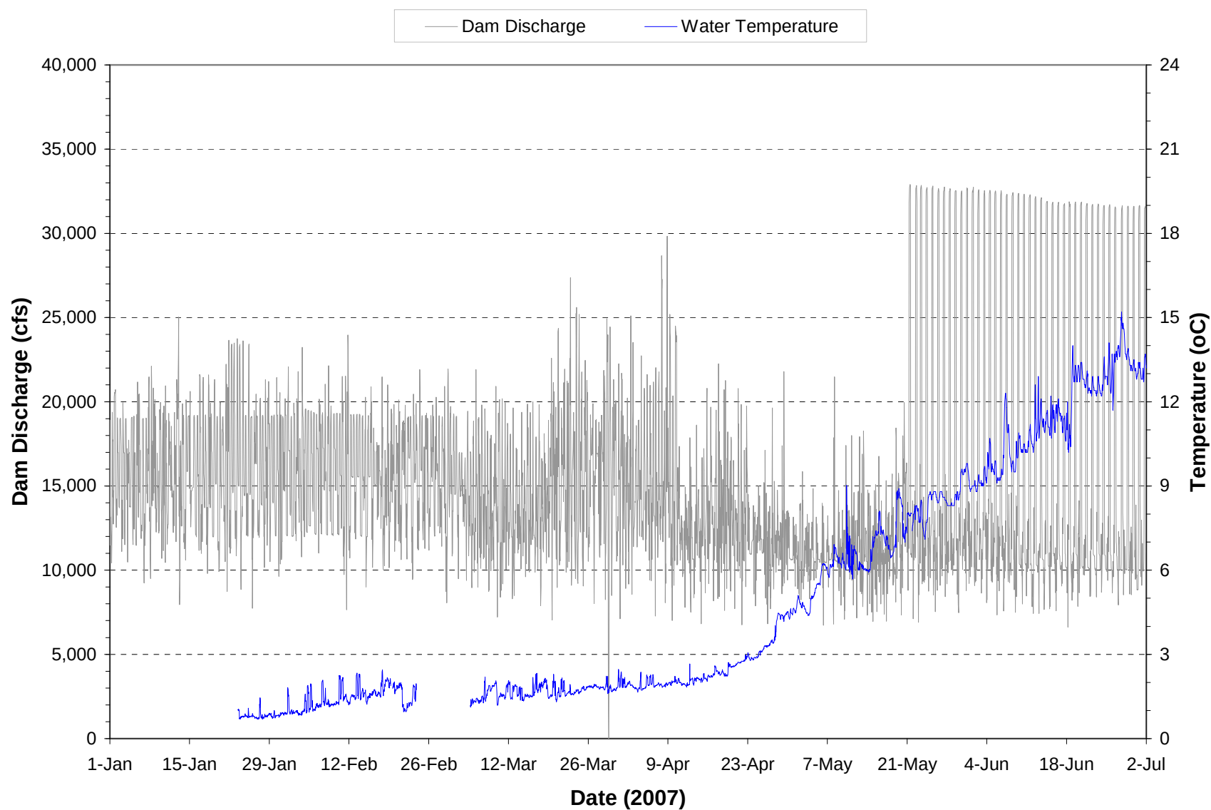
Plate 110. Hourly discharge and water temperature monitored at the Garrison powerplant on water discharged through the dam during the period January through June 2007.
