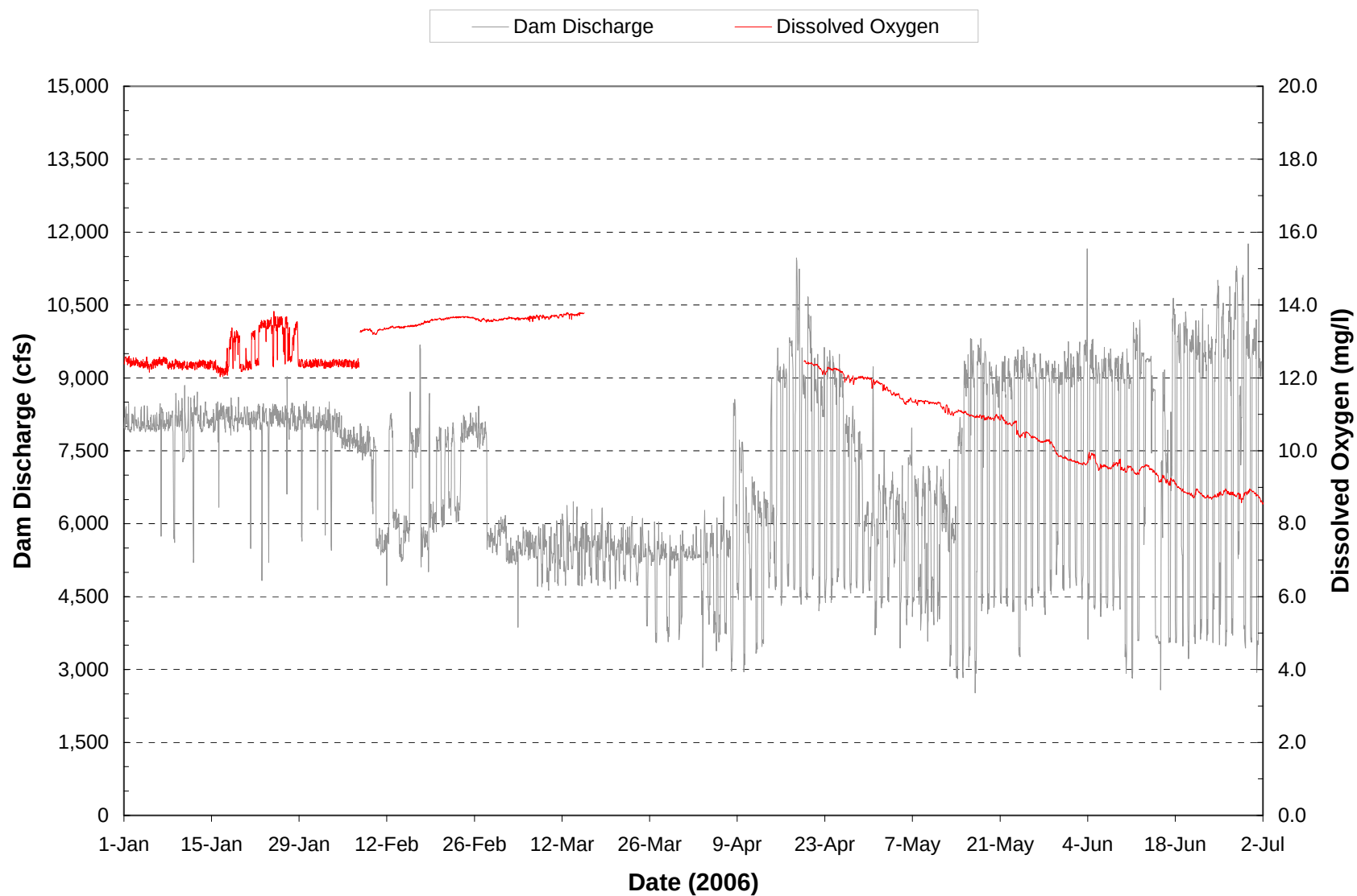
Plate 47. Hourly discharge and dissolved oxygen monitored at the Fort Peck powerplant on water discharged through the dam during the period January through June 2006. (Note: Gaps in dissolved oxygen plot represent periods when monitoring equipment was not operational.)
