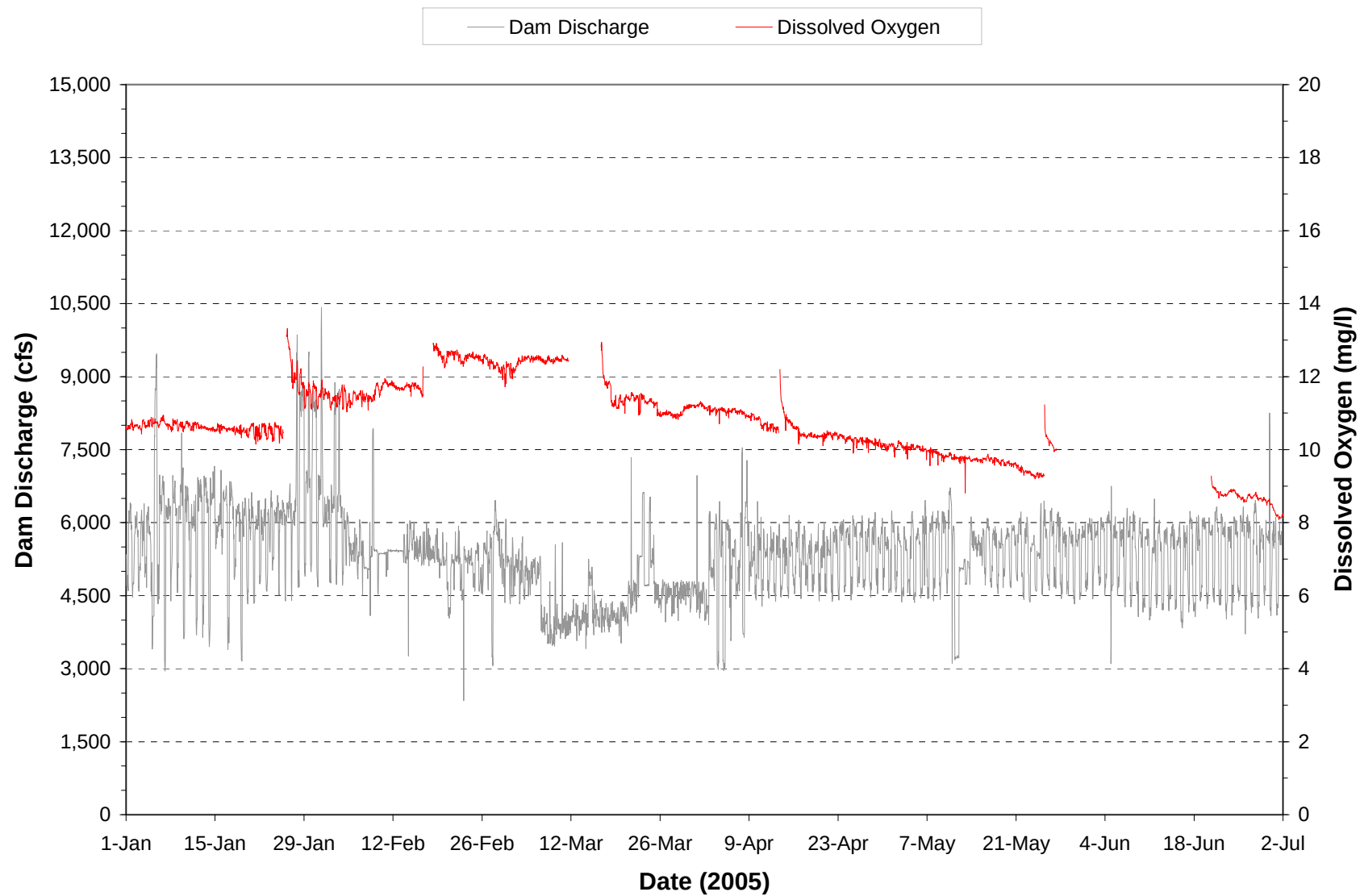
Plate 45. Hourly discharge and dissolved oxygen monitored at the Fort Peck powerplant on water discharged through the dam during the period January through June 2005. (Note: Gaps in dissolved oxygen plot represent periods when monitoring equipment was not operational.)
