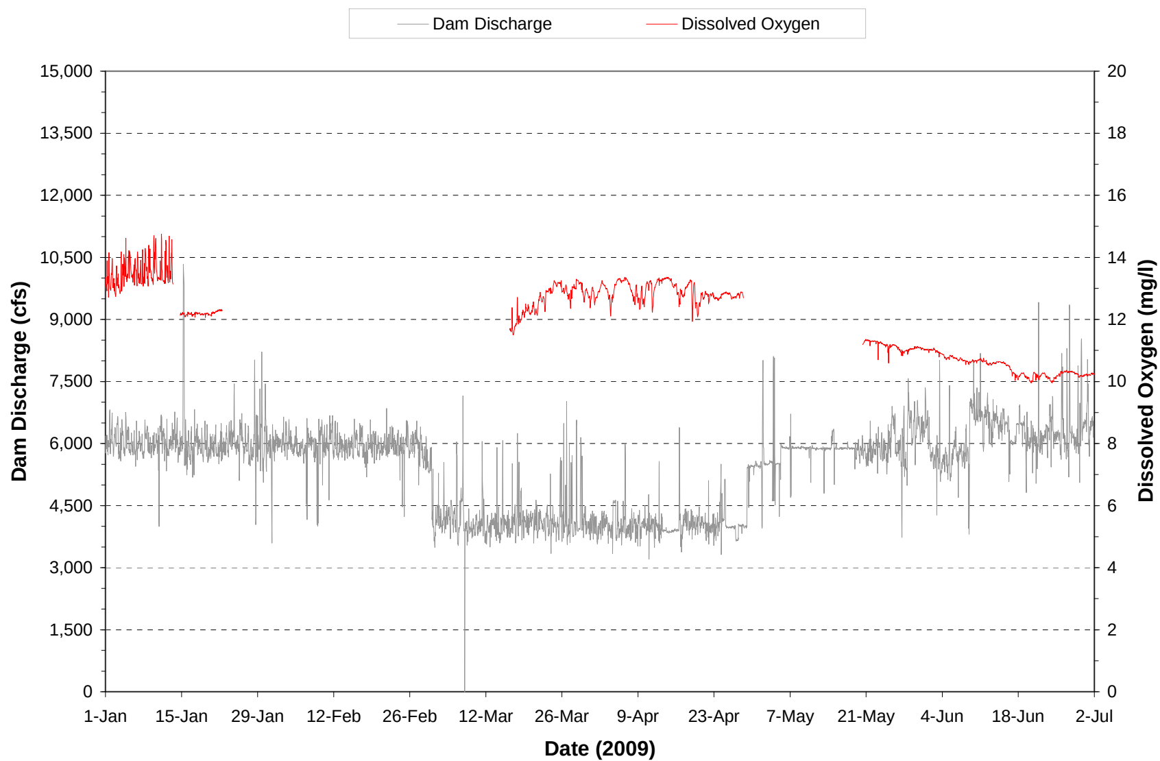
Plate 53. Hourly discharge and dissolved oxygen monitored at the Fort Peck powerplant on water discharged through the dam during the period January through June 2009.
