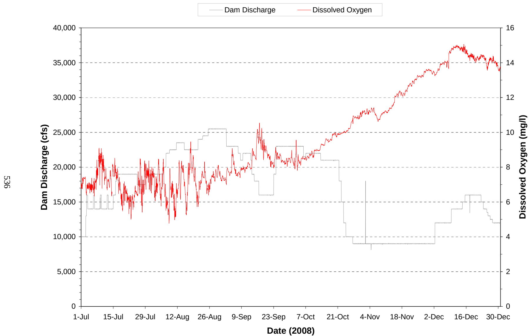
Plate 394. Hourly discharge and dissolved oxygen monitored at the Gavins Point powerplant on water discharged through the dam during the period July through December 2008.
