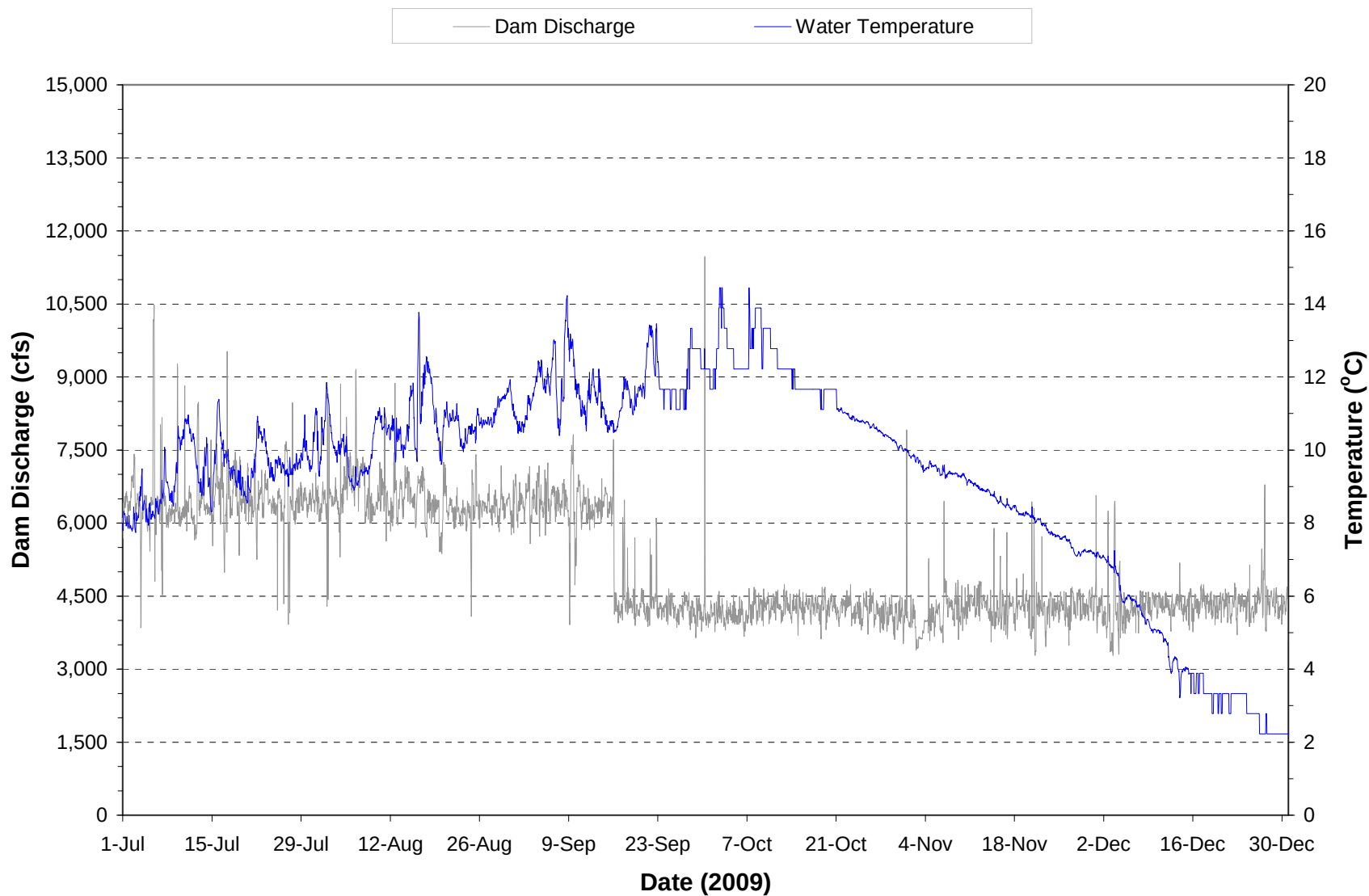
Plate 44. Hourly discharge and water temperature monitored at the Fort Peck powerplant on water discharged through the dam during the period July through December 2009.
