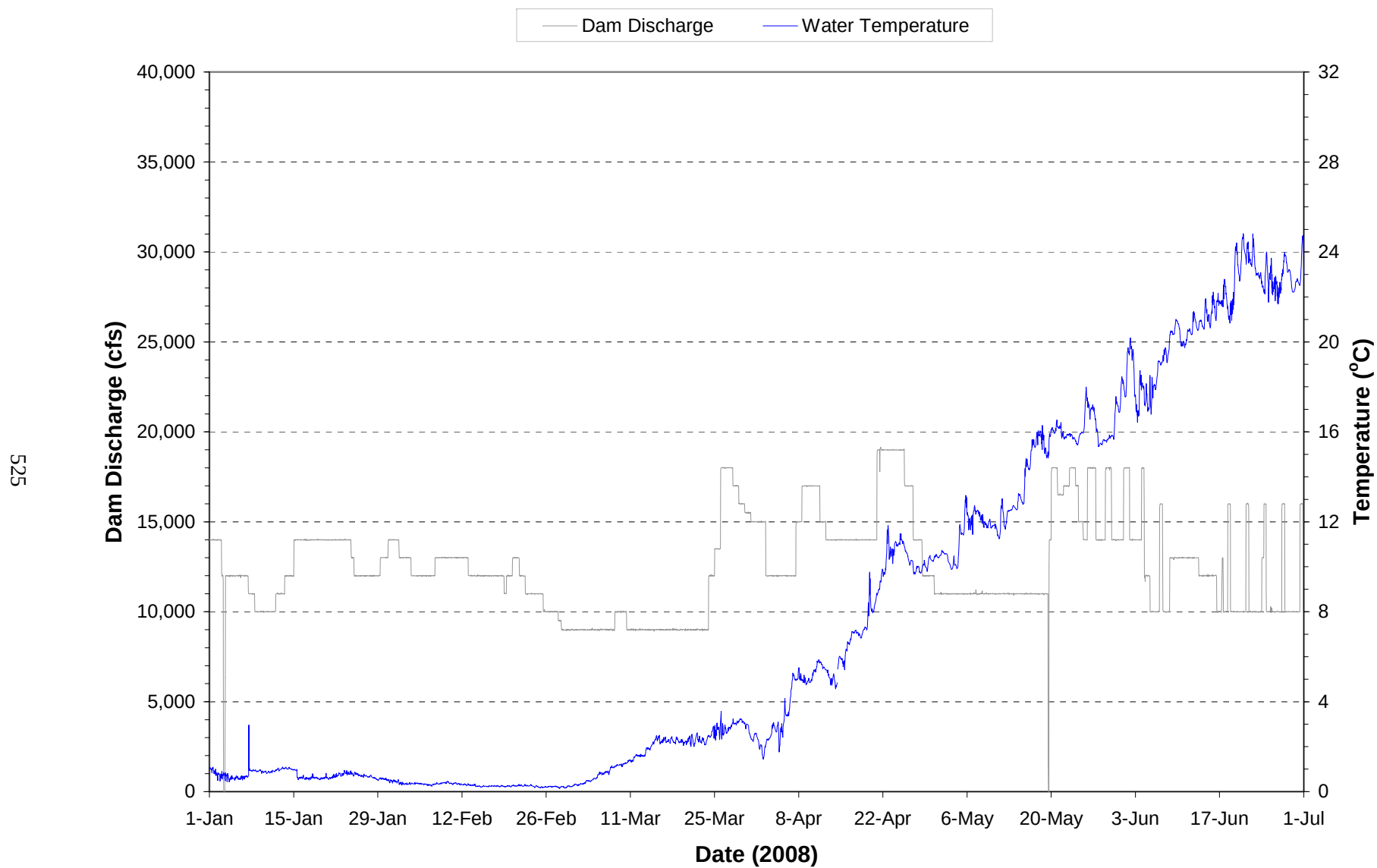
Plate 383. Hourly discharge and water temperature monitored at the Gavins Point powerplant on water discharged through the dam during the period January through June 2008.
