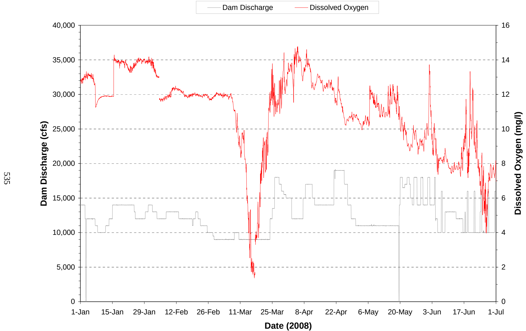
Plate 393. Hourly discharge and dissolved oxygen monitored at the Gavins Point powerplant on water discharged through the dam during the period January through June 2008.
