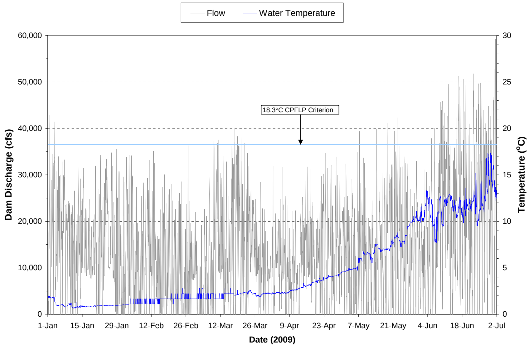
Plate 197. Hourly discharge and water temperature monitored at the Oahe powerplant on water discharged through the dam during the period January through June 2009.
