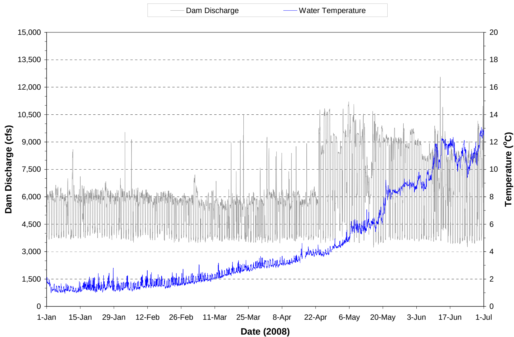
Plate 41. Hourly discharge and water temperature monitored at the Fort Peck powerplant on water discharged through the dam during the period January through June 2008.
