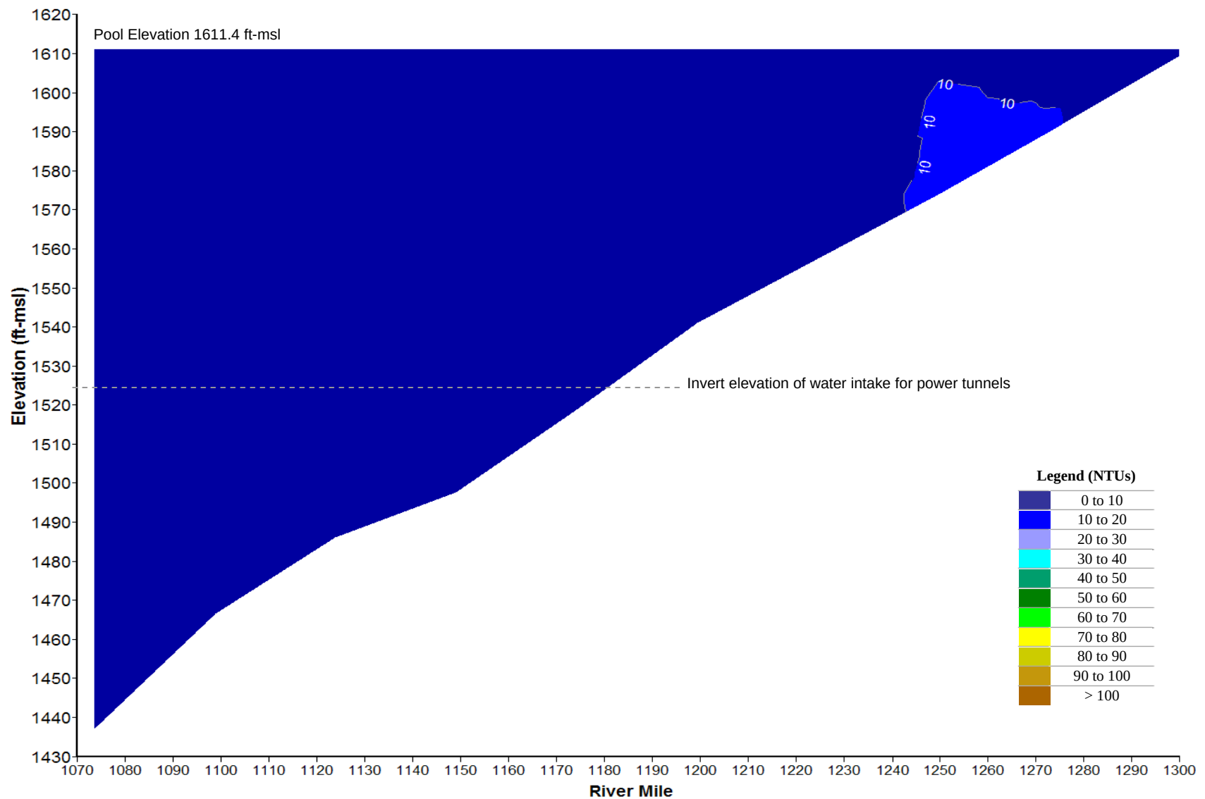
Plate 171. Longitudinal turbidity (NTU) contour plot of Lake Oahe based on depth-profile turbidity levels measured at sites OAHLK1073A, OAHLK1110DW, OAHLK1153DW, OAHLK1196DW, OAHLK1256DW, and OAHNFMORR1 on August 18, 2009.
