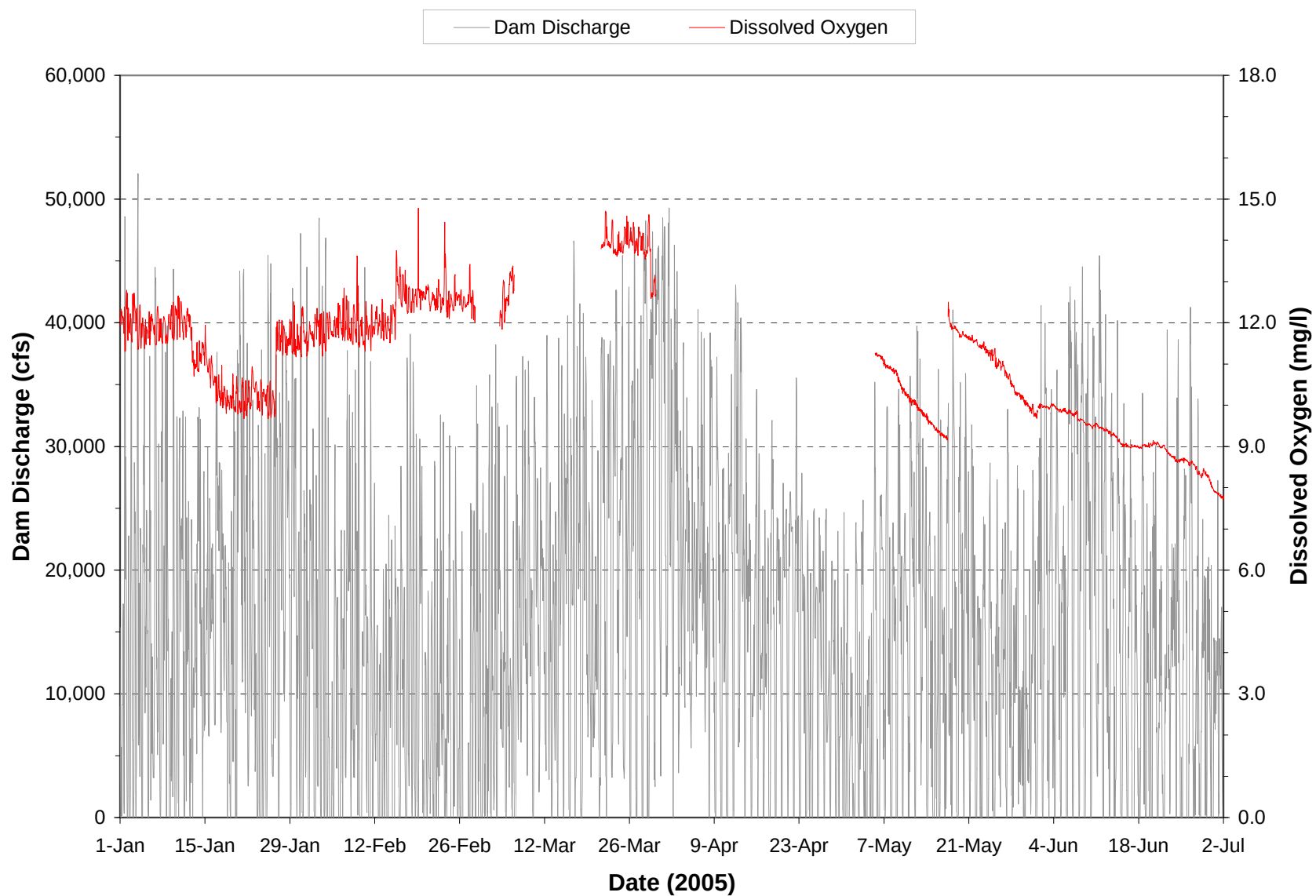
Plate 199. Hourly discharge and dissolved oxygen monitored at the Oahe powerplant on water discharged through the dam during the period January through June 2005. (Note: Gaps in dissolved oxygen plot represents periods when monitoring equipment was not operational.)
