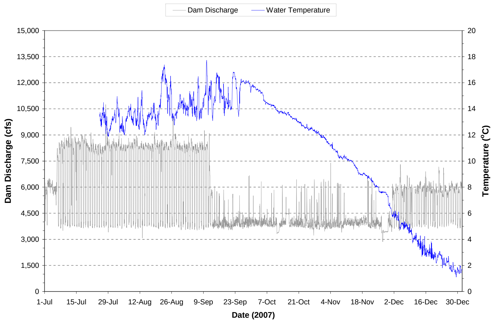
Plate 40. Hourly discharge and water temperature monitored at the Fort Peck powerplant on water discharged through the dam during the period July through December 2007. (Note: Gaps in temperature plot represents periods when monitoring equipment was not operational.)
