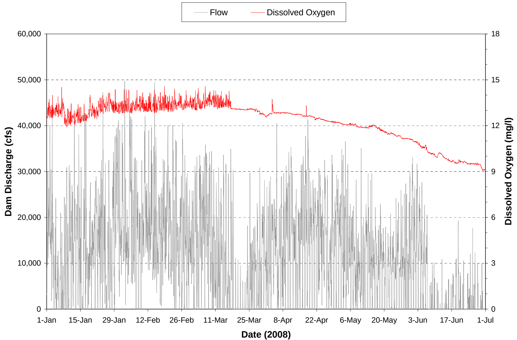
Plate 205. Hourly discharge and dissolved oxygen monitored at the Oahe powerplant on water discharged through the dam during the period January through June 2008.
