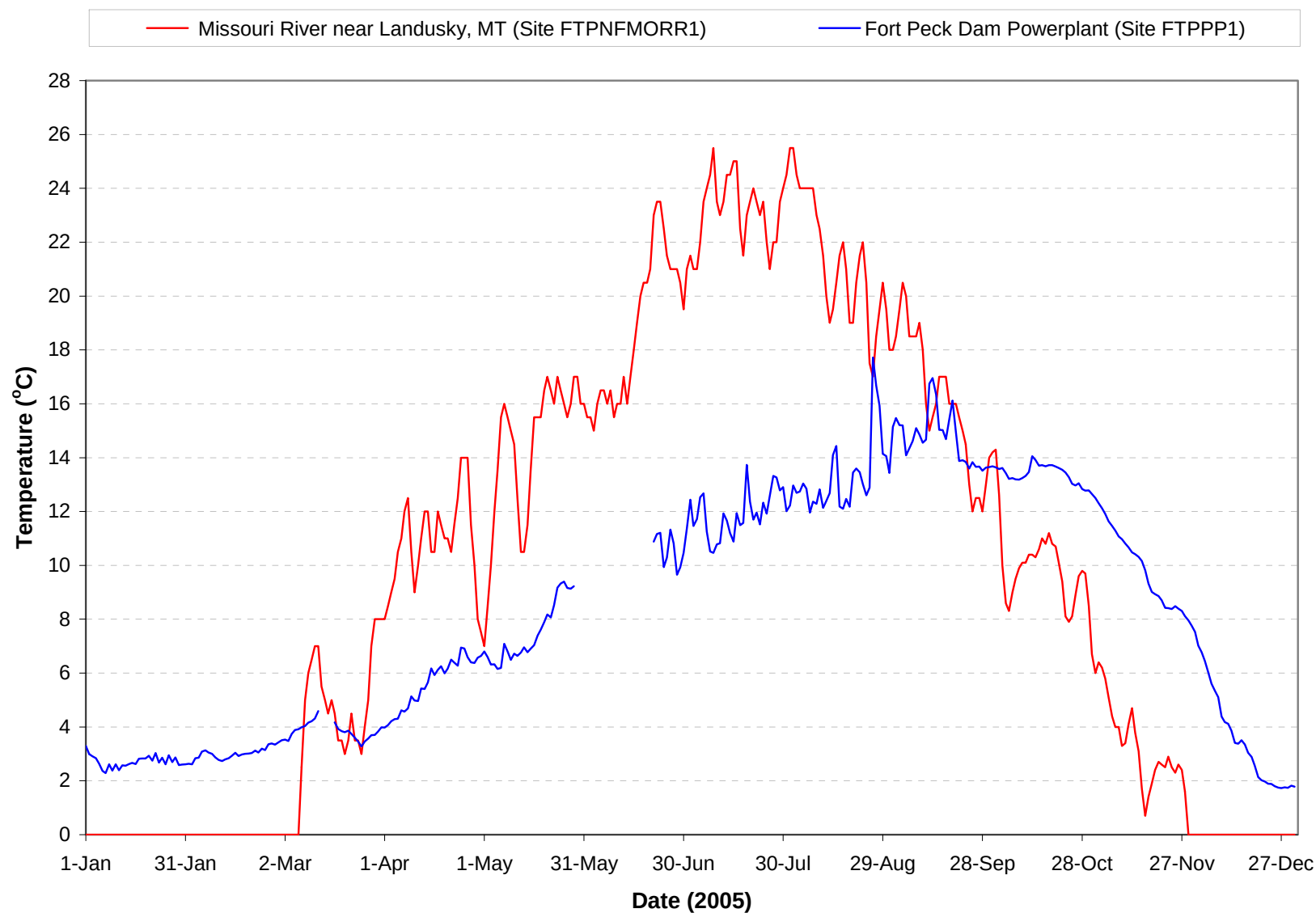
Plate 55. Mean daily water temperatures monitored at the Fort Peck Powerplant (i.e., site FTPPP1) and the Missouri River near Landusky, Montana (i.e., site FTPNFMORR1) during 2005. (Note: Gaps in temperature plots are periods when monitoring equipment was not operational.)
