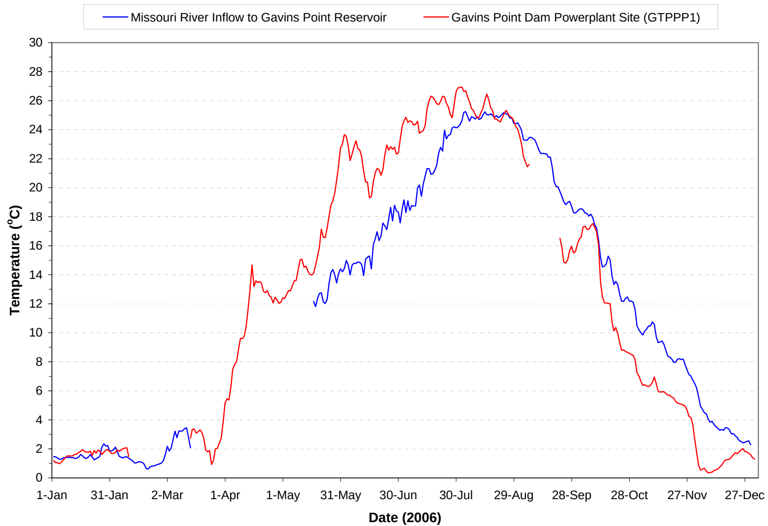
Plate 398. Mean daily water temperatures monitored at the Gavins Point Powerplant (i.e., site GTPPP1) and estimated for the Missouri River inflow to Lewis and Clark Lake during 2006.
