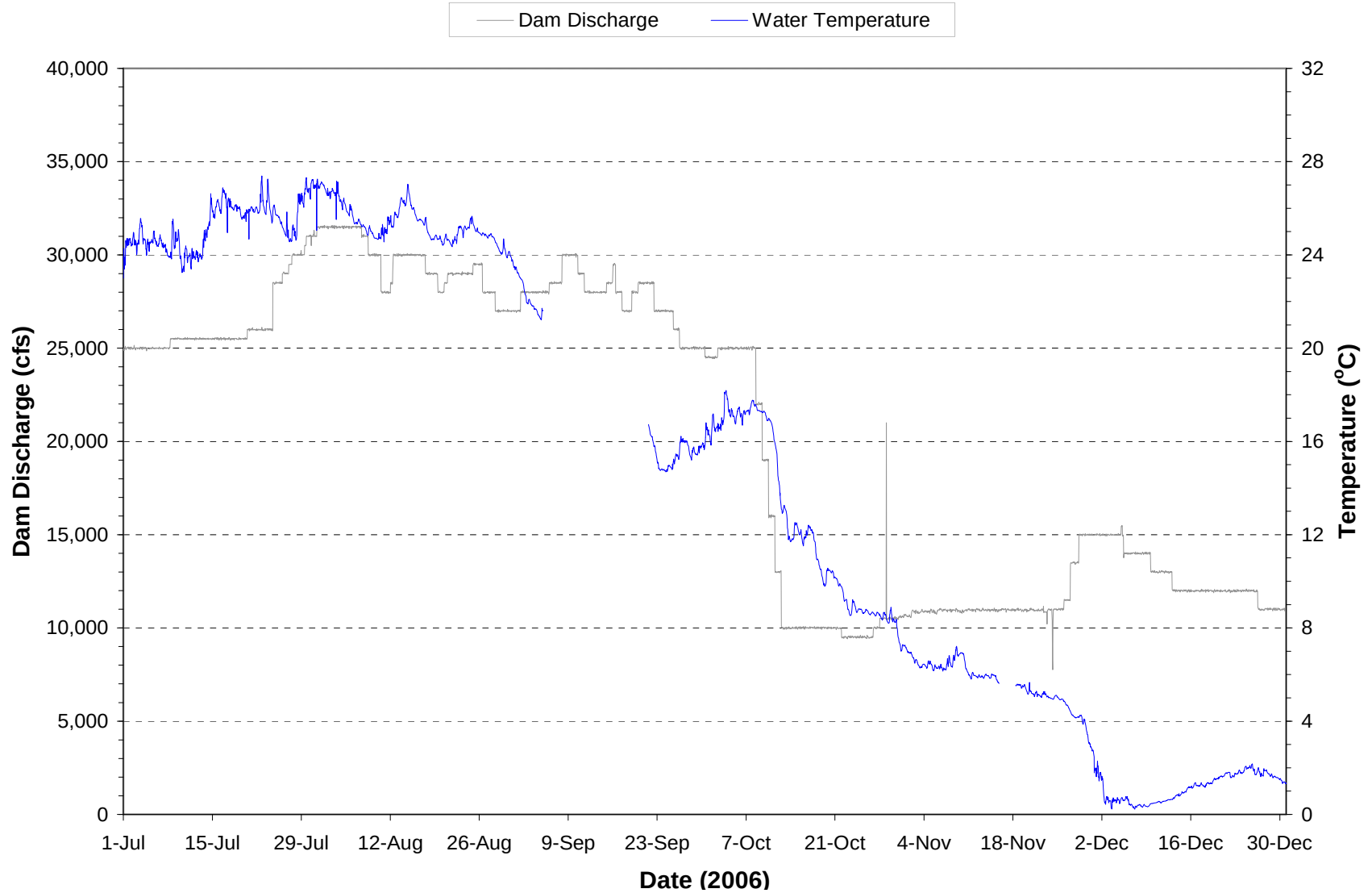
Plate 380. Hourly discharge and water temperature monitored at the Gavins Point powerplant on water discharged through the dam during the period July through December 2006.
