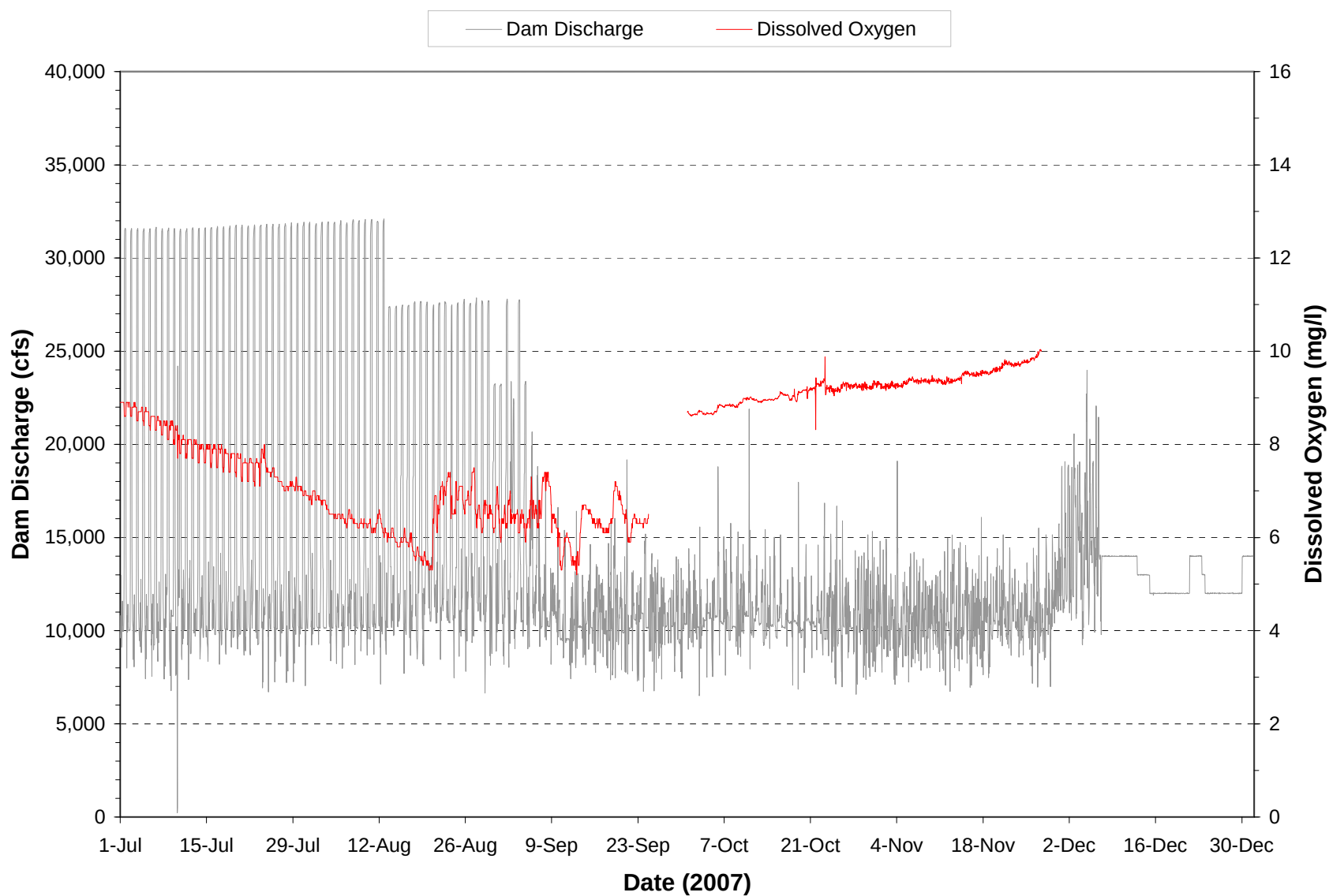
Plate 126. Hourly discharge and dissolved oxygen monitored at the Garrison powerplant on water discharged through the dam during the period July through December 2007. (Note: Gaps in dissolved oxygen plot represents periods when monitoring equipment was not operational.)
