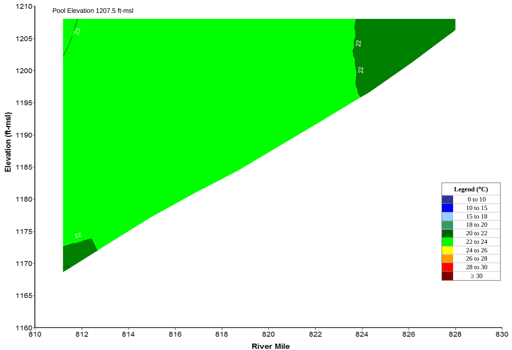
Plate 340. Longitudinal water temperature (°C) contour plot of Lewis and Clark Lake based on depth-profile water temperatures measured at sites GPTLK0811A, GPTLK0815DW, GPTLK0819DW, GPTLK0822DW, and GPTLK0825DW on July 16, 2009.
