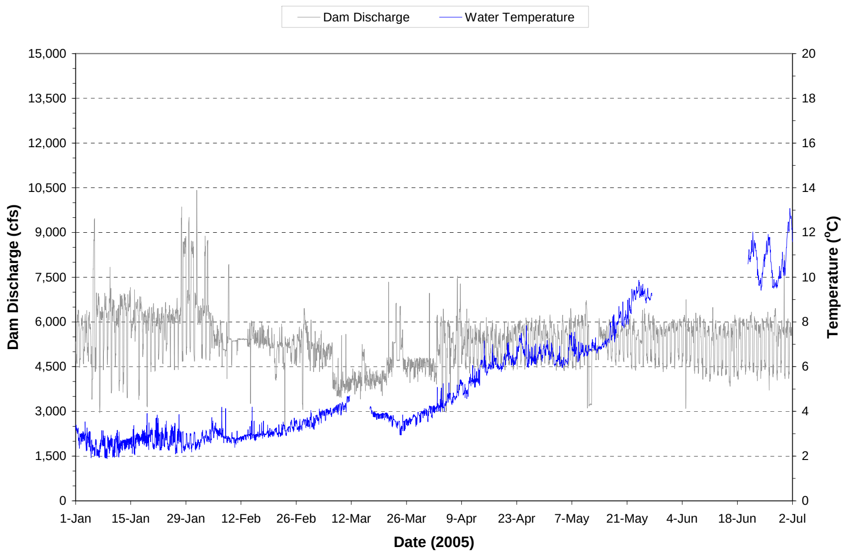
Plate 35. Hourly discharge and water temperature monitored at the Fort Peck powerplant on water discharged through the dam during the period January through June 2005. (Note: Gaps in temperature plot represents periods when monitoring equipment was not operational.)
