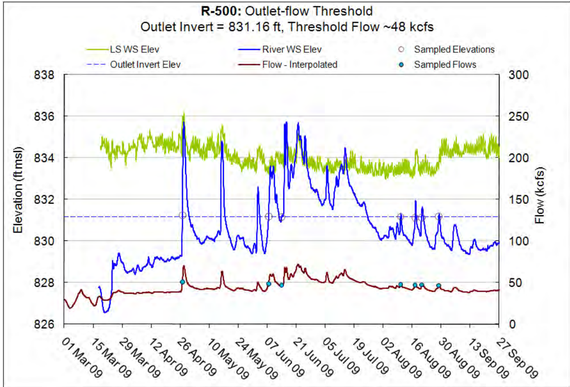
Figure 10.25.8 – Outlet-flow threshold, R-500
