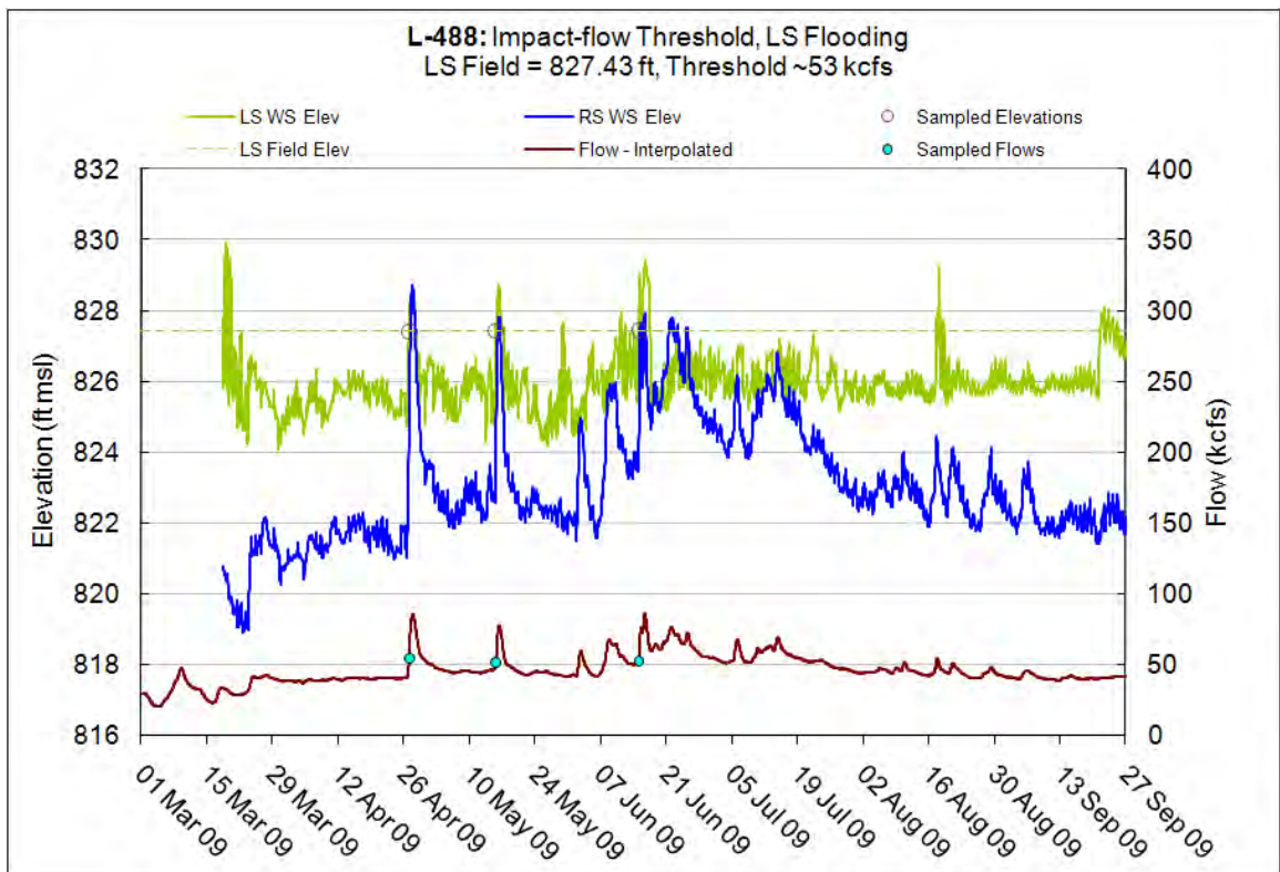
Figure 10.27.9 – Impact-flow threshold (overbank flooding), L-488
