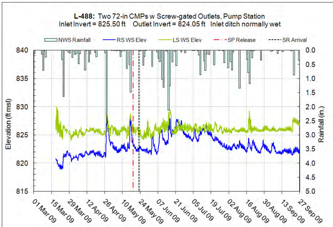
Figure 10.27.5 – Full monitoring record at L-488
