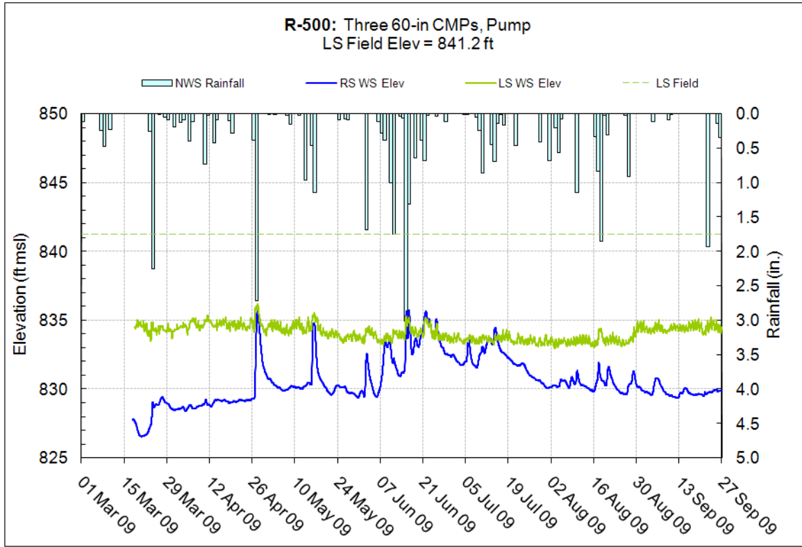
Figure 10.25.7 – Surveyed field elevations, R-500
