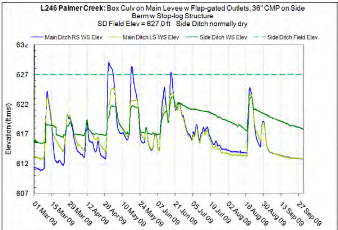
Figure 10.39.10 – Surveyed field elevations of side ditch, L-246 Palmer Creek
