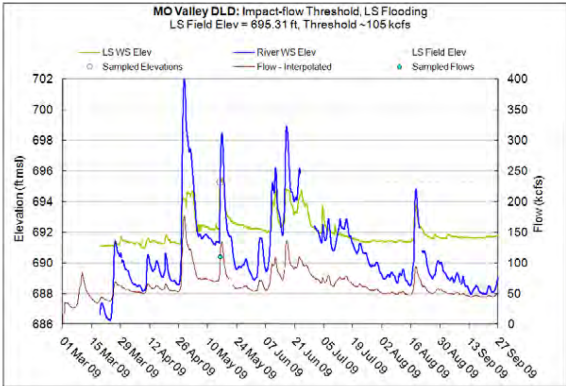
Figure 10.33.10 – Impact-flow threshold (LS overland flooding), MO Valley DLD
