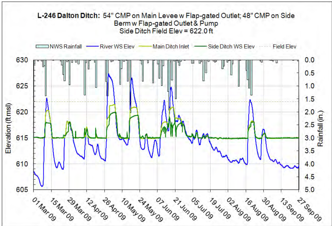
Figure 10.40.12 – Side ditch surveyed field elevations, L-246 Dalton Ditch
