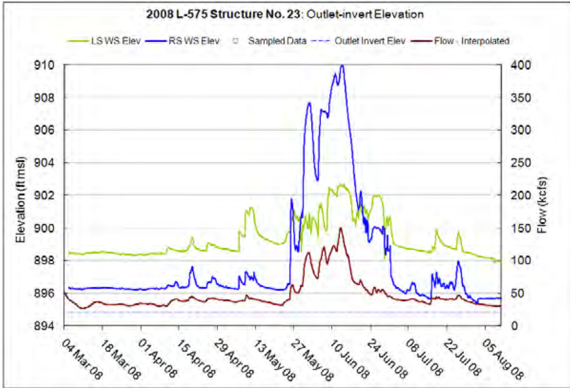
Figure 10.20.15 – Outlet-invert elevation, L-575 Structure No. 23 (2008 record)
