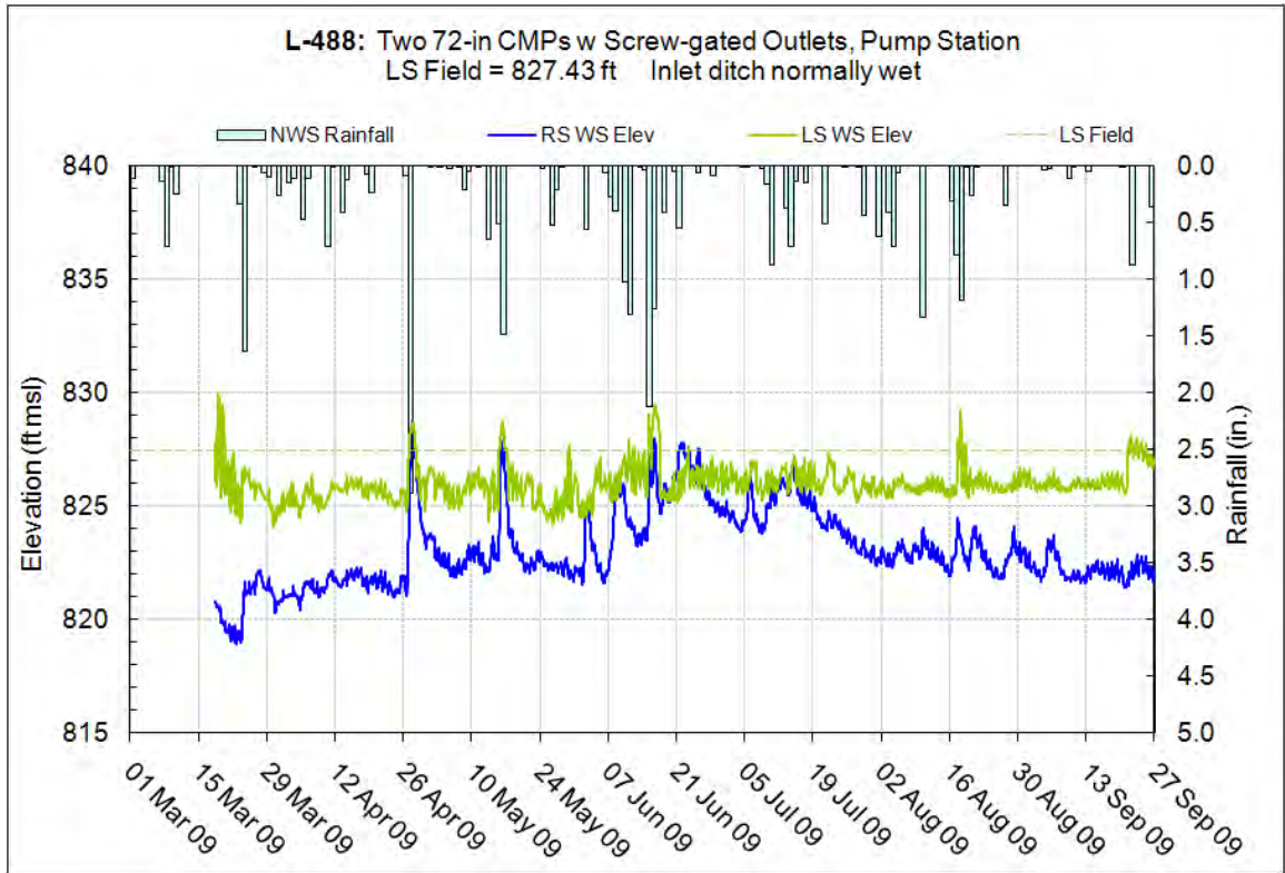
Figure 10.27.7 – Surveyed field elevations, L-488
