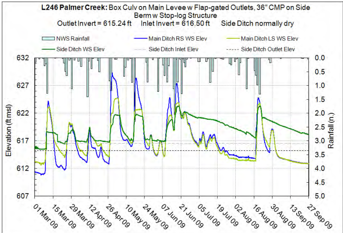
Figure 10.39.9 – Invert elevations of side ditch, L-246 Palmer Creek
