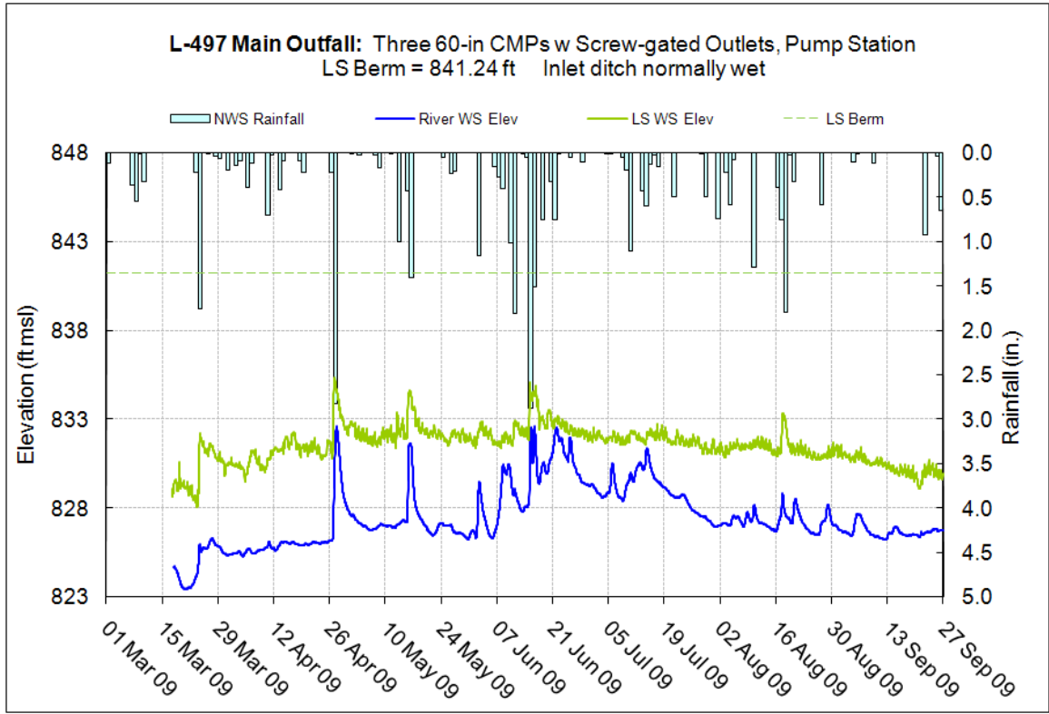
Figure 10.26.7 – Surveyed field elevations, L-497 Main Outfall
