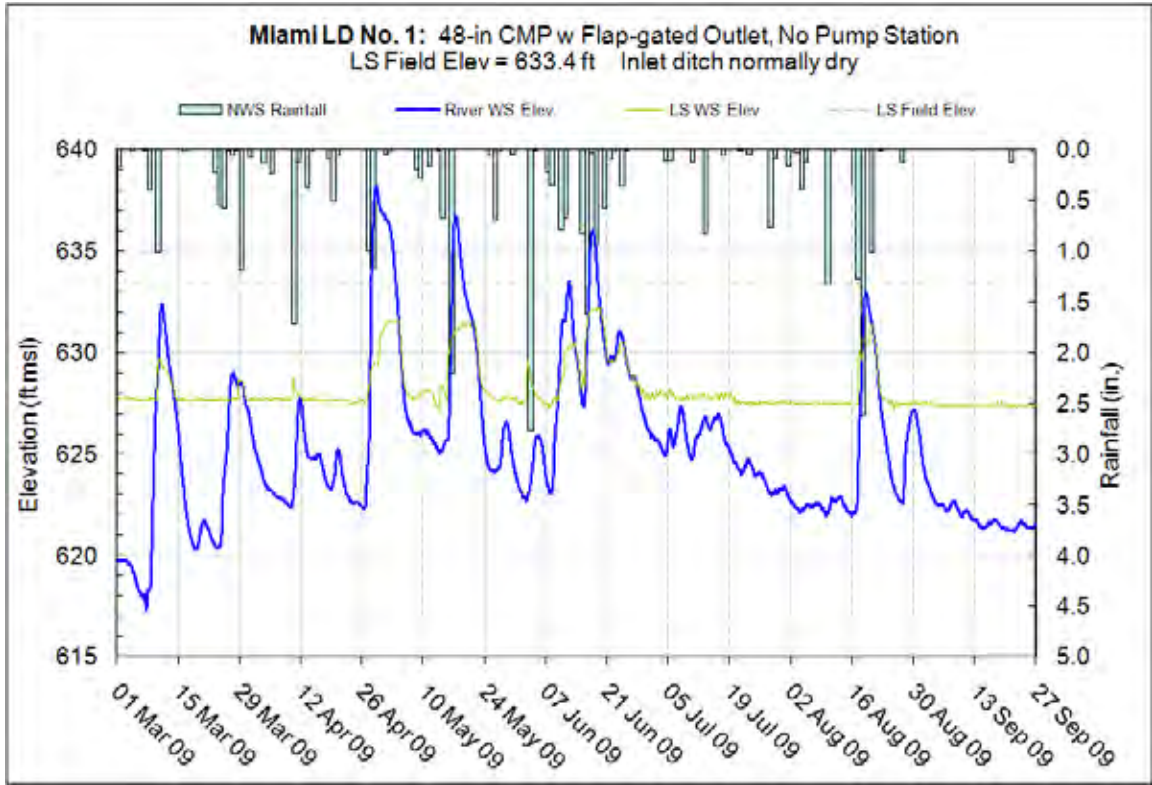
Figure 10.37.6 – Surveyed field elevations, Miami LD No. 1
