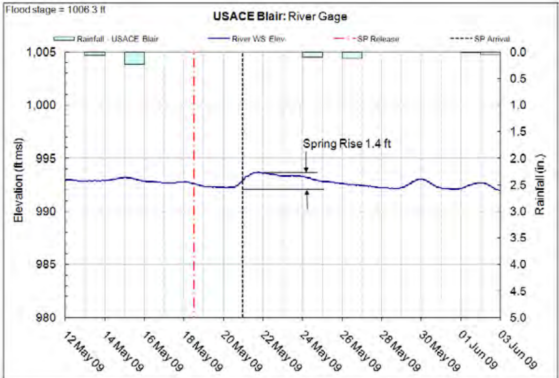
Figure 10.13.2 – Spring rise at USACE Blair
