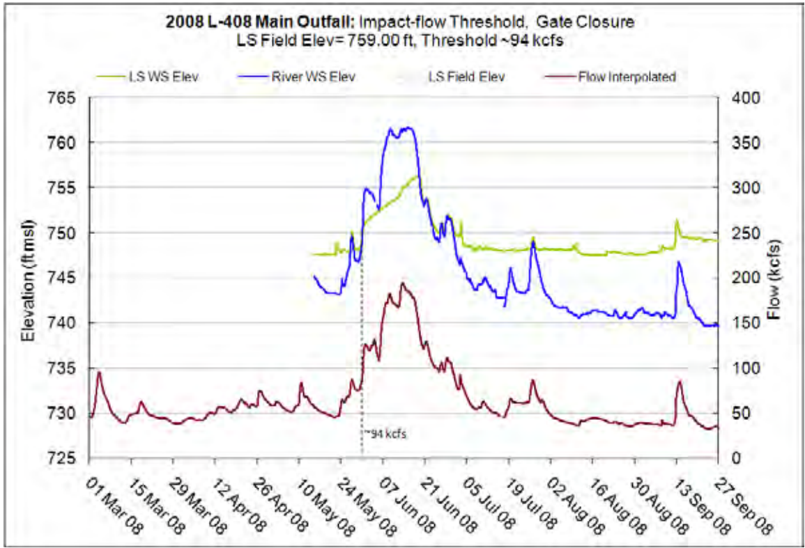
Figure 10.30.10 – Impact-flow threshold (gate closure), L-408 (2008 record)
