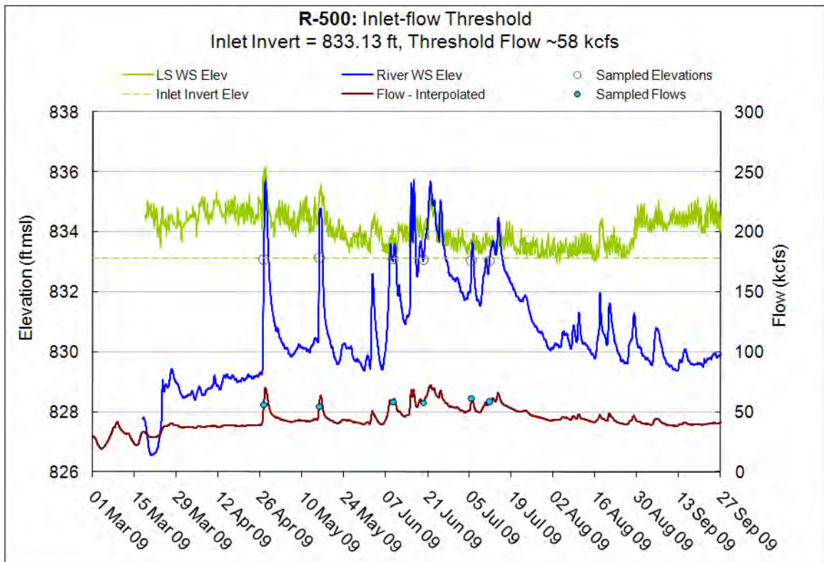
Figure 10.25.9 – Inlet-flow threshold, R-500
