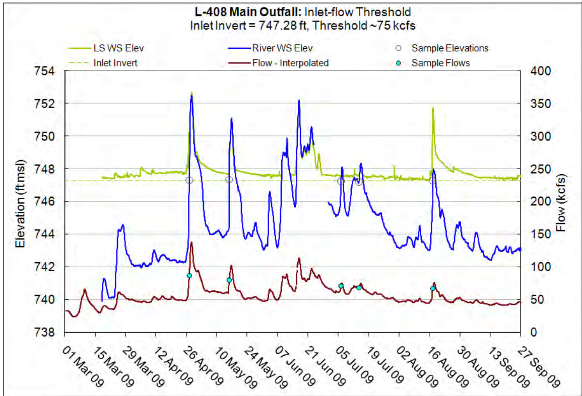
Figure 10.30.9 – Inlet-flow threshold, L-408
