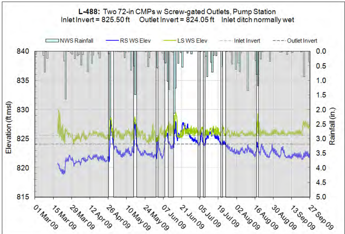
Figure 10.27.6 – Invert elevations, L-488
