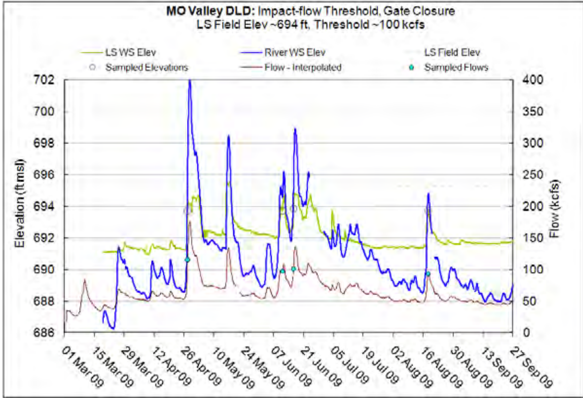
Figure 10.33.11 – Impact-flow threshold (gate closure), MO Valley DLD. The threshold varies in this case because the owner has some control of the gate.
