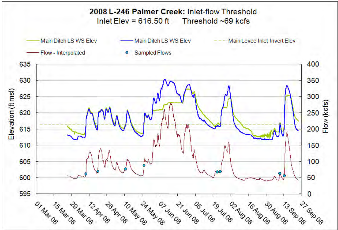
Figure 10.39.18 – Main ditch inlet-flow threshold, L-246 Palmer Creek (2008 record)
