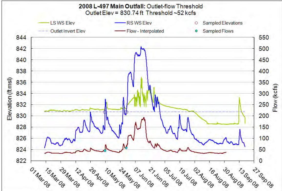
Figure 10.26.11 – Outlet-flow threshold, L-497 Main Outfall
