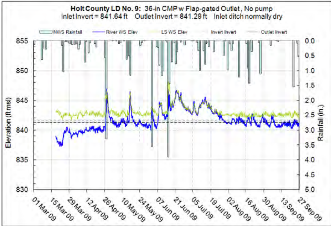
Figure 10.24.5 – Invert elevations, Holt County LD No. 9
