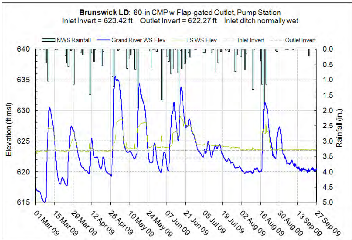
Figure 10.38.6 – Invert elevations, Brunswick LD
