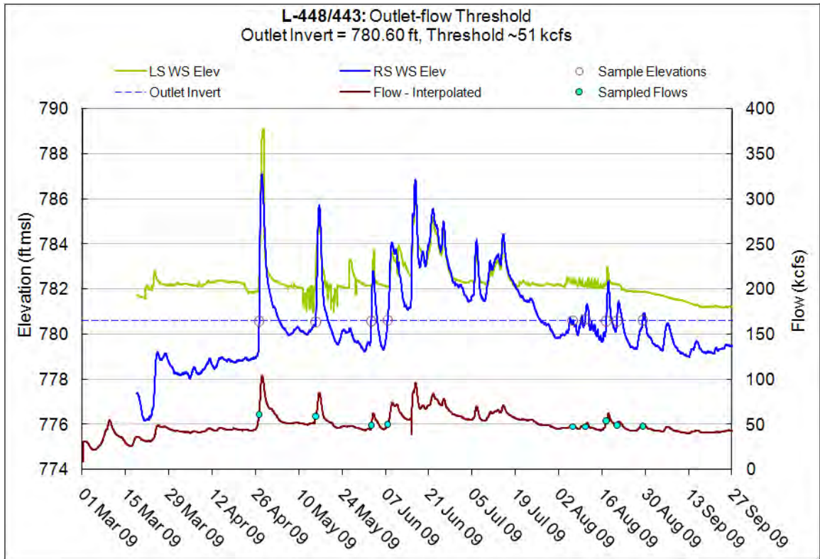
Figure 10.29.8 – Outlet-flow threshold, L-448/443
