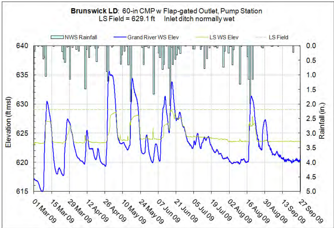
Figure 10.38.7 – Surveyed field elevations, Brunswick LD
