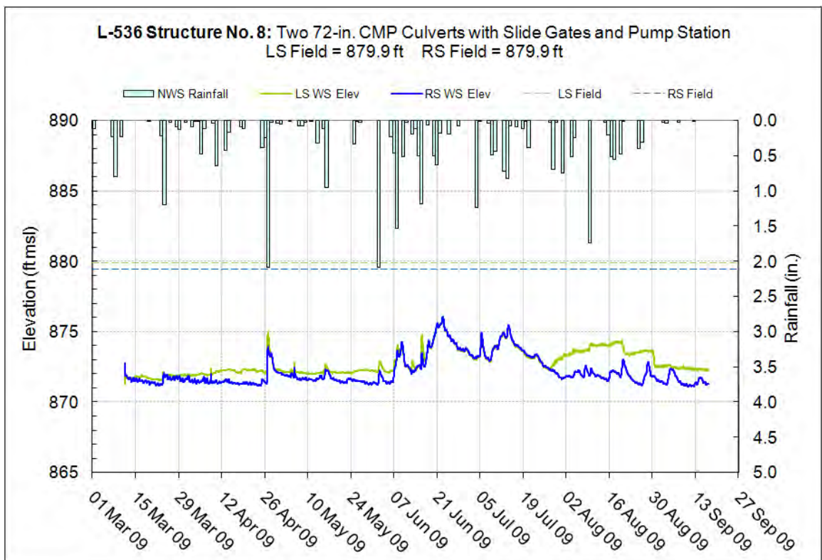
Figure 10.22.6 – Surveyed field elevations, L-536 Structure No. 8
