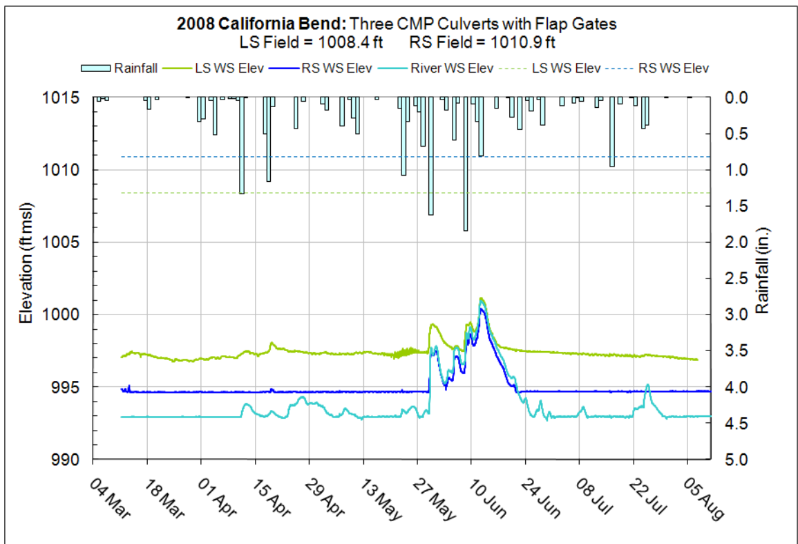
Figure 10.12.6 – Surveyed field elevations at California Bend, 2008 record
