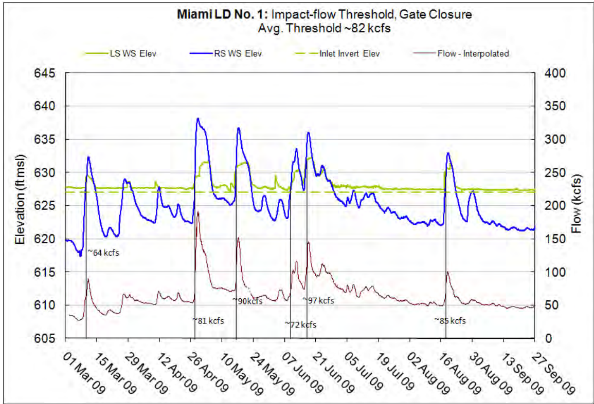
Figure 10.37.8 – NSR impact-flow threshold (gate-closure), Miami LD No. 1
