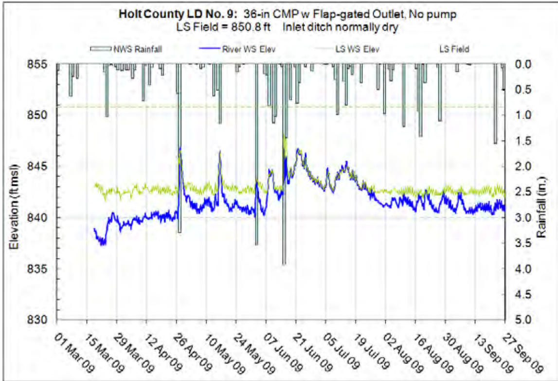
Figure 10.24.6 – Surveyed field elevations, Holt County LD No. 9
