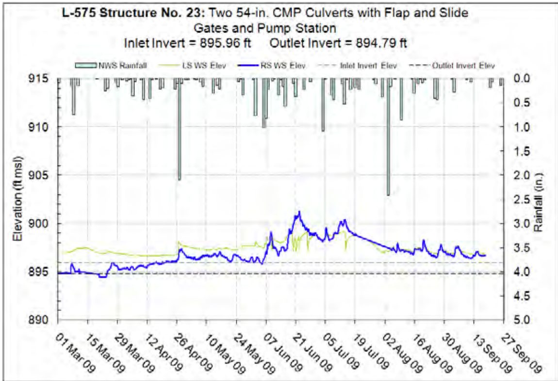
Figure 10.20.5 – Invert elevations, L-575 Structure No. 23
