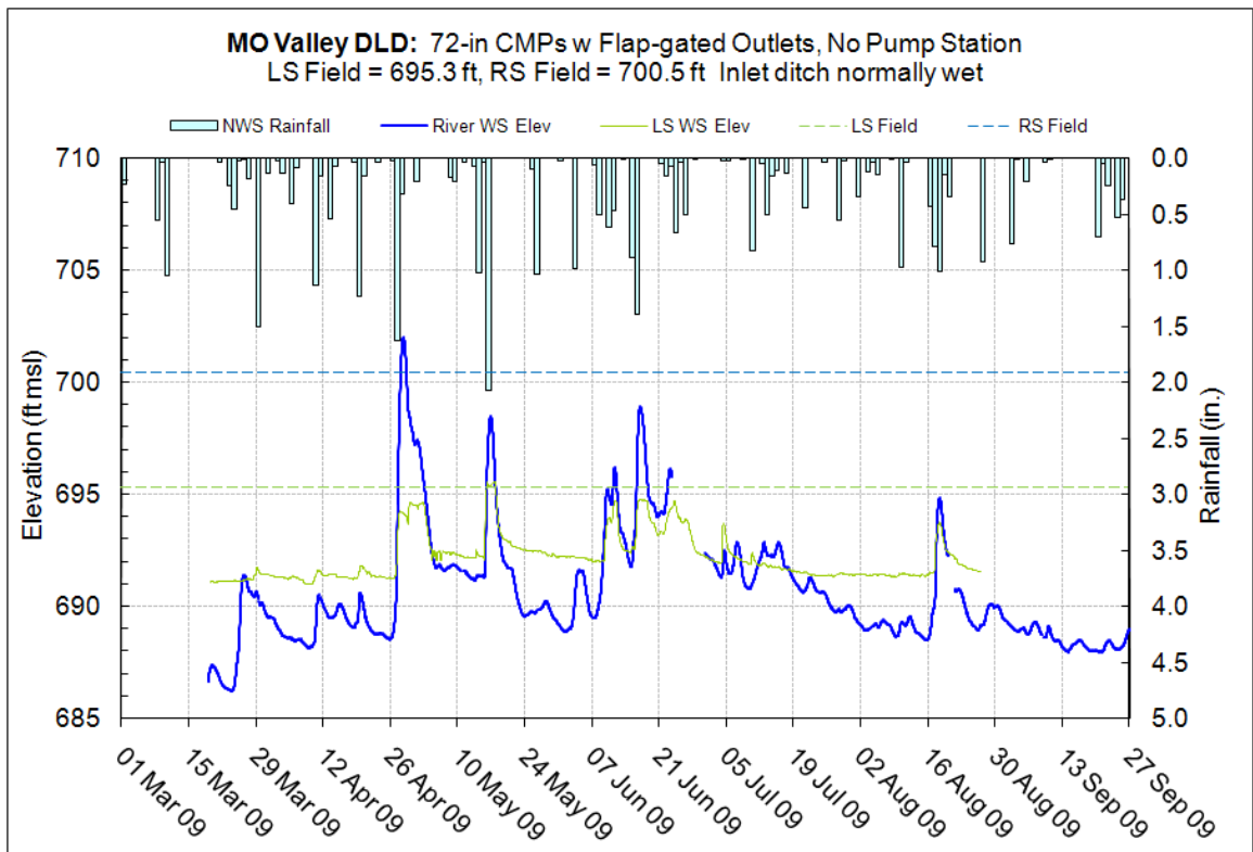
Figure 10.33.7 – Surveyed field elevations, MO Valley DLD
