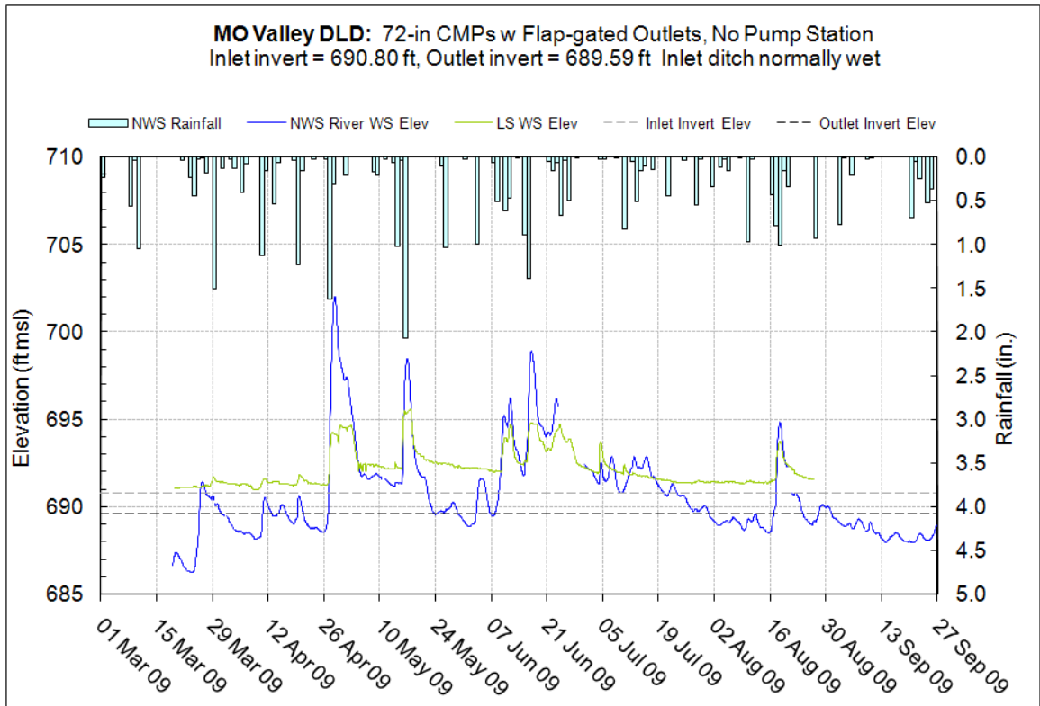
Figure 10.33.6 – Invert elevations, MO Valley DLD
