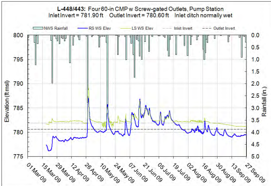
Figure 10.29.6 – Invert elevations, L-448/443
