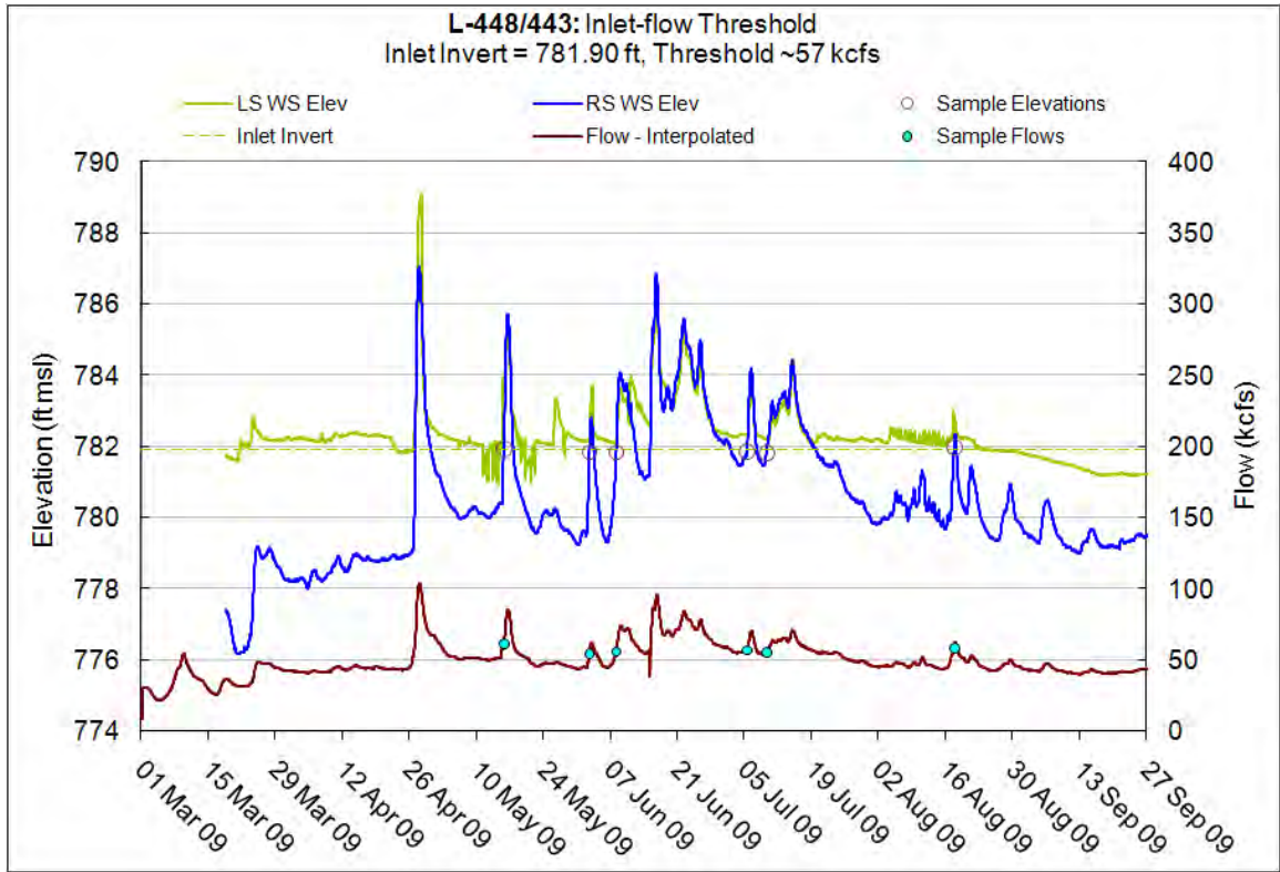
Figure 10.29.9 – Inlet-flow threshold, L-448/443
