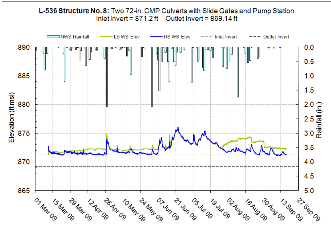
Figure 10.22.5 – Invert elevations, L-536 Structure No. 8
