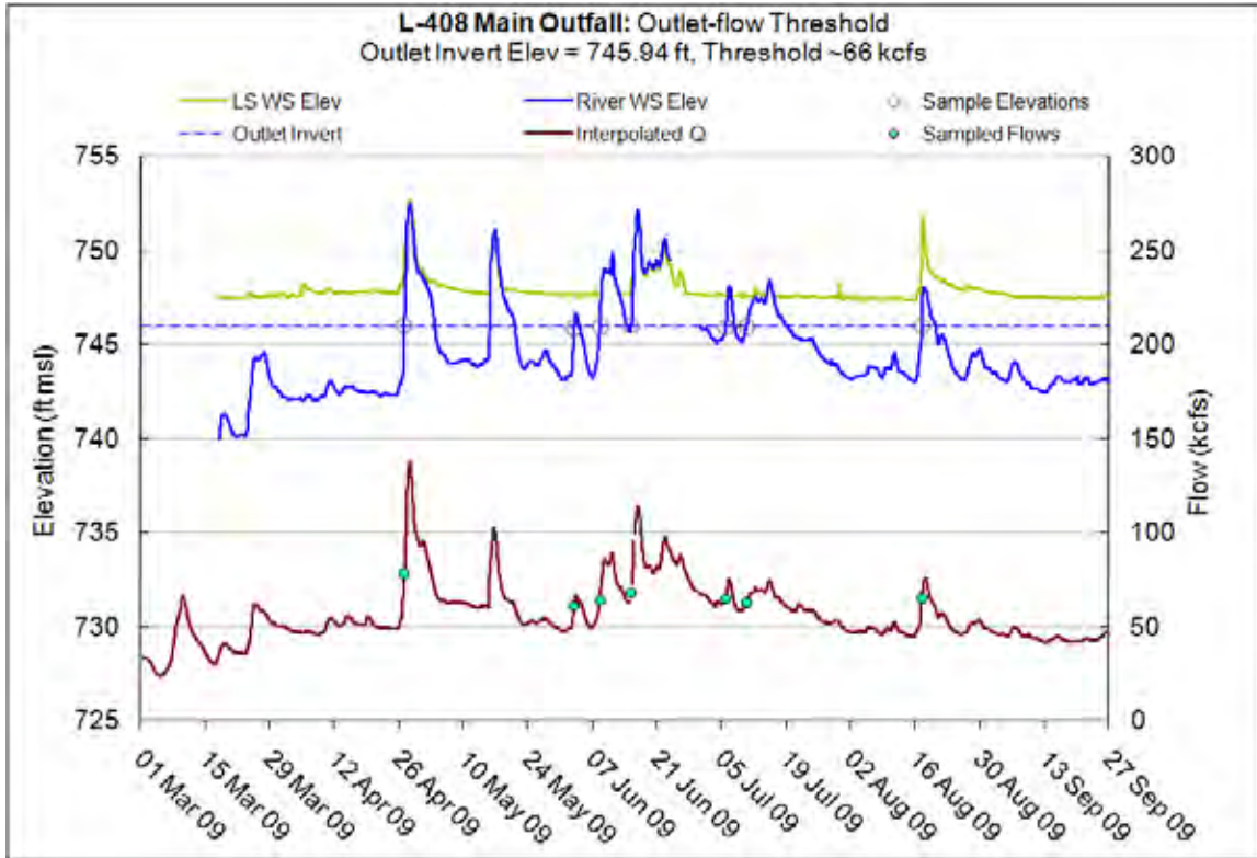
Figure 10.30.8 – Outlet-flow threshold, L-408
