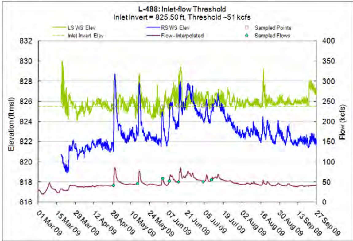
Figure 10.27.11 – Inlet-flow threshold, L-488
