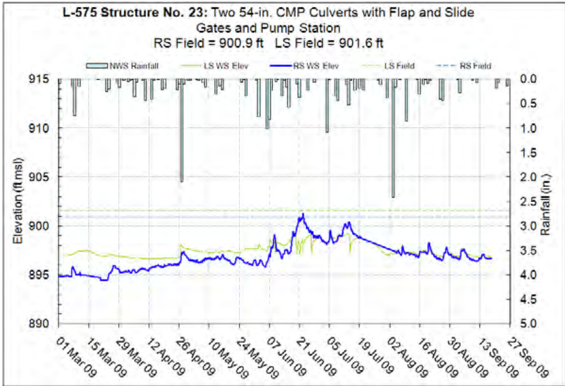
Figure 10.20.6 – Surveyed field elevations, L-575 Structure No. 23
