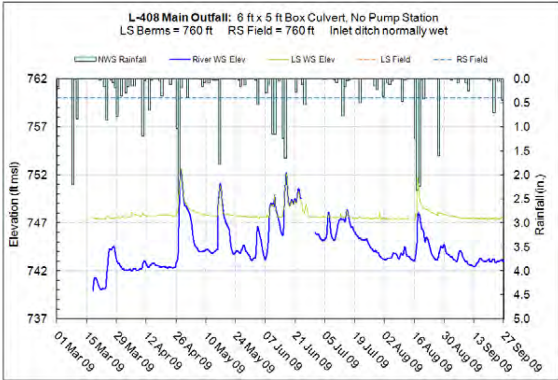
Figure 10.30.7 – Surveyed field elevations, L-408
