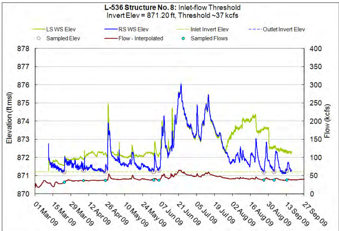
Figure 10.22.8 – Inlet-flow threshold, L-536 Structure No. 8 (2008 record)
