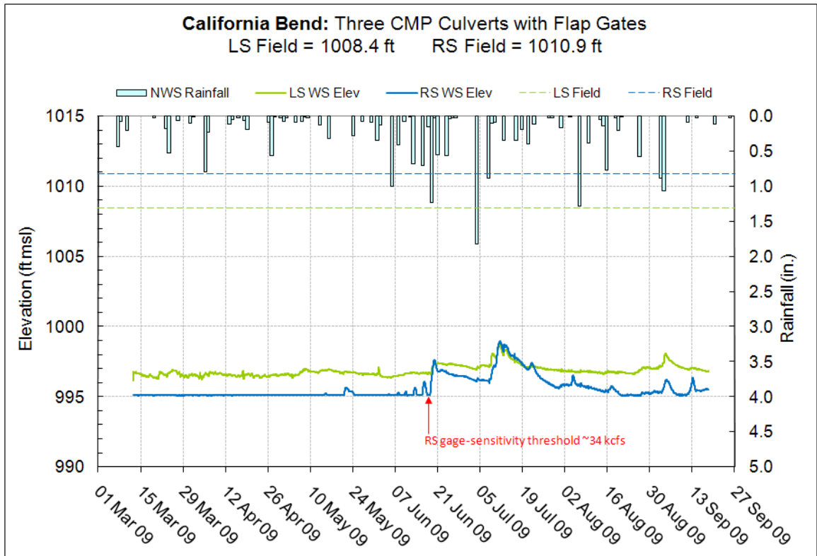
Figure 10.12.5 – Surveyed field elevations at California Bend
