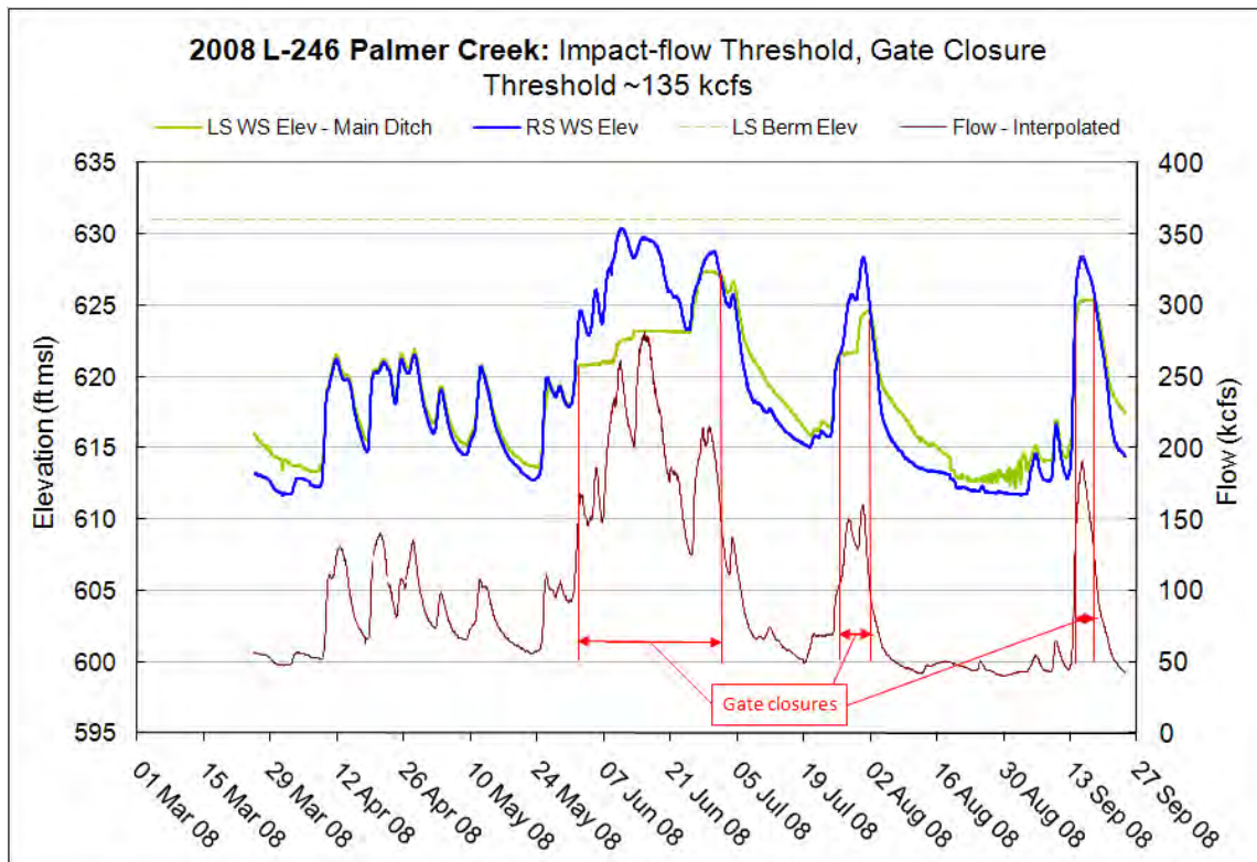
Figure 10.39.16 – Main ditch impact-flow threshold (gate closure), L-246 Palmer Creek (2008 record)
