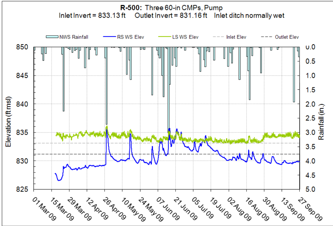
Figure 10.25.6 – Inlet elevations, R-500
