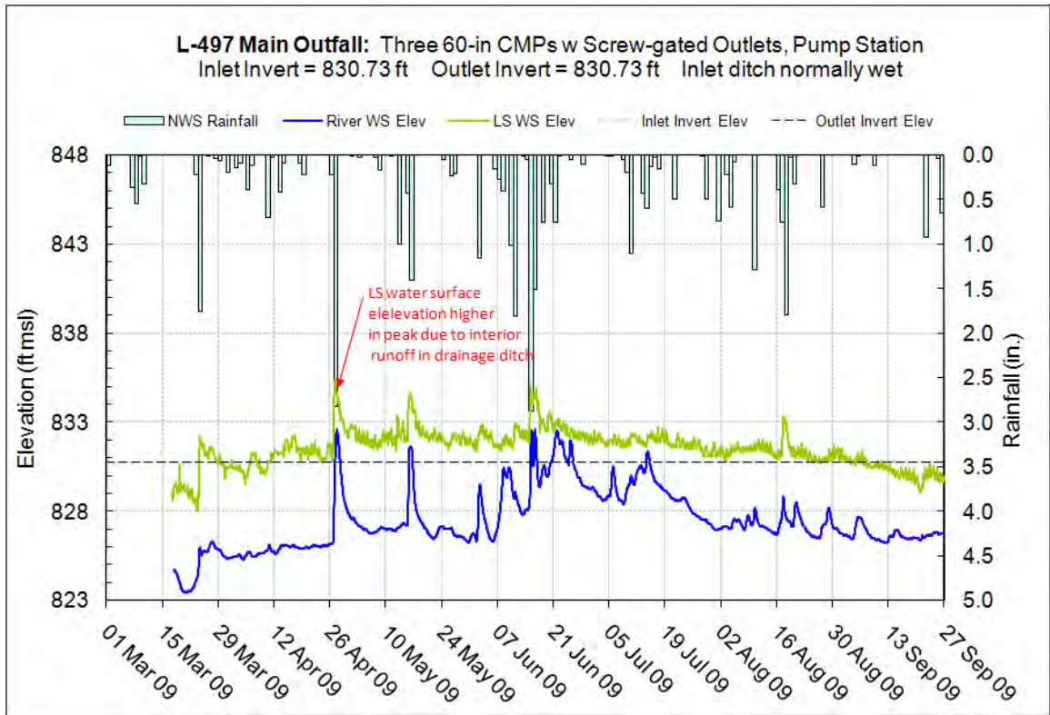
Figure 10.26.6 – Invert elevations, L-497 Main Outfall
