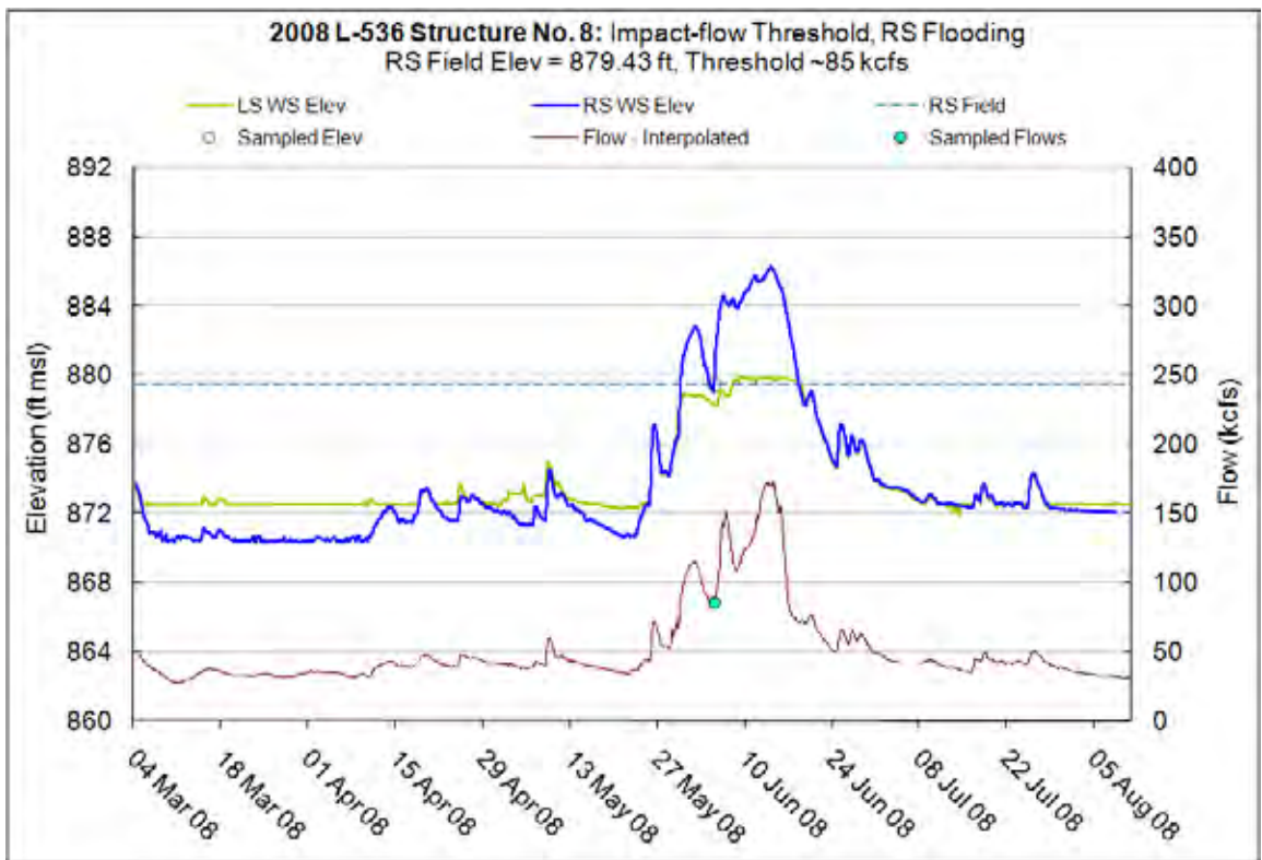
Figure 10.22.10 – Impact-flow threshold (RS flooding), L-536 Structure No. 8 (2008 record)
