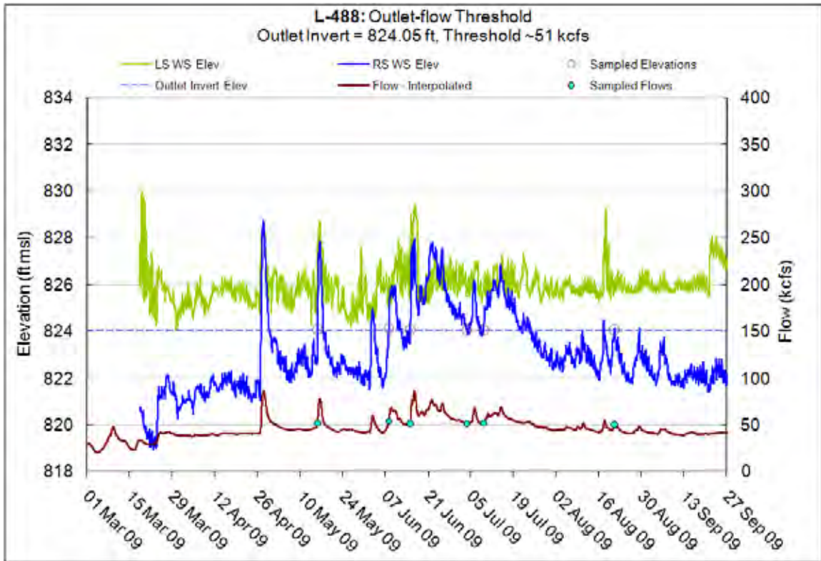
Figure 10.27.10 – Outlet-flow threshold, L-488
