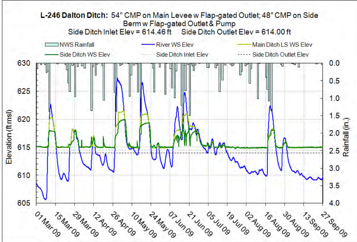
Figure 10.40.11 – Side ditch invert elevations of L-246 Dalton Ditch
