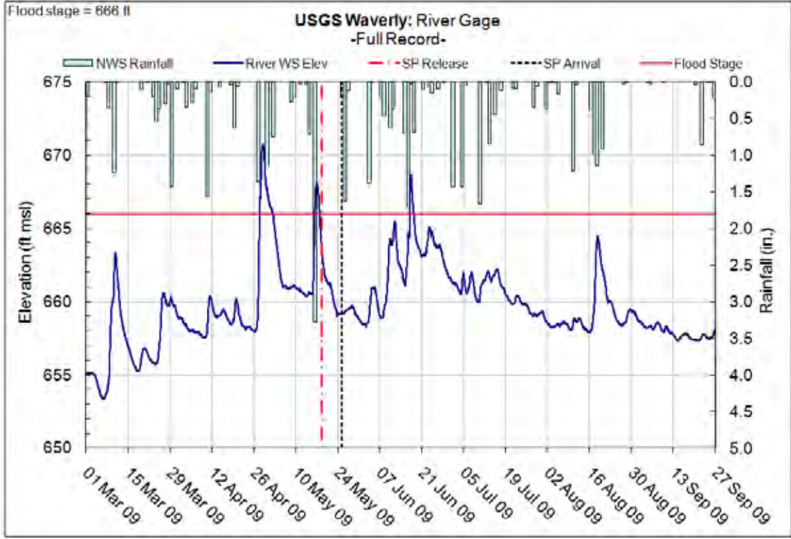
Figure 10.34.3 – Full monitoring record at USGS Waverly
