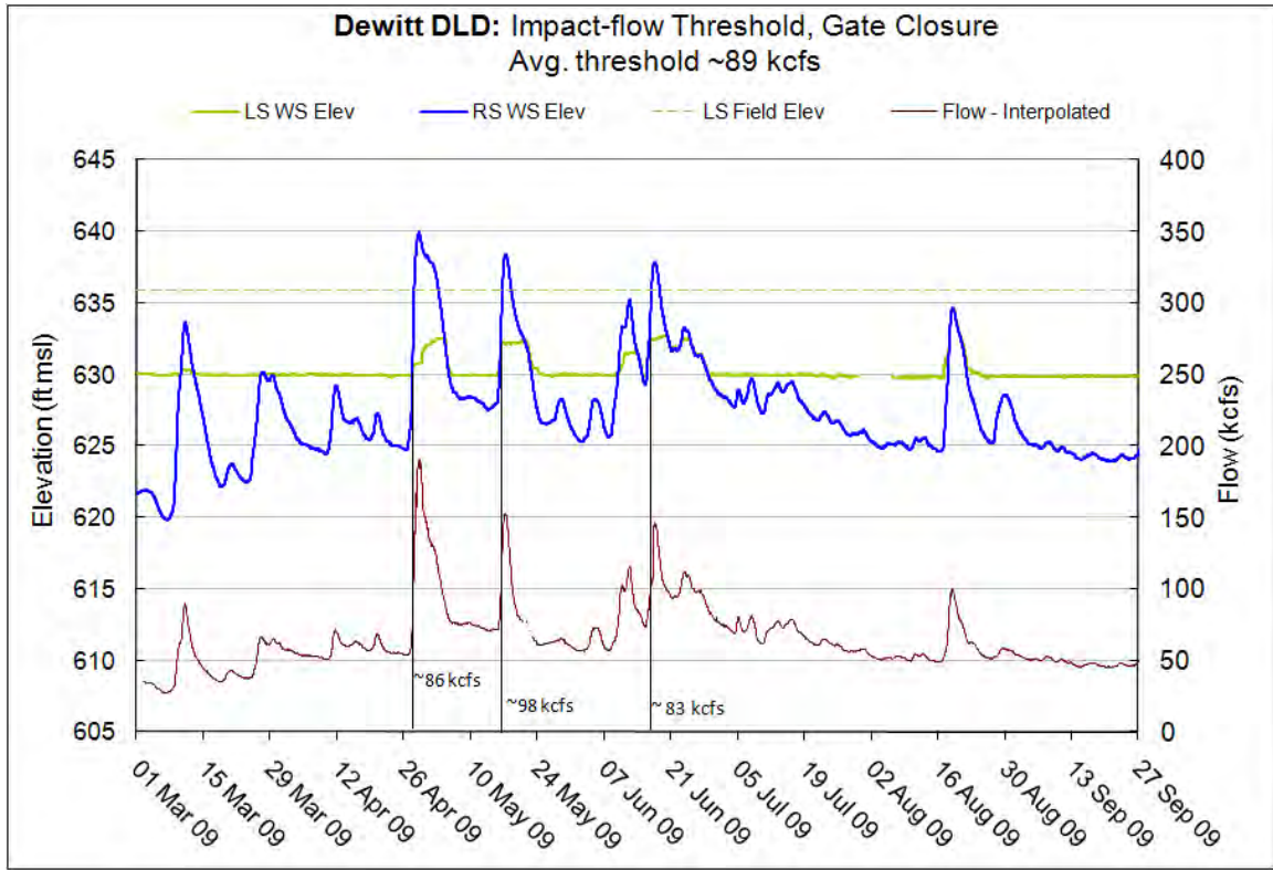
Figure 10.36.8 – Impact-flow threshold (gate closure), Dewitt DLD
