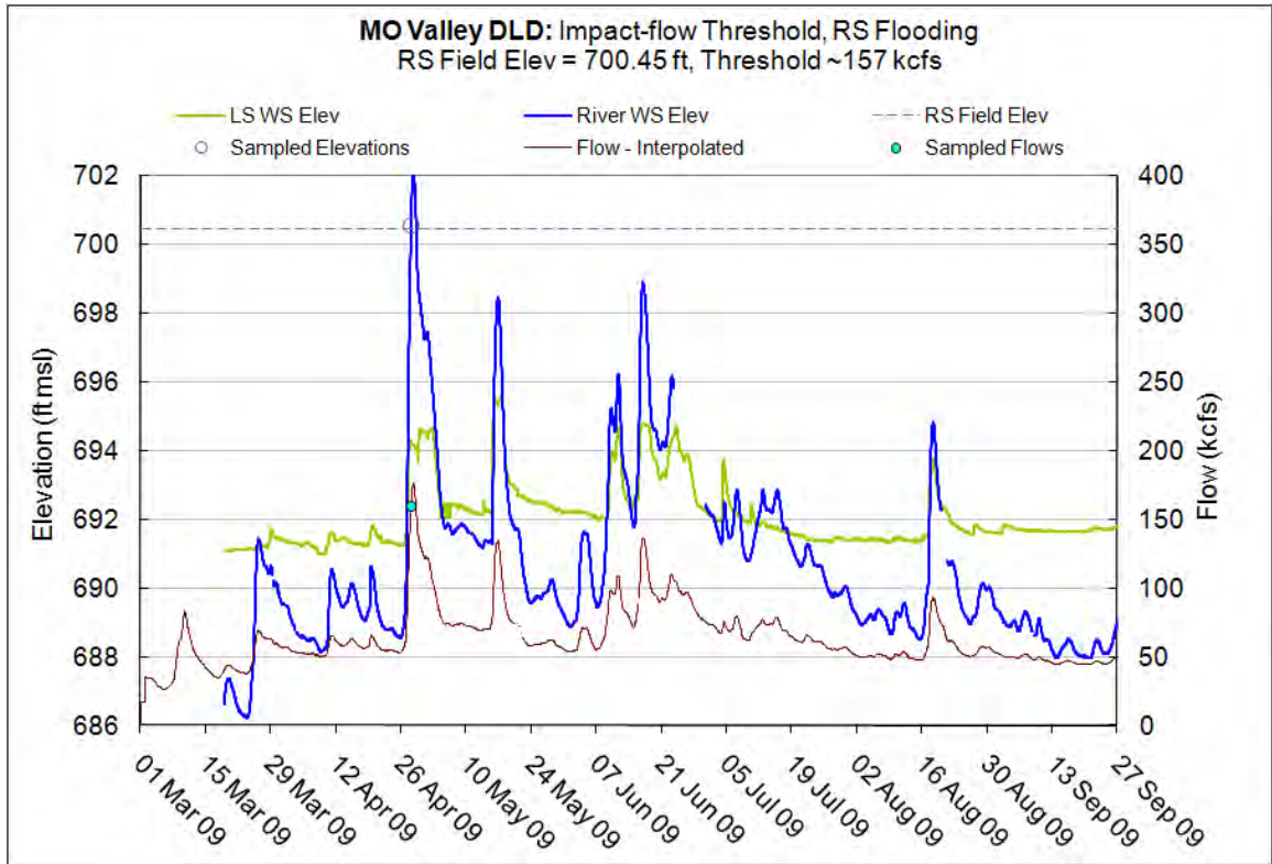
Figure 10.33.9 – Impact-flow threshold (RS overland flooding), MO Valley DLD
