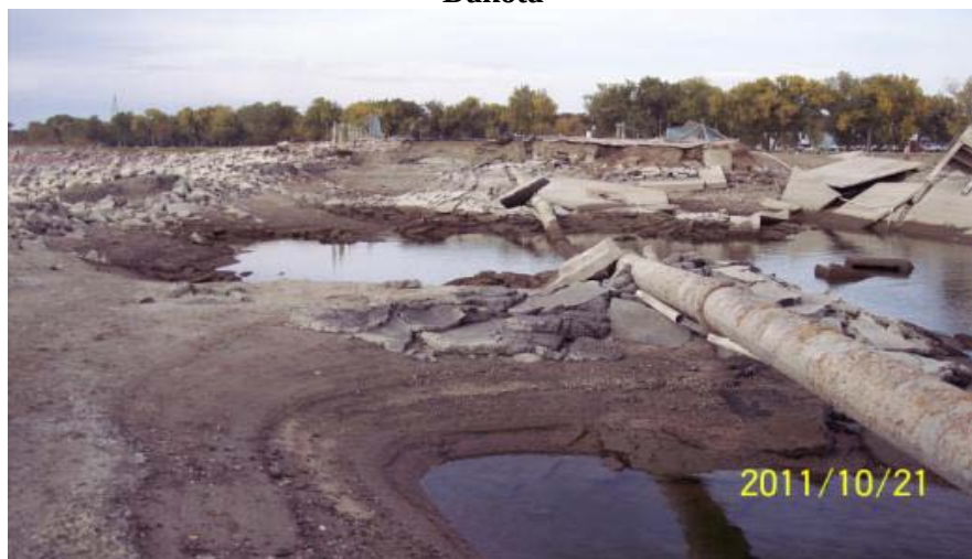
Figure 85. Damage/erosion: LaFramboise Island Causeway - City of Pierre waterlines damaged at LaFramboise Island Causeway (Corps) in Pierre, South Dakota
