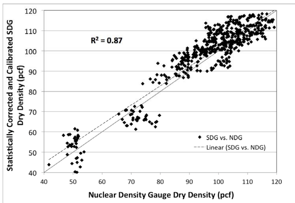
Figure 17. Comparison of NDG to SDG dry density with statistical correction and calibrated to one known density point in the test section.
