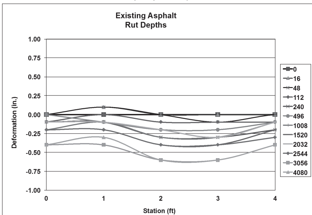
Figure C53. Rut depth measurements on cross-section 2 ft after repair PHP-4 (existing asphalt pavement).
