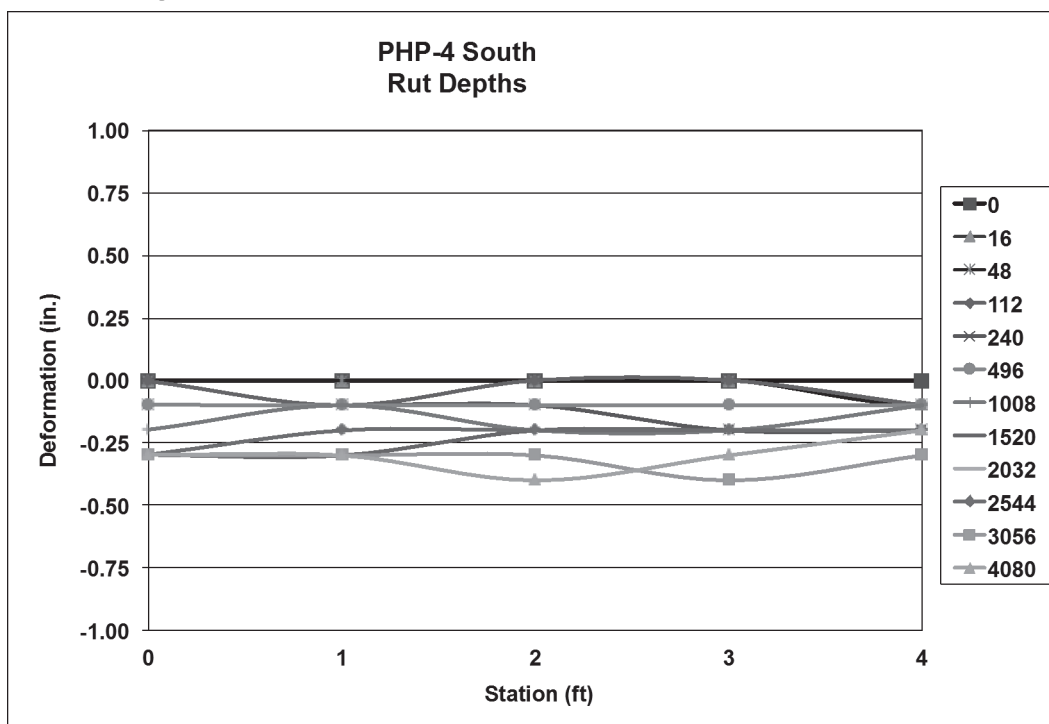
Figure C52. Rut depth measurements on south cross-section of PHP-4.
