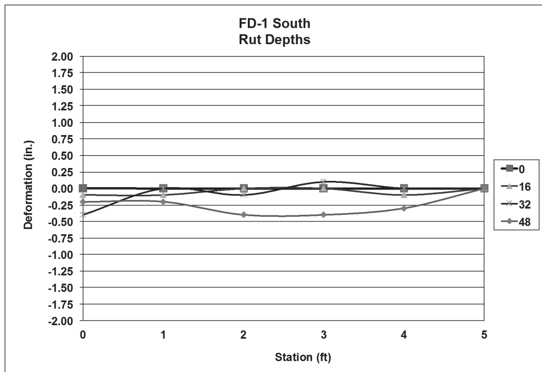
Figure C4. Rut depth measurements on south cross-section of FD-1.
