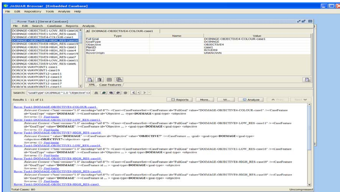
Figure 23. Rovers case base and query example.
