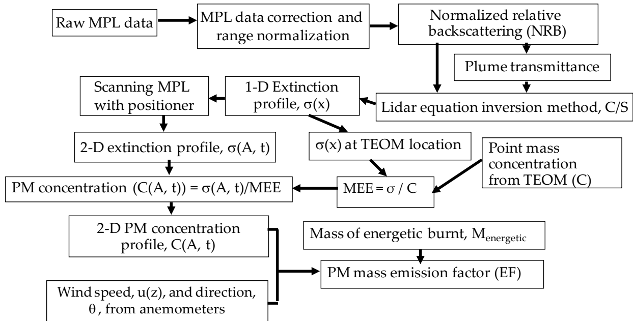
Figure 2-13. Schematic describing measurements and use of results to determine PM mass emission factor.
