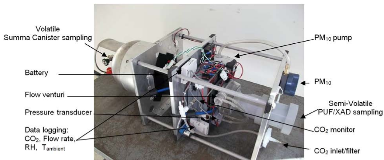
Figure 2-2. Instrumentation on the Flyer, GPS not in picture.
