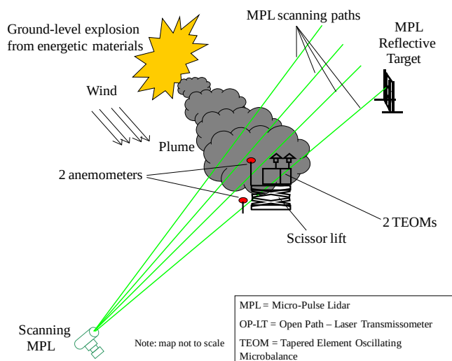
Figure 2-12. Schematic of open burning/open detonation operation and the ORS PM-10 measurement instrumentation.
