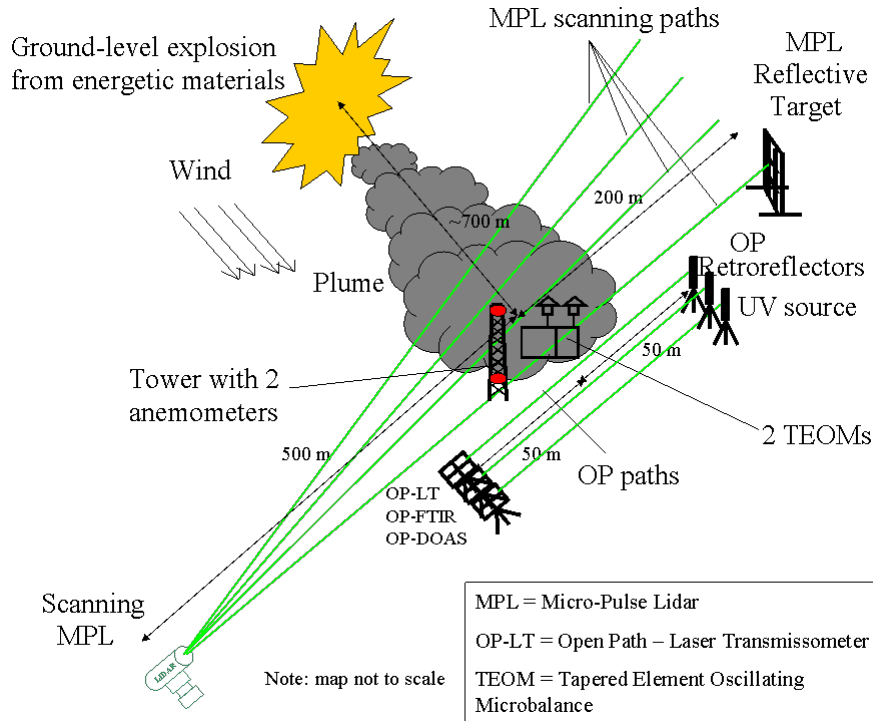
Figure 2-17. Schematic of open burning/open detonation operation and the ORS measurement instrumentation
