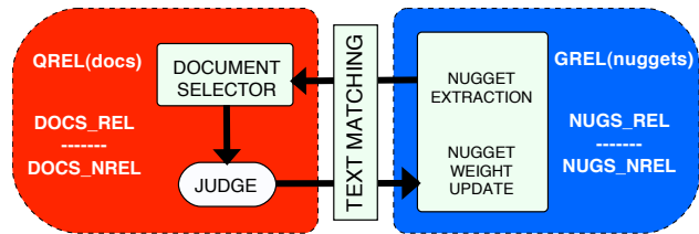
Figure 3: The overall design of assessment process: Iteratively, documents are selected and assessed, and nuggets are extracted and [re]weighted.
