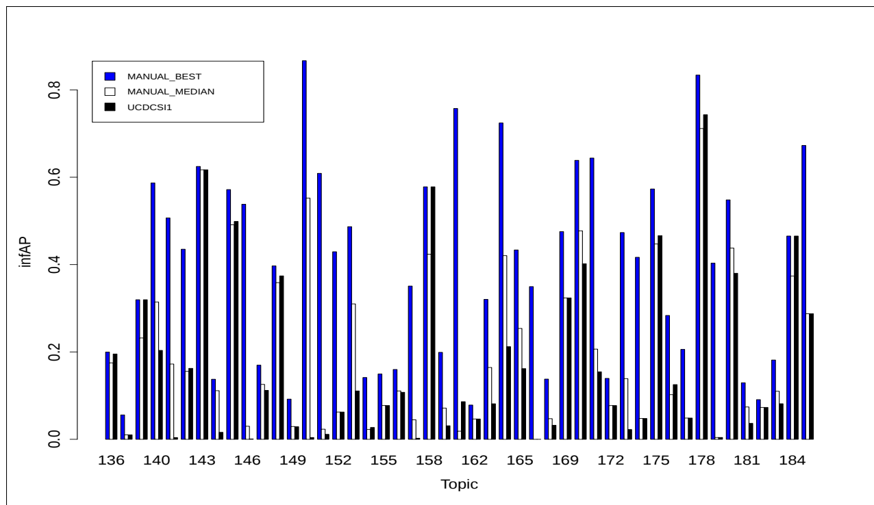
Figure 1: infAP Max, Median and UCDCSrun1 scores per topic
