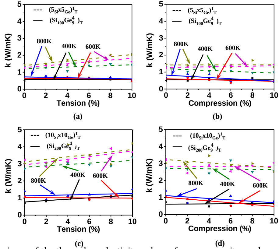
Fig. 21 Comparisons of the thermal conductivity values of nanocomposites and superlattices of equal thickness as a function of strain. Plots are (a) for \text{Si}_{100}\text{Ge}_9^4 and (5\text{Si} \times 5\text{Ge})_1^1 under tension, (b) for \text{Si}_{100}\text{Ge}_9^4 and (5\text{Si} \times 5\text{Ge})_1^1 under compression, (c) for \text{Si}_{200}\text{Ge}_9^4 and (10\text{Si} \times 10\text{Ge})_1^1 under tension, and (d) for \text{Si}_{200}\text{Ge}_9^4 and (10\text{Si} \times 10\text{Ge})_1^1 under compression at 400 K, 600 K and 800 K.
