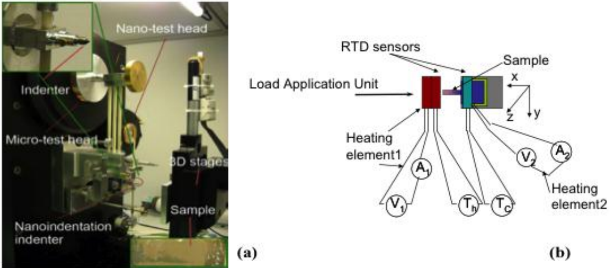
Fig. 1 (a) Experimental setup of simultaneous compressing and measuring thermal conductivity as a function of mechanical deformation and temperature and (b) schematic of the experimental arrangement.
