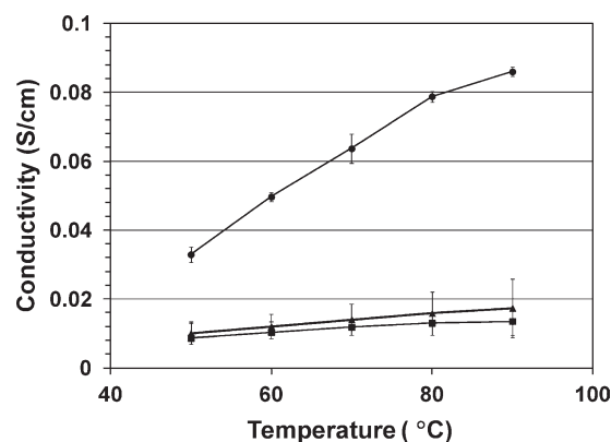
FIGURE 10 Conductivity of ATMPP 4 membrane in its bromide (■), carbonate (▲), and hydroxide (●) forms as a function of temperature at 95% RH.
