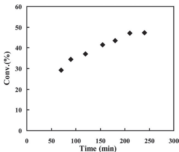
FIGURE 1 Time dependence of conversion for polymerization of [VBtMA][BF 4 ] by ATRP. [[\text{VBtMA}][\text{BF}_4]]_0/[\text{initiator}]_0/[\text{CuBr}]/[\text{HMTETA}]_0 = 100:1:1:1 and [\text{VBtMA}][\text{BF}_4] = 1.9\text{ M} .
