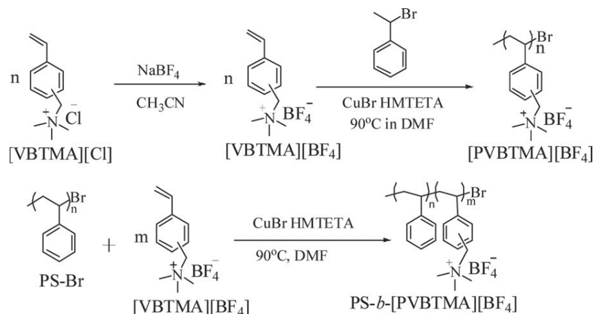
SCHEME 1 Synthesis of poly(vinyl benzyl trimethylammonium tetrafluoroborate) [PVBtMA][BF 4 ] homopolymers and polystyrene- b -poly(vinyl benzyl trimethylammonium tetrafluoroborate) PS- b -[PVBtMA][BF 4 ] block copolymers.
