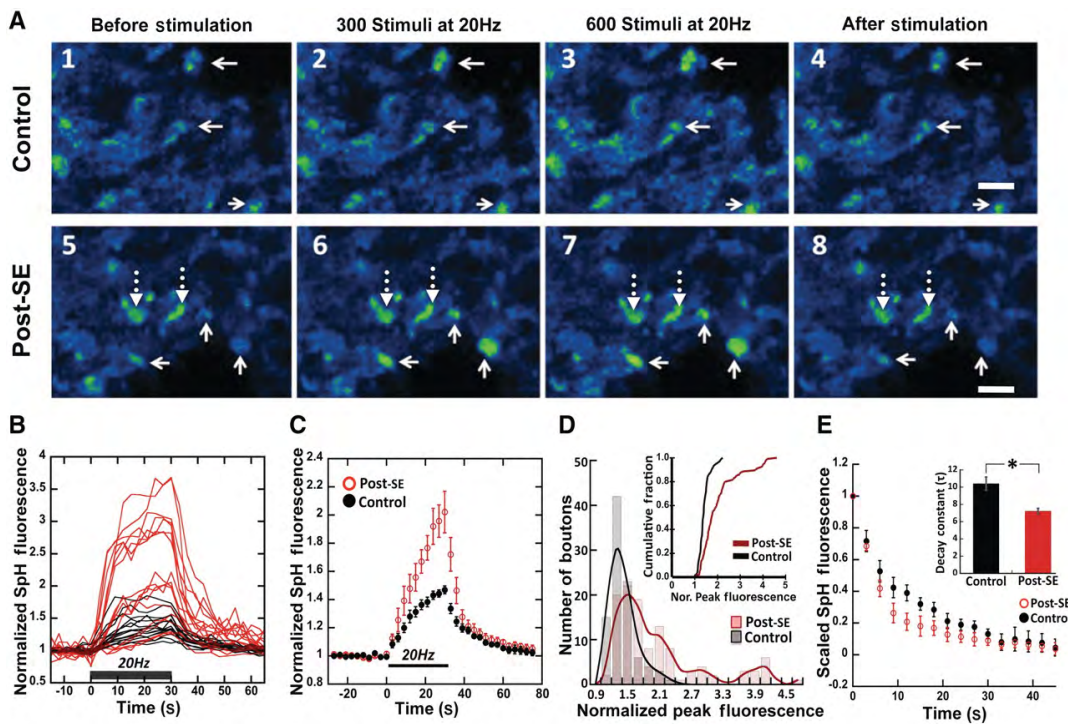
Figure 3: Pilocarpine-induced SE enhances vesicular release and endocytosis at mossy fiber terminals in CA3 stratum lucidum . (A) Two-photon images from control and post-SE SpH-expressing MFBs in proximal apical dendritic region of CA3 neurons. Solid arrows indicate puncta that showed activity-driven fluorescence changes during a 600 pulse 20 Hz stimulus train. The broken arrows in the lower panel show slowly fluorescing boutons in the epileptic slices. (Scale bar = 5 \mu\text{m} )
