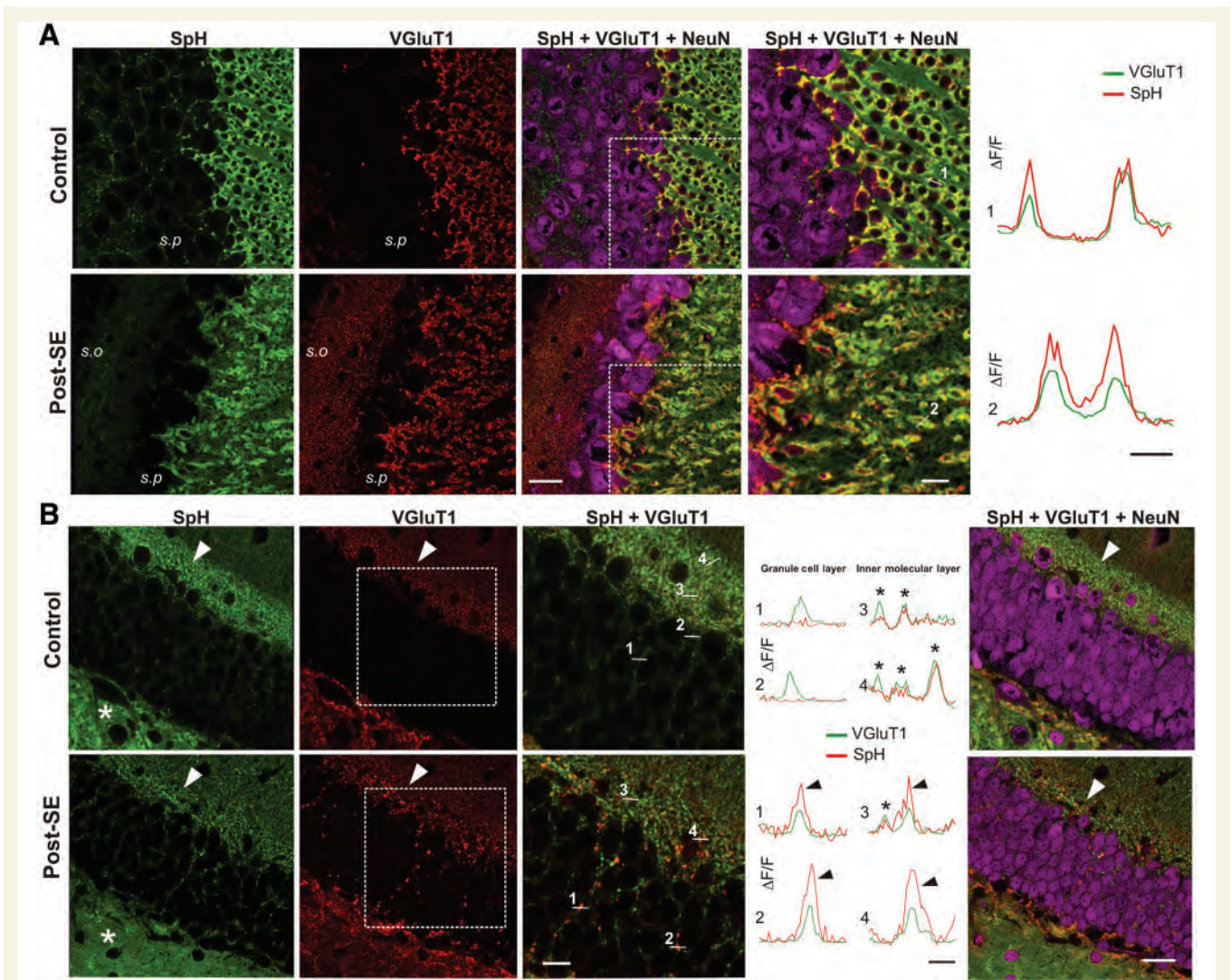
Figure 2 Confocal images of SpH, VGluT1 and NeuN expression in CA3 ( A ) and dentate granule cell ( B ) layers of control and post-status epilepticus (SE) SpH transgenic mice. ( A ) Native SpH fluorescence image (green), VGluT1 immunofluorescence image (red) and NeuN immunofluorescence image (purple) in control and post-status epilepticus mice showing co-localization of SpH with VGluT1 labelling in MFBs. A dramatic loss of cells was noticed in CA3 stratum pyramidale by NeuN staining (SpH + VGluT1 + NeuN, column 3) and SpH and VGluT1-positive terminals appear disorganized in stratum lucidum of post-status epilepticus compared with controls (SpH + VGluT1 + NeuN, column 4). Punctate SpH signals were also scattered through the pyramidal cell layer (s.p) surrounding cell somata that were stained with NeuN antibody. The column on the right (column 4) shows fluorescence intensity profile and co-localization along line scans (1: control and 2: post-status epilepticus) through single MFBs indicated in the respective \times 2 magnification images (scale bar = 25 \mu\text{m} ) of the rectangular boxes seen in column 3 (scale bar = 50 \mu\text{m} ). Scale bar for line scans = 2 \mu\text{m} . ( B ) In the dentate granule cell layer of control and post-status epilepticus, (NeuN labelling), SpH fluorescence (green) and VGluT1 immunofluorescence (red) were intense in the hilus (asterisk) and in the inner molecular layer (arrow head). In the control ( B , top row) SpH-positive puncta around putative granule cell somata were devoid of VGluT1 expression (line plots: lines 1 and 2), while SpH and VGluT1 signals co-localized in the inner molecular layer (line plots: lines 3 and 4), as shown by respective line scans of fluorescence intensity through puncta in the granule cell layer (1 and 2) versus the inner molecular layer (3 and 4). In post-status epilepticus ( B , bottom row) SpH and VGluT1 co-localize in both the dentate granule cell layer (SpH + VGluT1) and inner molecular layer. NeuN immunofluorescence illustrates a lack of marked granule cell loss in post-status epilepticus dentate gyrus (SpH + VGluT1 + NeuN). Stratum oriens scale bar = 2 \mu\text{m} .
