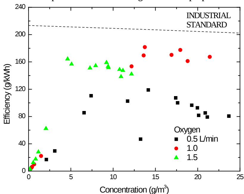
Figure 8. Dependence of reactor efficiency on \text{O}_3 concentration for a composite reactor fabricated by stacking six layers of 6 parallel microchannels with a channel depth of 200 \mu\text{m} and a width of 500 \mu\text{m} .
