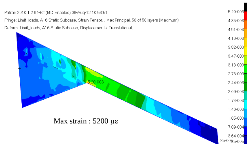
Figure 40: Lower skin strains
