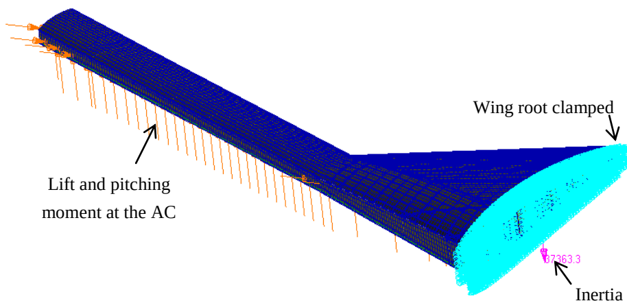
Figure 35: Loads and boundary conditions applied on the model
