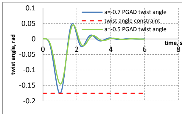
Figure 15. PGAD twist angle in response to gust
