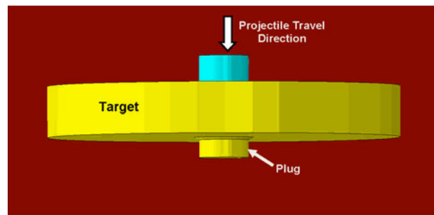
Fig. 6 Schematic representation of the plugging failure mechanism
