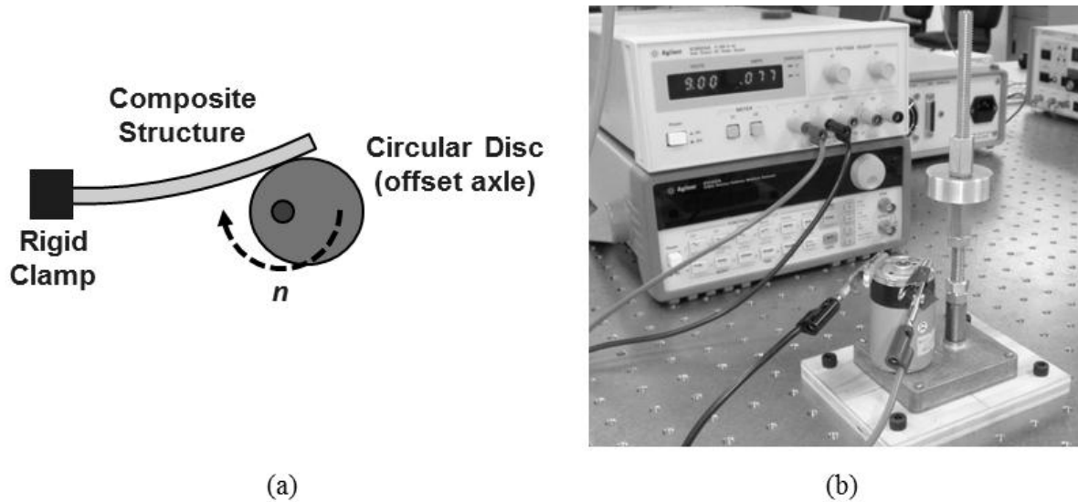
Figure 10: (a) Top view of the cyclic strain apparatus in contact with a rigidly clamped composite structure. As the disc rotates, the structure deflects accordingly. (b) Side view of the cyclic strain apparatus (foreground) with a DC voltage source (background) to provide the desired drive voltage. Here, 9.00 Volts DC are applied.
