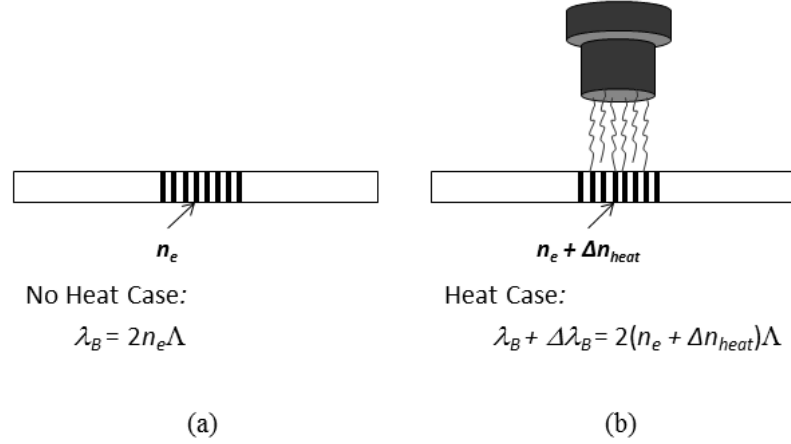
Figure 2: Diagrams show the effect of heat on the Bragg wavelength. (a) With no heat applied, \lambda_B follows Equation (1) as expected. (b) If the FBG is exposed to a heat source (i.e. a heat gun), then \lambda_B experiences a positive shift of \Delta\lambda_B .
