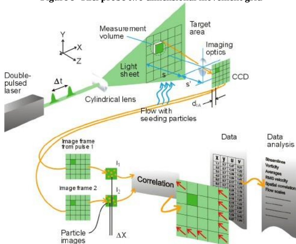
Figure 10-PIV visual explanation- Dantec Dynamics (2012)
