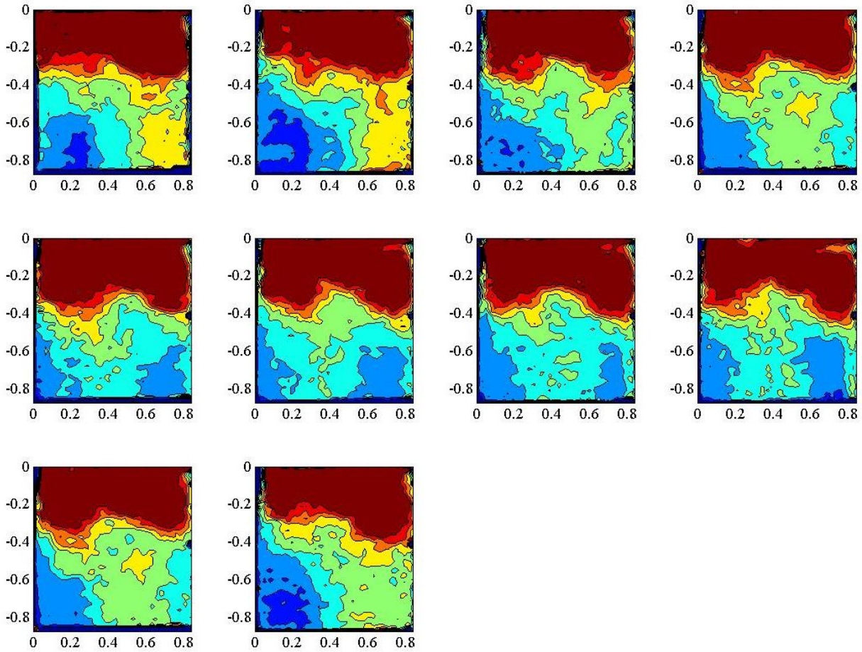
Figure 60 – w'/u_1 in the 2 plane for the case with a 2 mm tip gap and wakes. The phases are separated by a time delay of t=0.1T
