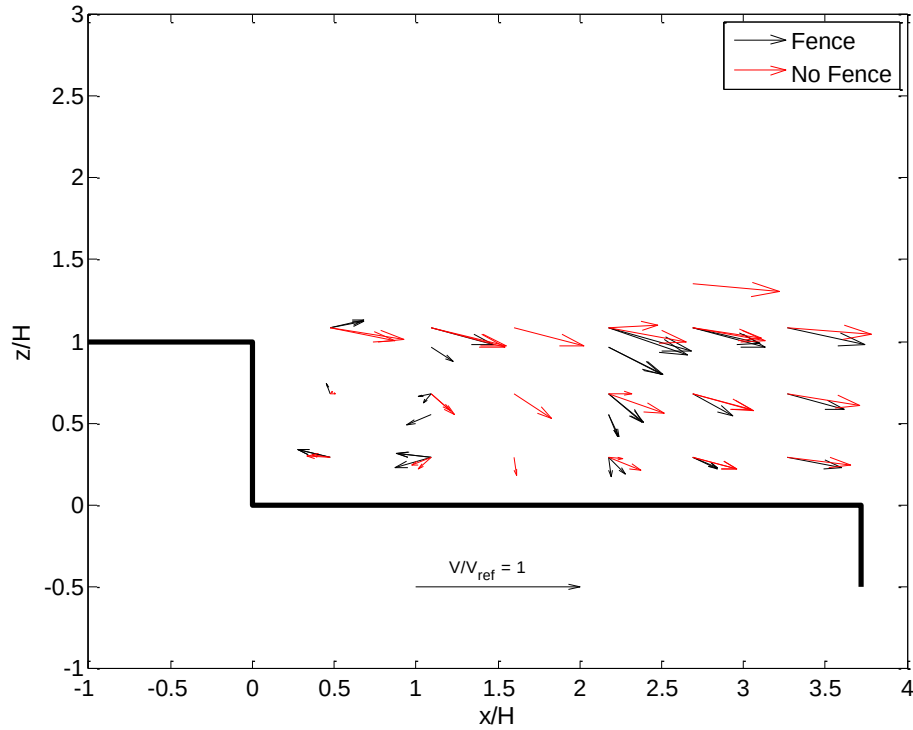
Figure 34. In situ data at y/H = 0 for \beta = 15^\circ
