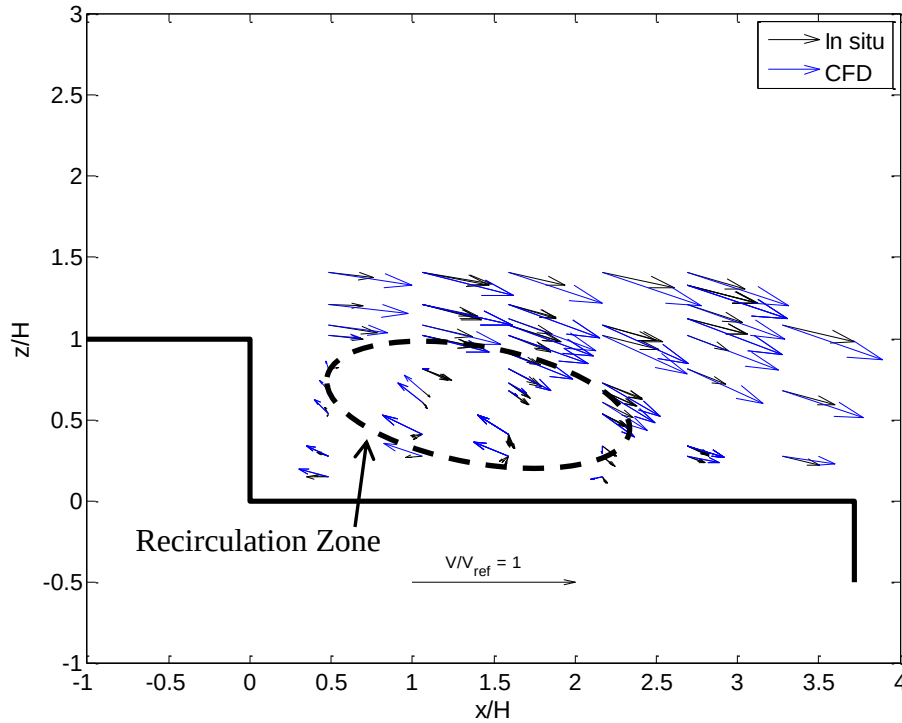
Figure 11. In situ vs. CFD at y/H = 0 for \beta = 0^\circ with 7 kt uniform CFD inflow
