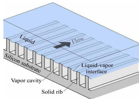
Figure 5: Superhydrophobic Surface (BYU 2013)
