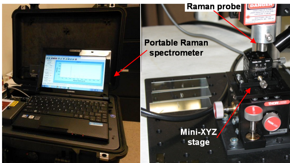
Figure 32. Illustration of a portable Raman sensor coupled with a fiber-optic Raman probe and a miniaturized XYZ stage.
