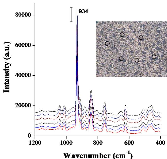
Figure 7. SERS spectra of \text{ClO}_4^- ( 1 \times 10^{-5} M) obtained from six randomly selected spots (inset) on a substrate made of DMAE-modified Au nanoparticles. Each spectrum was offset for the clarity of presentation, and the error bar represents a standard deviation of about 16% at peak position 934 \text{ cm}^{-1} .
