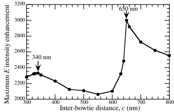
Fig. 5. The maximum E intensity enhancement at plasmon resonance as a function of the inter-bowtie distance along the polarization direction, c , for fixing the inter-bowtie distance along the direction normal to the polarization as 300 nm and truncated apex with w = 10 nm and d = 10 nm.
