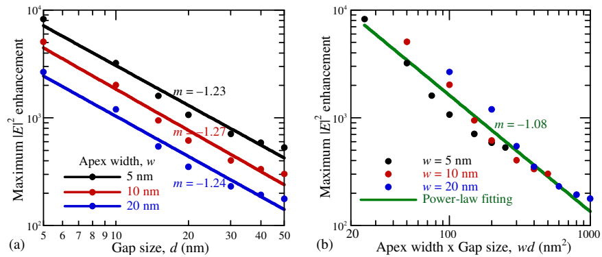
Fig. 4. The maximum E intensity enhancement at plasmon resonance as a function of (a) the gap size, d , for apex widths w of 5, 10, and 20 nm and (b) the product of the apex width and the gap size, wd . (symbols: FDTD data; lines: power-law fitting)
