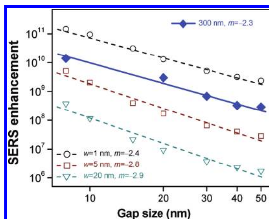
FIGURE 3. Comparison of the FDTD calculated maximum field |E|^4 enhancement (dashed lines with open symbols) for apex widths w = 1, 5 , and 20 nm with the experimentally determined SERS enhancement (solid line with solid diamonds) as a function of nanogap size for elevated bowtie arrays with ccd = rrd = 300 nm (III in Figure 2). The slope is determined by fitting the power-law relationship of EF \propto |E|^4 = Ad^m to the data.
