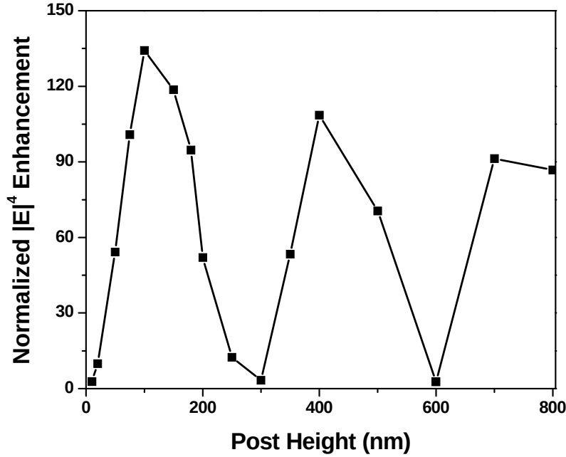
Figure 24. The calculated maximum field enhancement |E|^4 normalized by that without the Si post as a function of the post height showing the characteristics of nanocavity resonance.
