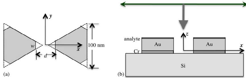
Fig. 1. Schematics showing (a) a truncated bowtie on the x - y plane and (b) the cross-section of Si/Cr/Au bowtie/ p -aminothiophenol nanostructure on the x - z plane. A polarized plane wave is illuminated from the bowtie side.
