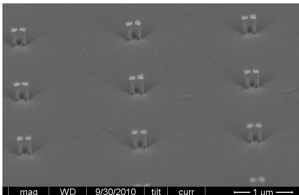
Figure 22. SEM image of bowtie arrays using a backscattered electron detector. The technique is used to distinguish heavy element gold (white triangles) from light element Si (gray posts).
