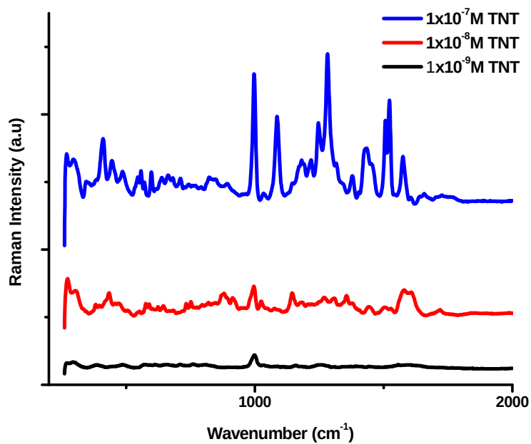
Figure 13. SERS detection of TNT at varying concentrations (from about 0.23 to 23 \mu\text{g/L} ) using Au nanoparticles as a SERS substrate.
