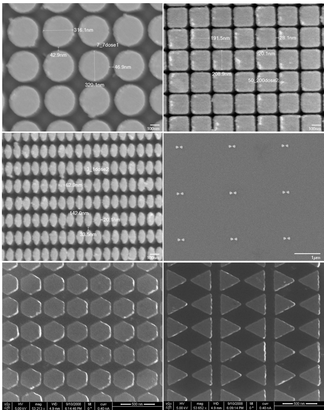
Figure 16. Scanning electron micrographs (SEM) and examples of SERS patterns fabricated by EBL and lift-off techniques after the deposition of 40 nm gold.
