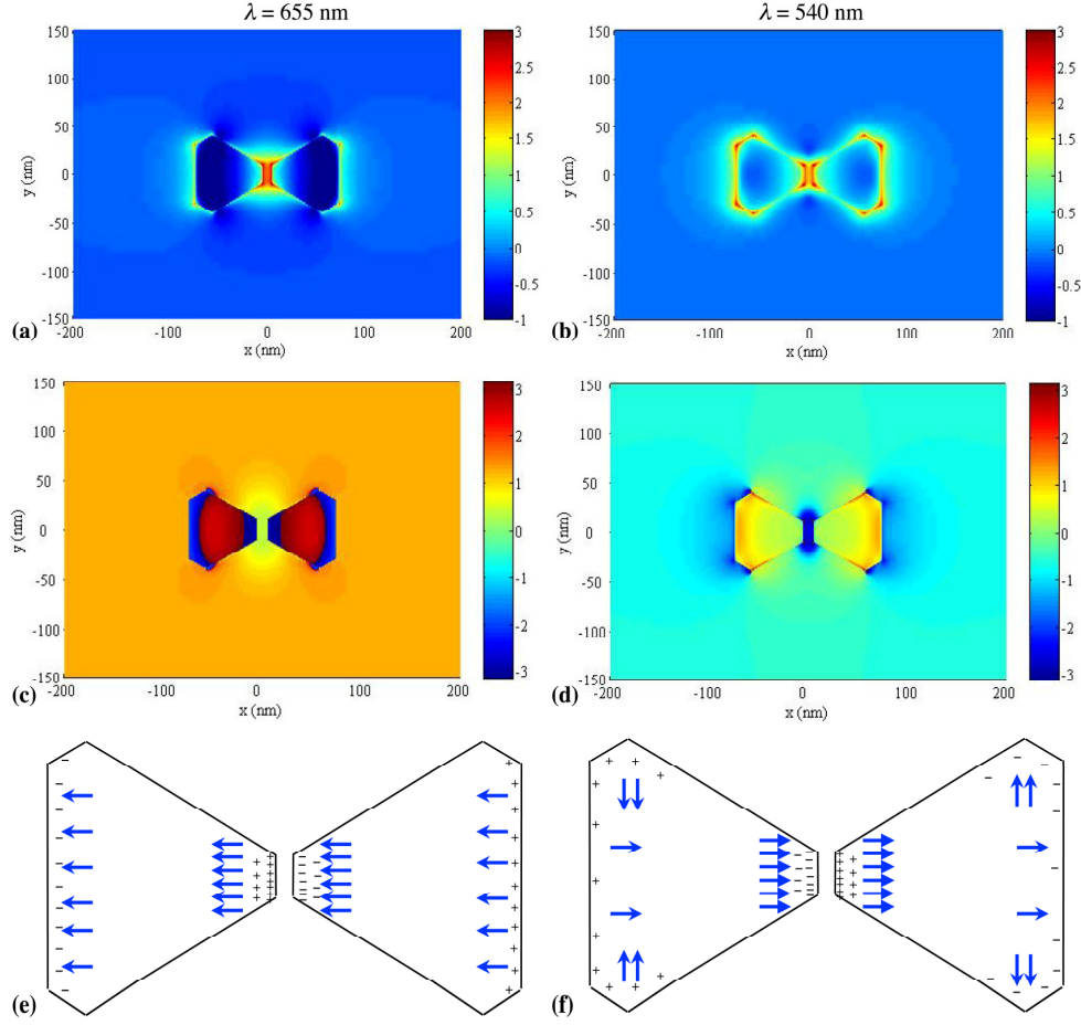
Fig. 3. The E intensity enhancement profiles on the plane containing the bowtie surface for (a) \lambda = 655 nm with dipole resonance and (b) \lambda = 540 nm with quadrupole resonance. The color bar is logarithmic-scale and limited to -1 to 3 . The corresponding phase profiles of E_x for (c) \lambda = 655 nm and (d) \lambda = 540 nm, and schematics showing the bound surface charge distribution on the bowtie surface and the major polarizations for (e) \lambda = 655 nm and (f) \lambda = 540 nm. The apex is truncated with w = 20 nm and the gap size, d , is 10 nm.
