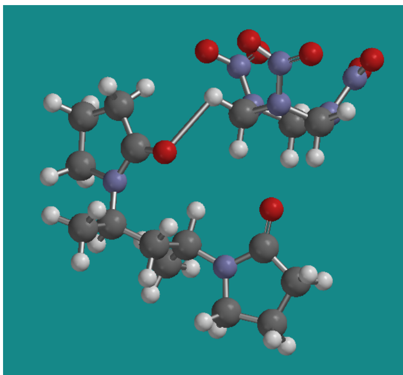
Figure 14. Calculated structure of the RDX complex with pyrrolidone. RDX shows a bowl-like shape (upper right of the figure).
