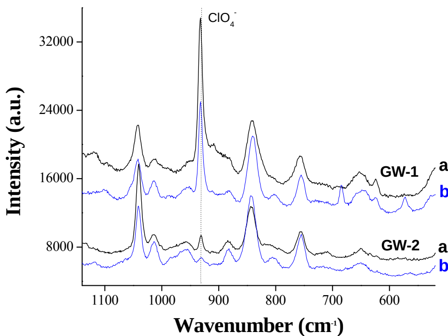
Figure 9. SERS spectra of two contaminated groundwater samples (GW-1 and GW-2) without dilution (a) or with a 10x dilution (b).
