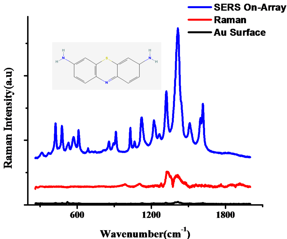
Figure 18. Illustration of nanostructure SERS substrate efficiency, spectra from top to bottom are: nanofabricated SERS substrate (T_1) of thionine ( 1 \times 10^{-7} M); thionine ( 1 \times 10^{-7} M) Raman spectrum dry on glass slide; and spectra of 1 \times 10^{-7} M thionine on flat Au surface.
