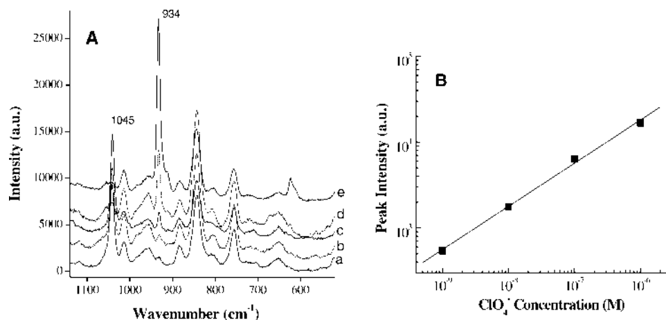
FIG. 3. (A) SERS spectroscopic analysis of \text{ClO}_4^- in the presence of background electrolytes of \text{SO}_4^{2-} , \text{PO}_4^{3-} , and \text{NO}_3^- at 10^{-4} M each, and \text{Cl}^- at 10^{-3} M. Perchlorate concentrations varied from (a) 0, (b) 10^{-9} , (c) 10^{-8} , (d) 10^{-7} , to (e) 10^{-6} M. (B) A log-log plot of the peak intensity at 934 \text{cm}^{-1} against the \text{ClO}_4^- concentration.
