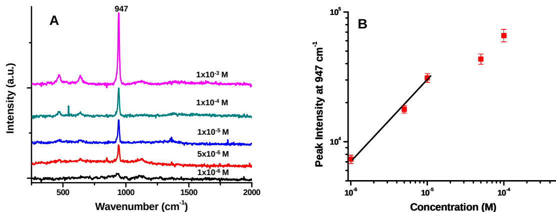
Figure 33. (A) Detection and spectral analysis of perchlorate ( \text{ClO}_4^- ) at varying concentrations using a portable Raman sensor. (B) A log-log plot of the peak intensity at 947 \text{cm}^{-1} as a function of the \text{ClO}_4^- concentration.
