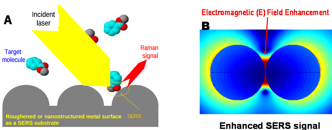
Figure 1. Schematic illustration of surface enhanced Raman scattering that occurs as a result of the excitation of surface plasmons localized on roughened noble metal surfaces when illuminated by a laser light.
