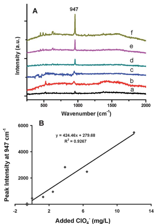
Fig. 4 SERS determination of \text{ClO}_4^- in a contaminated groundwater sample (GWOBOD03) by the standard addition method. (A) SERS spectra with the addition of varying concentrations of \text{ClO}_4^- at (a) 0, (b) 0.01, (c) 0.03, (d) 0.04, (e) 0.07, and (f) 0.12 mM. (B) The calibration curve for determining the actual \text{ClO}_4^- concentration in groundwater.
