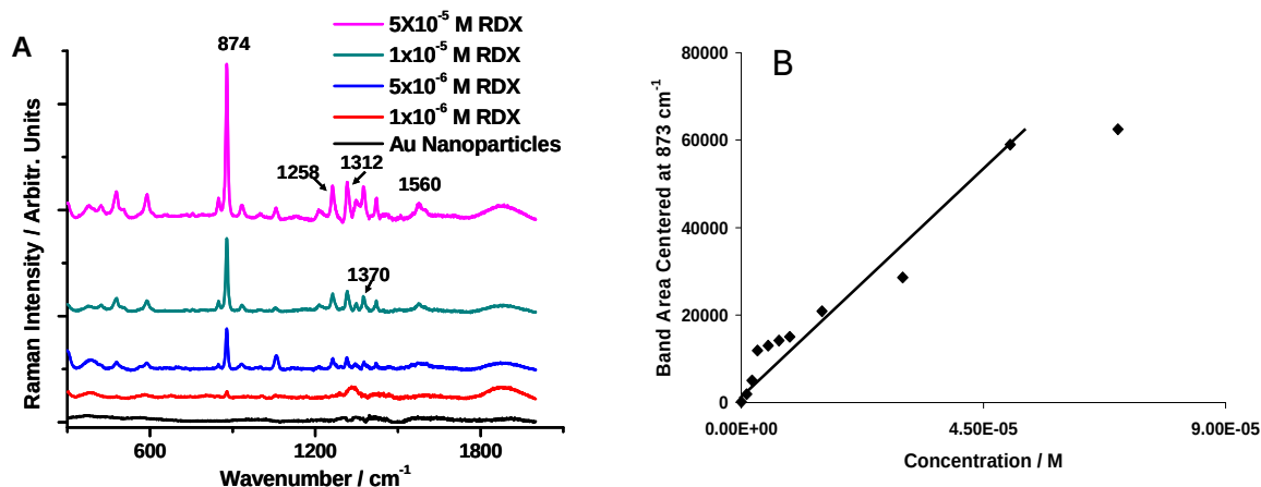
Figure 10. (A) SERS spectra of RDX at concentrations ranging from 1 \times 10^{-6}\text{ M} to 5 \times 10^{-5}\text{ M} . Laser power was \sim 1\text{ mW} at the exit of the microscope objective, and the scan time was \sim 10\text{ s} . (B) Peak area at 873\text{ cm}^{-1} as a function of RDX concentration.
