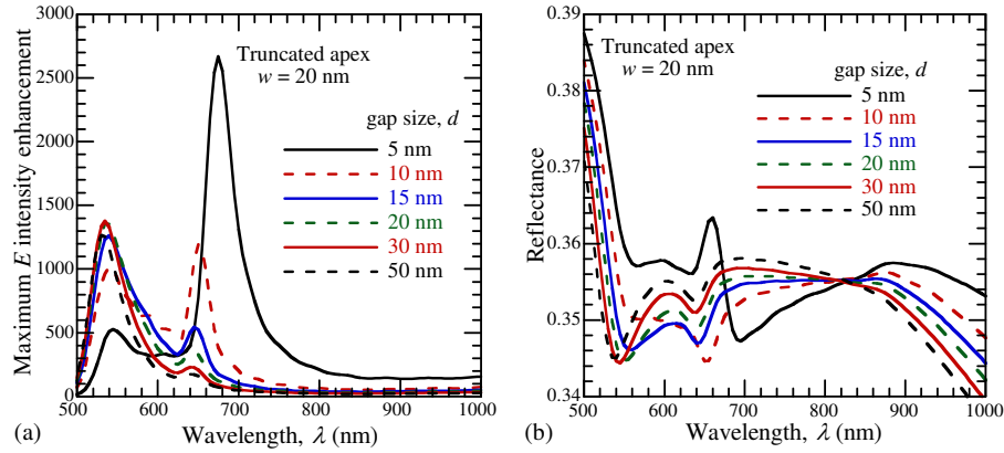
Fig. 2. (a) Maximum E intensity enhancement at the apex and on the bowtie surface and (b) the reflectance as functions of the illumination wavelength, \lambda , at different gap sizes. The width of the truncated apex, w , is 20 nm.
