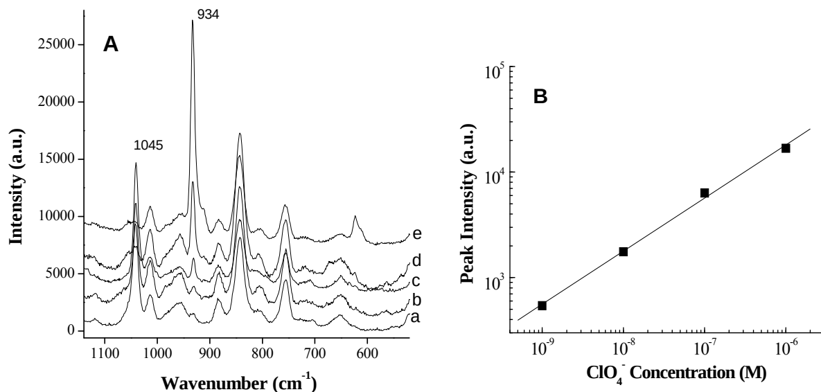
Figure 8. (A) SERS spectroscopic analysis of \text{ClO}_4^- in the presence of background electrolytes of \text{SO}_4^{2-} , \text{PO}_4^{3-} , and \text{NO}_3^- at 10^{-4} M each and \text{Cl}^- at 10^{-3} M. Perchlorate concentrations varied from a: 0, b: 10^{-9} , c: 10^{-8} , d: 10^{-7} , to e: 10^{-6} M. (B) A log-log plot of the peak intensity at 934\text{ cm}^{-1} against the \text{ClO}_4^- concentration.
