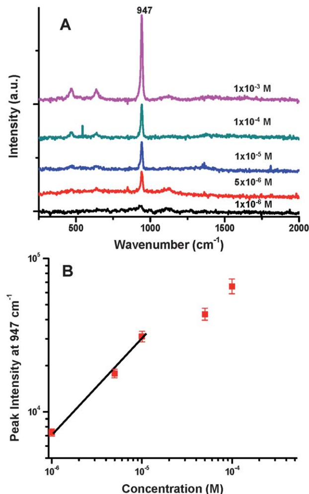
Fig. 2 (A) Detection and spectral analysis of perchlorate ( \text{ClO}_4^- ) at varying concentrations using a portable Raman sensor. (B) A log-log plot of the peak intensity at 947 \text{ cm}^{-1} as a function of the \text{ClO}_4^- concentration.
