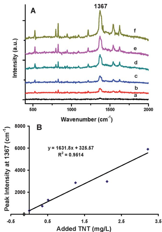
Fig. 5 SERS determination of TNT in a contaminated groundwater sample (MW38) by the standard addition method. (A) SERS spectra with the addition of varying concentrations of TNT standard at (a) 0, (b) 1.6, (c) 2.3, (d) 5.5, (e) 9.3, and (f) 14.0\text{ }\mu\text{M} , and (B) the calibration curve for determining the actual TNT concentration in groundwater.
