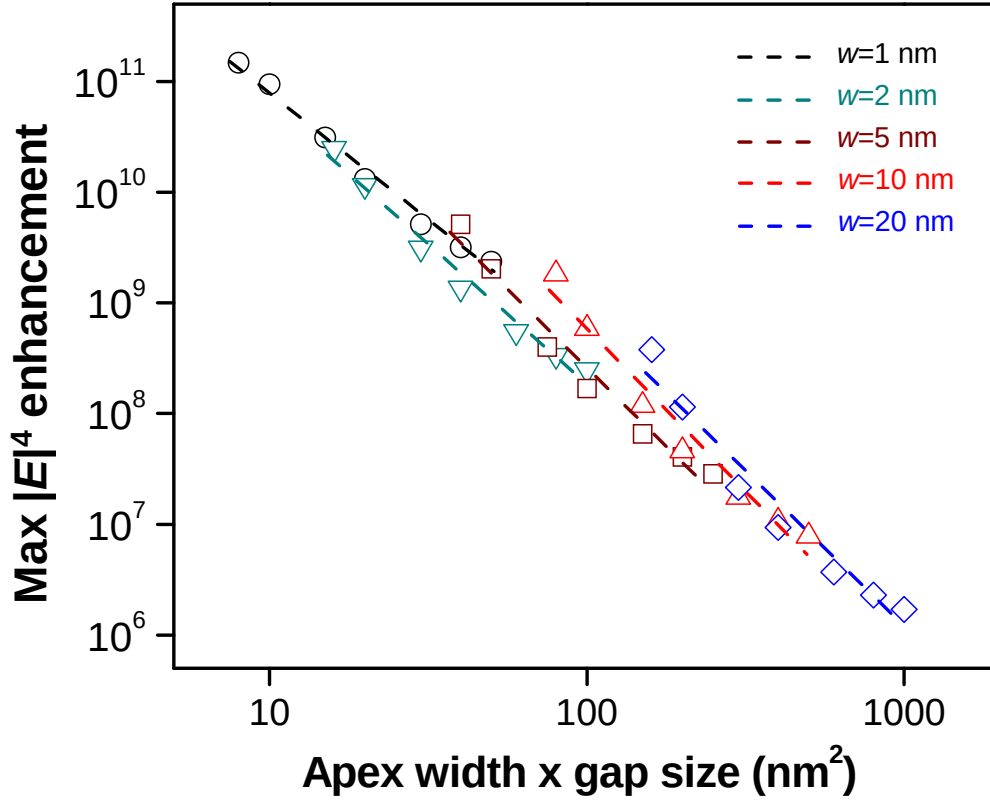
Figure 26. The maximum field enhancement |E|^4 calculated by FDTD as a function of the product of the apex width and the gap size, wd , for varying apex widths. The open symbols are FDTD data and the lines are the power-law fit. The inter-bowtie distances are ccd = rrd = 300 nm. The diameter of the Si posts is 40 nm, and the height is 200 nm. The calculated slope falls in a narrow range of about -2.5 .
