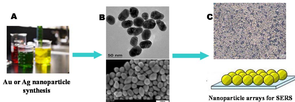
Figure 2. Illustration of wet-chemical synthesis of gold or silver nanoparticles, which are subsequently used to form nanoparticle thin films as SERS substrates for chemical analysis.
