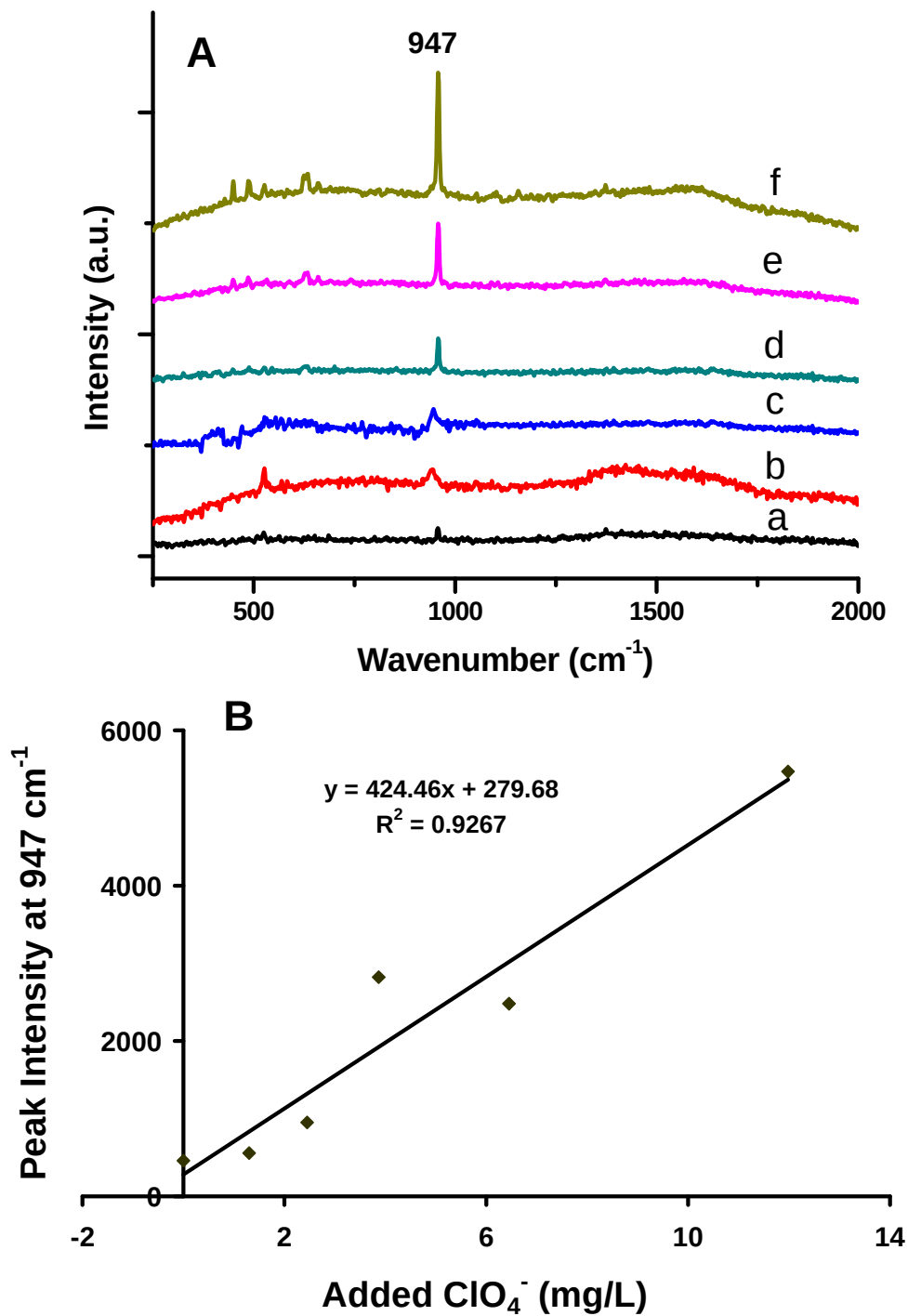
Figure 35. SERS determination of \text{ClO}_4^- in a contaminated groundwater sample (GWOBOD03) by the standard addition method. (A) SERS spectra with the addition of varying concentration of \text{ClO}_4^- at (a) 0, (b) 0.01, (c) 0.03, (d) 0.04, (e) 0.07, and (f) 0.12 mM. (B) The calibration curve for determining the actual \text{ClO}_4^- concentration in groundwater.
