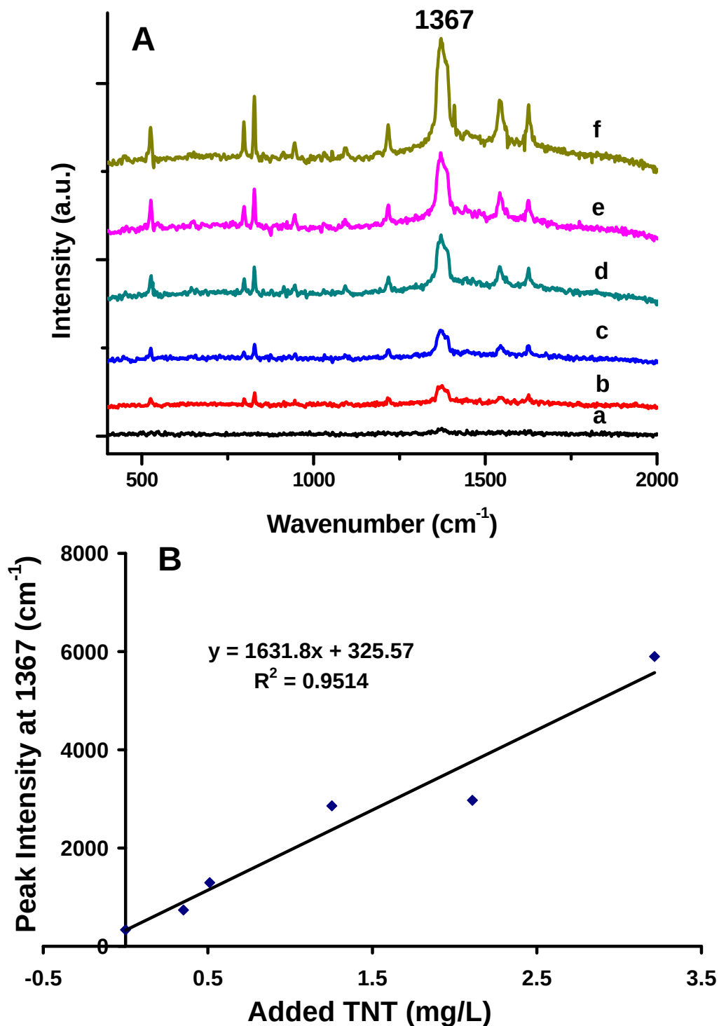
Figure 36. SERS determination of TNT in a contaminated groundwater sample (MW38) by the standard addition method. (A) SERS spectra with the addition of varying concentrations of TNT standard at (a) 0, (b) 1.6, (c) 2.3, (d) 5.5, (e) 9.3, and (f) 14.0 \mu\text{M} , and (B) the calibration curve for determining the actual TNT concentration in groundwater.
