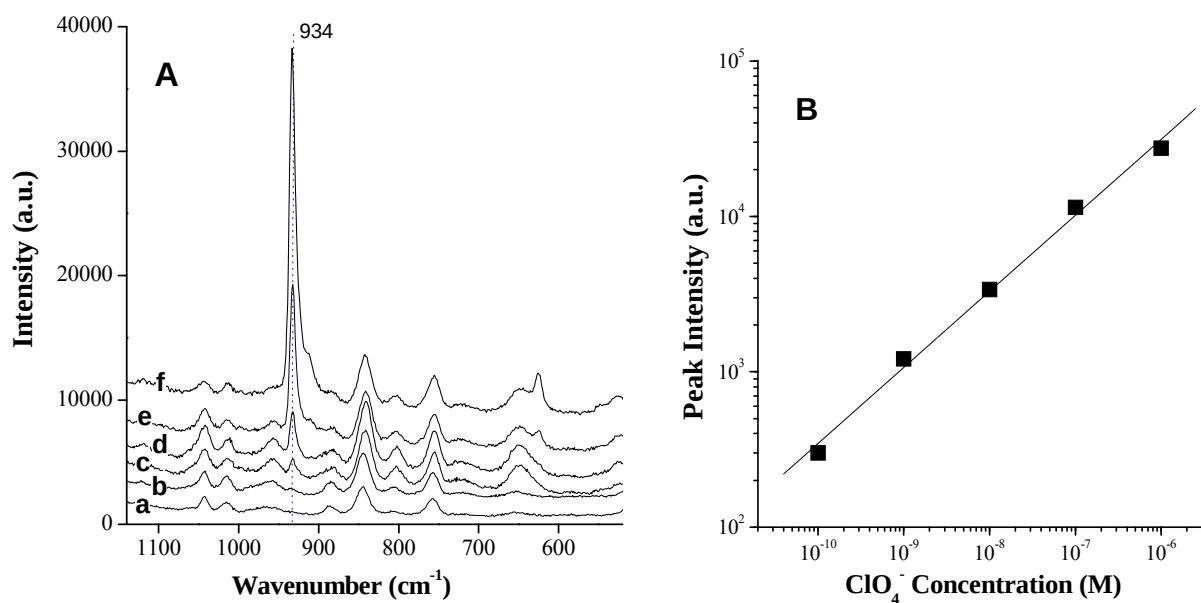
Figure 6. (A) Raman spectroscopic analysis of \text{ClO}_4^- at concentrations of a: 0, b: 10^{-10} , c: 10^{-9} , d: 10^{-8} , e: 10^{-7} , and f: 10^{-6} M using DMAE-modified Au nanoparticles as a SERS substrate; (B) a log-log plot of the peak intensity at 934\text{ cm}^{-1} against the \text{ClO}_4^- concentration.
