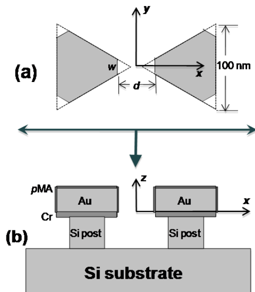
Figure 4. Schematic illustration (not to scale) of the top view of a bowtie structure in the x - y plane (a) and the cross-section in the x - z plane (b). The height of the gold bowtie is 40 nm with a sorbed analyte layer of 0.5 nm of p -mercaptoaniline ( p MA). The Cr adhesion layer is 8 nm, the Si post diameter is 40 nm, and the post height is 200 nm.
