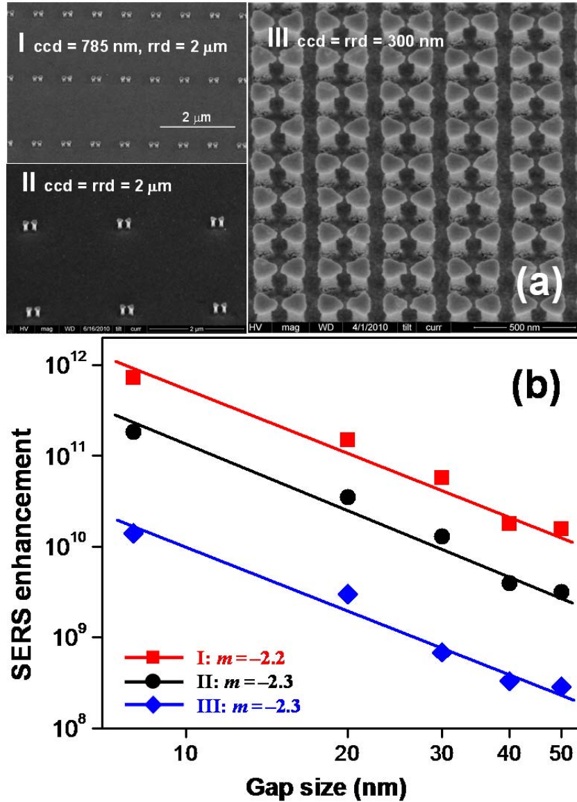
Figure 23. Determination of the gap size dependence and the long-range collective plasmonic effects in SERS enhancement using elevated gold bowtie nanoantenna arrays. (a) SEM images of the elevated gold bowtie arrays with varying center-to-center distance (ccd) in rows along the bowtie axis, and row-to-row distance (rrd). (b) A log-log plot of SERS enhancement factors ( EF ) as a function of bowtie nanogap size in arrays I, II, and III with different bowtie spacing. The slope ( m ) is determined by fitting the power-law relationship of EF \propto Ad^m to the experimental data.
