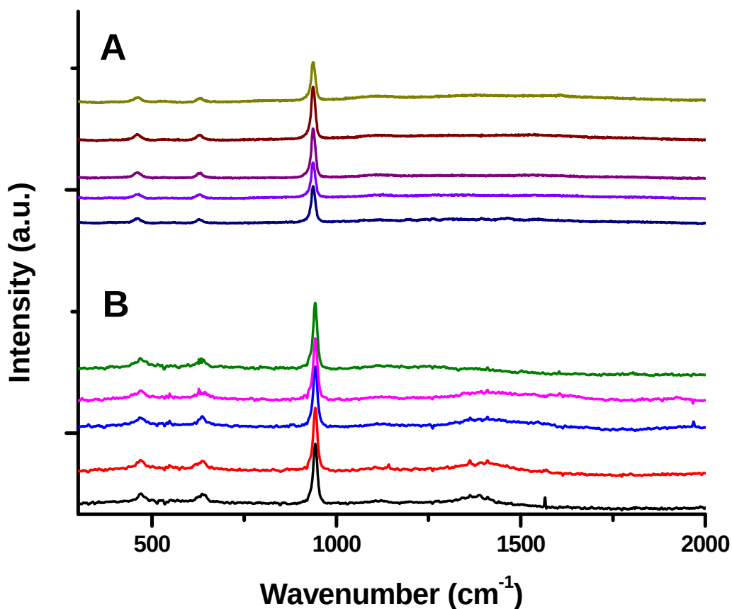
Figure 34. Reproducibility evaluation of the SERS sensor: (A) SERS spectra of \text{ClO}_4^- ( 1 \times 10^{-4} M) obtained from five different gold bowtie array substrates, and (B) spectra of \text{ClO}_4^- ( 5 \times 10^{-3} M) obtained from five different spots on a single gold bowtie array substrate.
