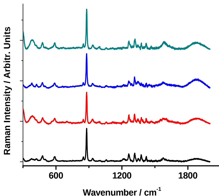
Figure 11. SERS spectra of 5\times 10^{-5}\text{ M} RDX using different batches of Au nanoparticles as SERS substrates for reproducibility evaluation.
