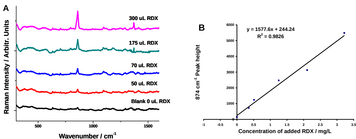
Figure 12. (A) SERS spectra of a contaminated groundwater sample using the standard addition method. (B) Standard addition curve for determining the RDX concentration (0.12 mg/L analyzed by HPLC) in groundwater.
