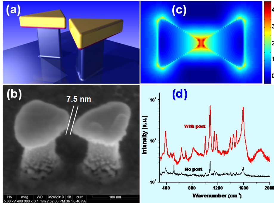
Figure 21. (a) Schematic illustration of elevated gold bowties on top of Si posts etched into a Si wafer with a magenta colored Cr adhesion layer between the gold layer and the Si post. (b) Side view SEM image of a three-dimensional gold bowtie nanoantenna with a gap of 8 \pm 1 nm. (c) The spatial distribution of the E field intensity calculated by FDTD simulations. The intensity is given by a logarithmic scale color bar. (d) Comparison of SERS spectra of p -mercaptoaniline from elevated and non-elevated bowtie array substrates.
