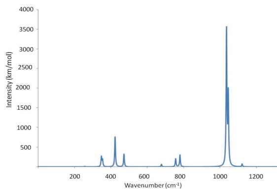
Figure 53. Calculated IR spectrum.
