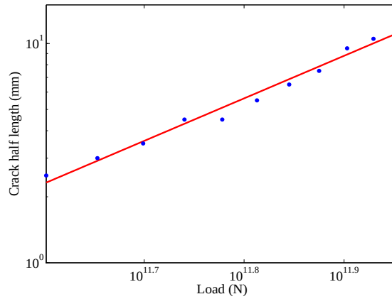
Figure 73. Crack half length versus load for a center crack problem using bond-based peridynamics.
