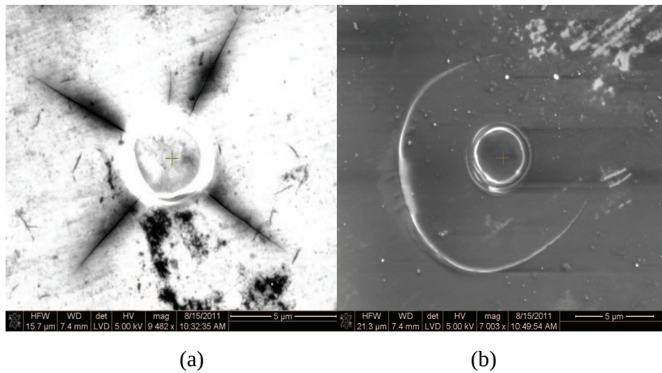
Figure 32. SEM micrographs of fused silica indented to 1500 nm (a) radial cracks and (b) cone cracks.
