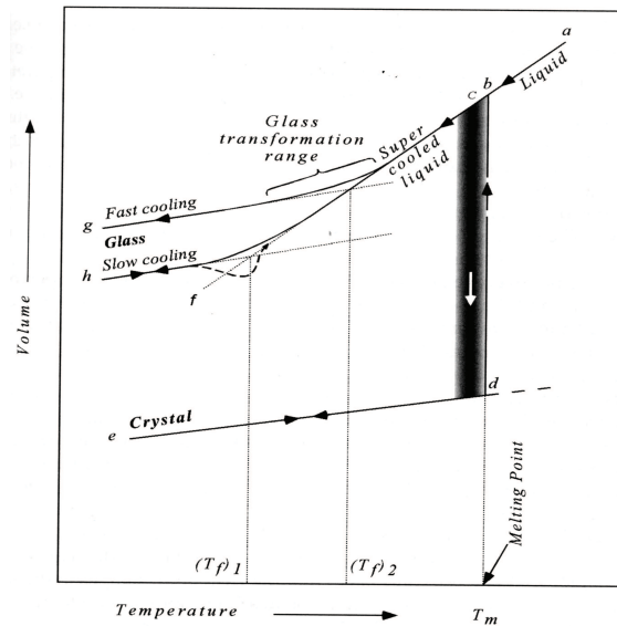
Figure 75. The volume-temperature diagram for a glass-forming liquid, after Varshneya (26).
