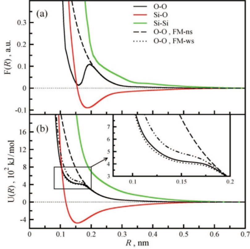
Figure 34. Effective atom-atom forces [panel (a)] and corresponding potentials [panel (b)] in liquid SiO_2 generated through the FM method as functions of interatomic separation: O - O (black), Si - O (red), and Si - Si (green). The dashed line corresponds to the model without the soft repulsive shoulder (FM-ns model). In panel (b), the dotted line corresponds to the FM model with a weaker repulsive shoulder (FM-ws model) and the dot-dot-dashed lines indicate the variation of the O - O repulsion in the FM procedure with a length of ab initio reference trajectories as discussed in (14).
