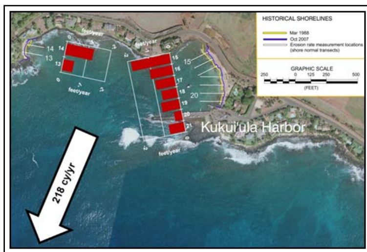
Figure 4. Kukulula Bay cell shoreline change rates and sediment budget, 1988-2007.
