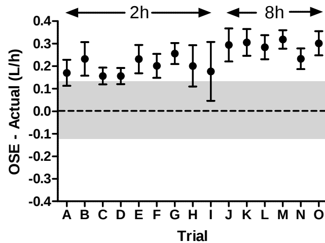
Figure 1: Differences between predicted sweat rate (OSE) and actual sweating rate during 2h (A through I) and 8h (J through O) trials. Data are group (trial) means; bars are 95% confidence intervals. Shaded area represents zone of indifference ( \pm 0.125 L/h) based on the desire to predict sweat losses to within 1L over an 8h work day. From reference 4.
