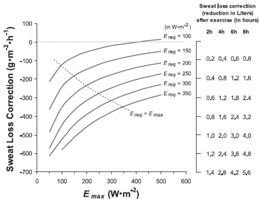
Figure 2: Sweat loss correction (left y-axis) and associated water volume error (right y-axis) observed when using OSE versus OSE c . Right y-axis volumes represent an overestimate of individual water needs (in liters) over time. From reference 13.
