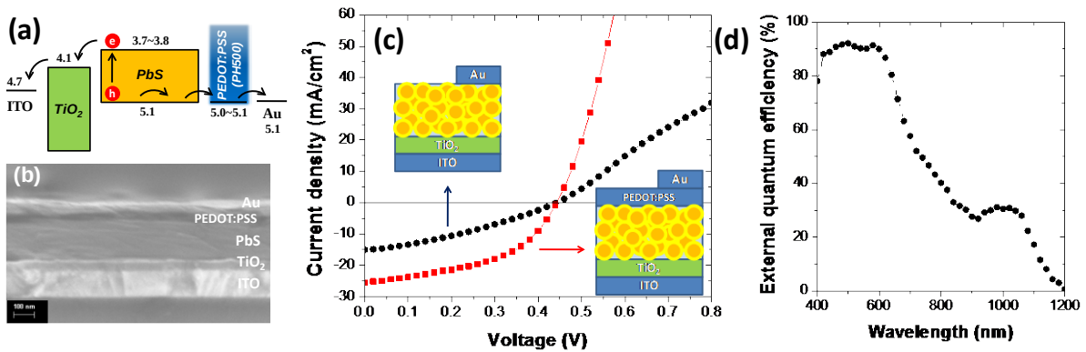
Figure 7: (a) Energy band diagram of the device structure, (b) The SEM image of the cross section of the devices, (c) I-V characteristics of the \text{TiO}_2 -PbS heterojunction device without (black) / with (red) a PEDOT:PSS layer under AM1.5G ( 100 \text{ mW}/\text{cm}^2 ) illumination, and (d) EQE spectrum of the \text{TiO}_2 -PbS heterojunction device with a PEDOT:PSS layer.
