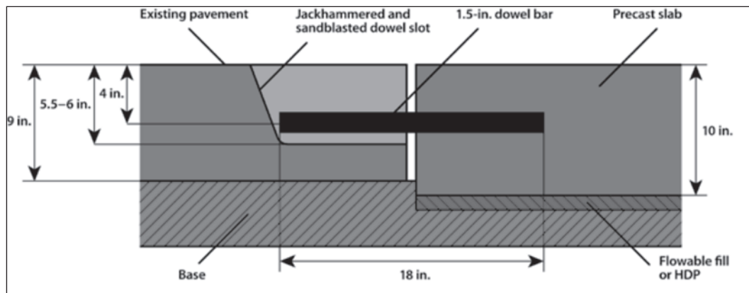
Figure 1. Michigan method cross-section of dowel assembly (Buch 2003).
