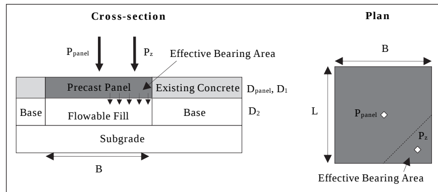
Figure 45. Schematic of bearing capacity modeling.
