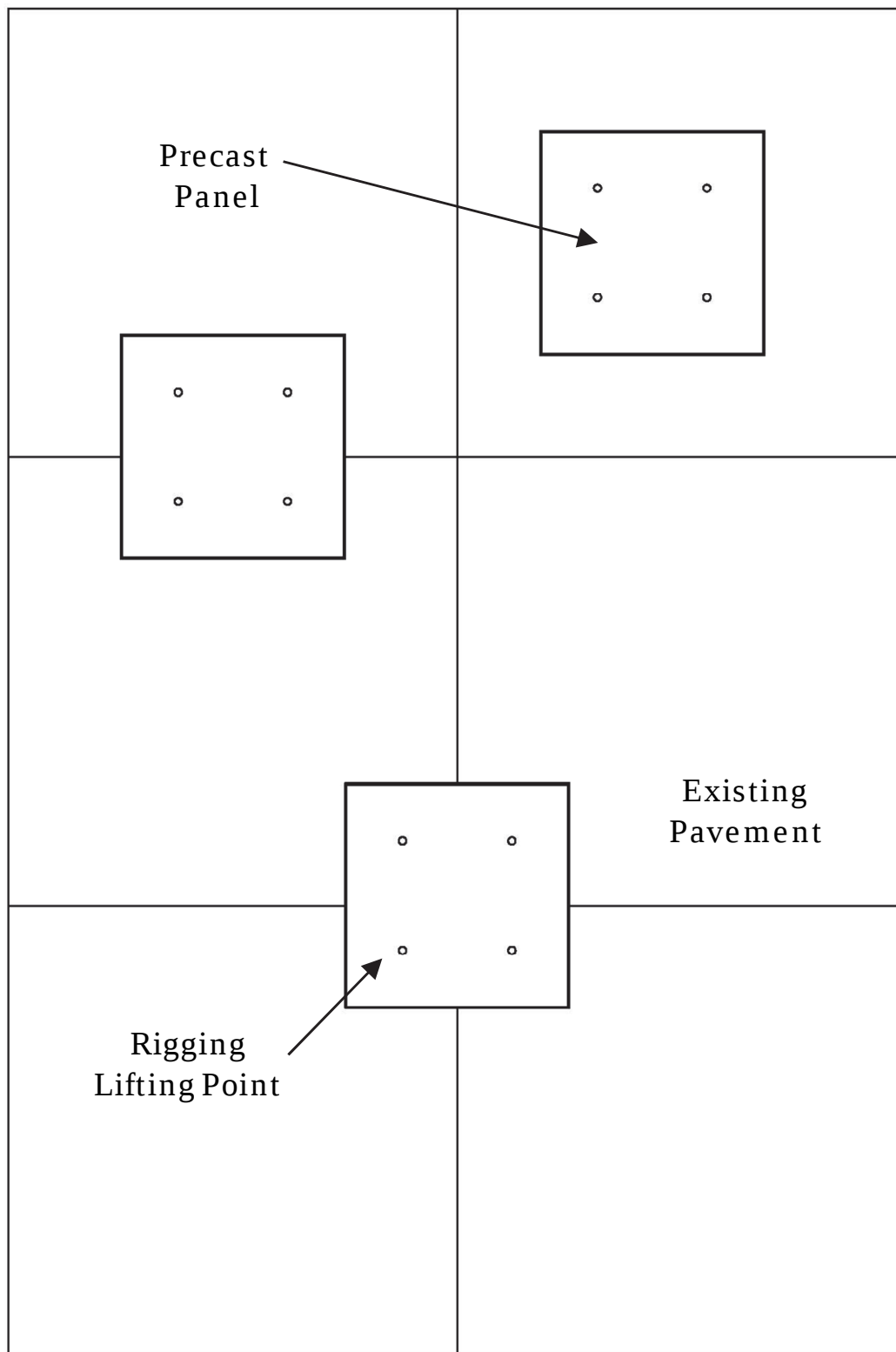
Figure 12. Nonstandard configurations.
