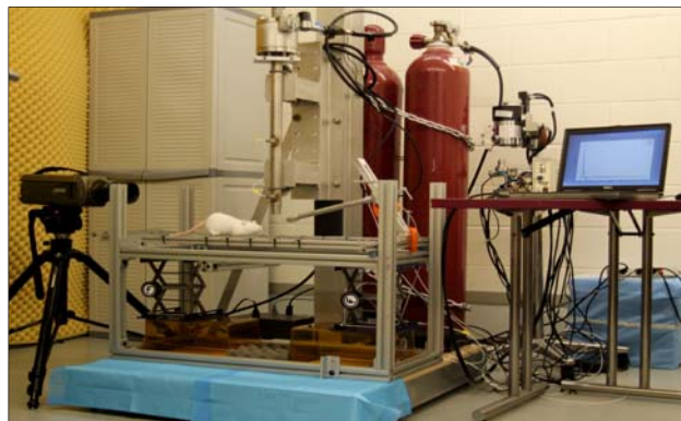
Fig.2 Overview of shock tube and experimental blast model facility at Banyan Biomarkers, Inc.
