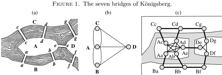
FIGURE 1. The seven bridges of Königsberg.
