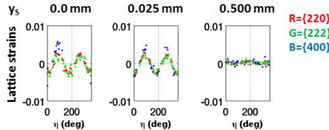
Figure 12: A subset of the lattice strains measured in normal incidence ( z_S parallel to the incident beam path) at various y_S positions for three crystallographic planes.
