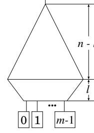
Figure A.1. Partition of MDD.
