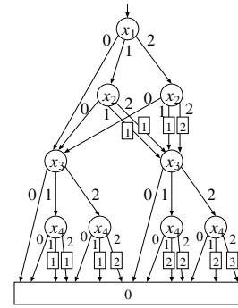
Figure 3. EVMDD for the structure function.
