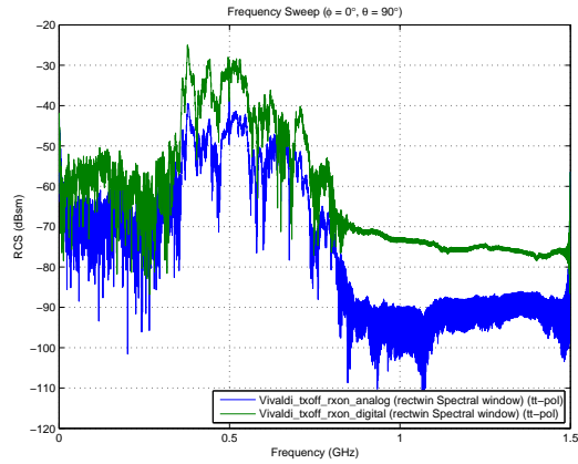
(b) Transmit filters off, received filters on
