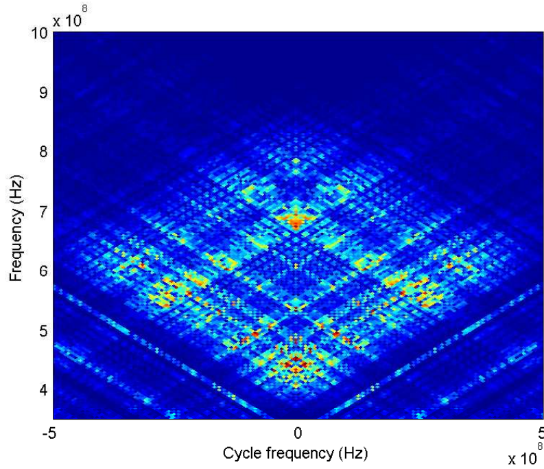
Figure 4.18: Digital source transmission cyclostationary analysis at SNIR = 5.97 dB zoomed in on top quadrant, with the color axis adjusted to better view features
