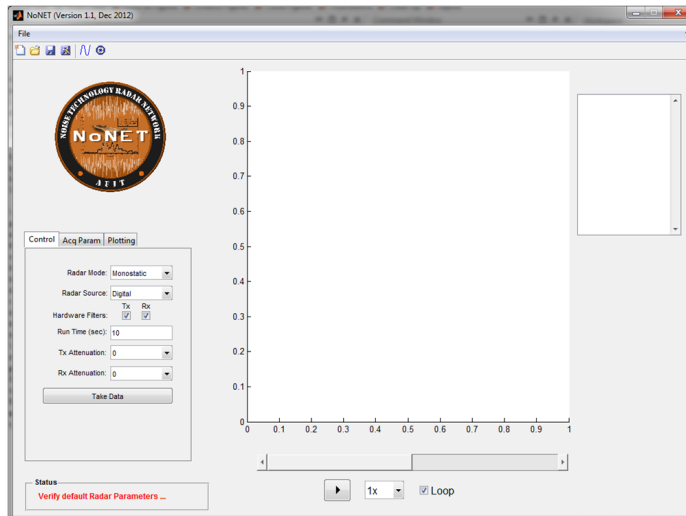
Figure C.4: NoNET GUI
