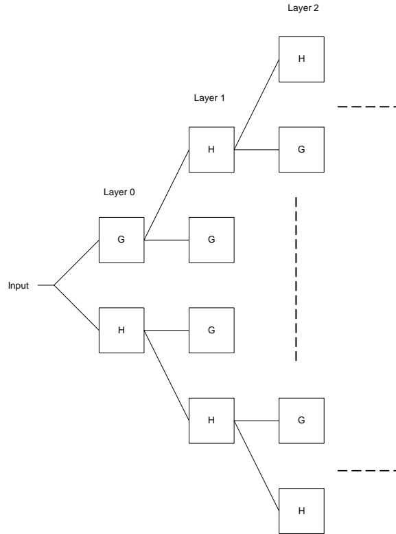
Figure 2.6: A QMFB tree diagram [18]
