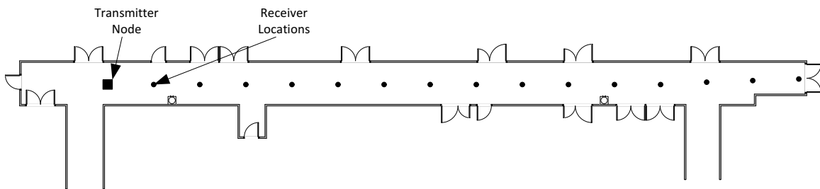
Figure 3.12: Diagram of communication experiment setup
