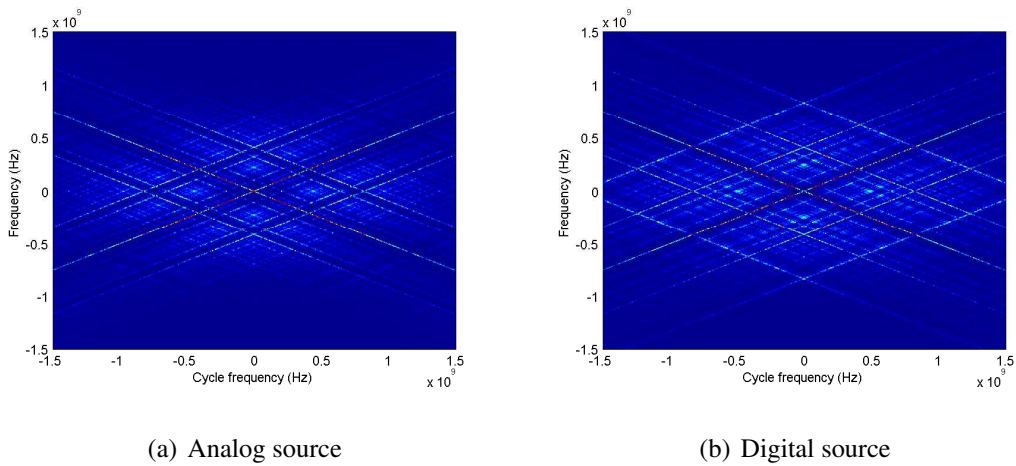
Figure 4.19: Analog and digital source transmitted waveform cyclostationary process at SNIR equal to -24 dB
