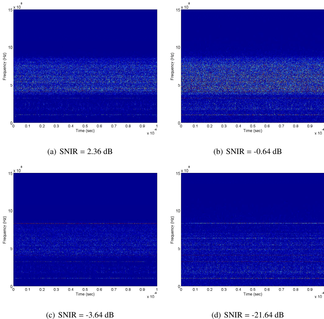
Figure 4.14: Analog source transmitted waveform QMFB layer 9 color plots at approximately various SNIR
