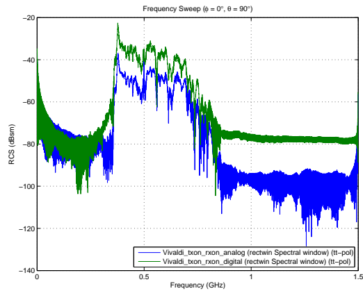
(d) Transmit filters on, received filters on
