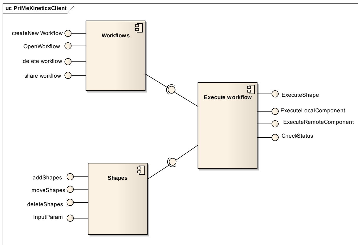
Figure 16. General PriMeKineticsClient.dll structure
