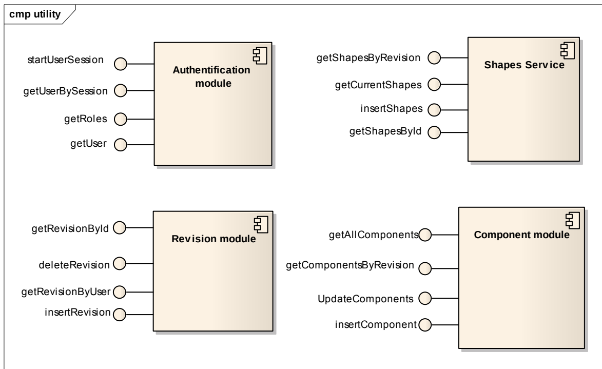
Figure 7. Utility.dll structure
