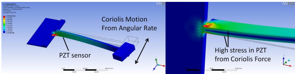
Figure 10. ANSYS modal analysis showing the Coriolis force sensing mode shape, in-plane motion and relative strain along the sides of the high aspect ratio beam due to the sideways motion.
