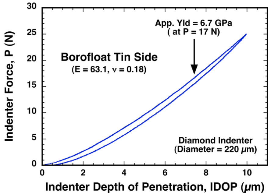
Figure 3.4. Example of a generated load-unload profile from a spherical indentation test.
