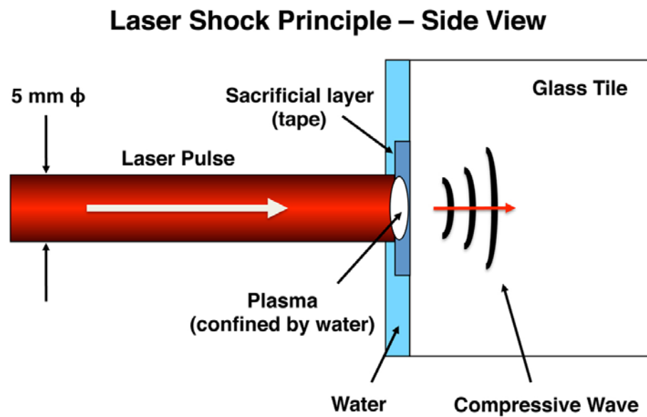
Figure 5.2. Schematic of laser shock process.
