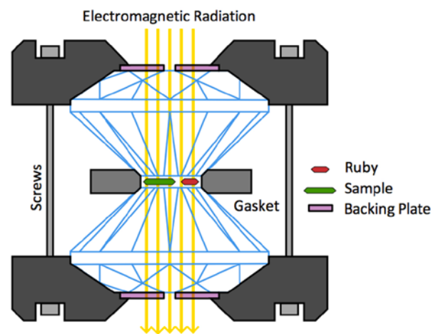
Figure 4.1. Schematic of the diamond anvil cell test.
