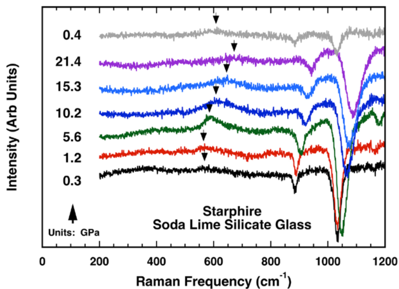
Figure 4.6. Raman spectrum as a function of stress for Starphire soda lime silicate glass.
