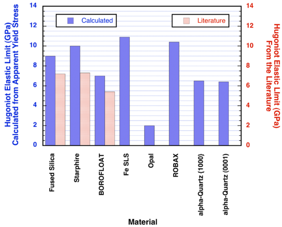
Figure 3.10. Comparison of the calculated Hugoniot Elastic Limit from apparent yield stress values with literature HEL values.
