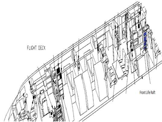
Figure 17. C-5 Flight Deck Raft Location
