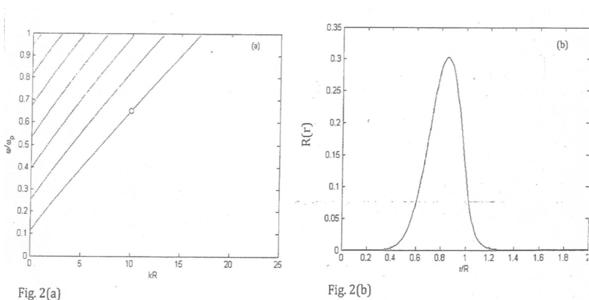
Figure 2. Dispersion Curves of S-Polarized Surface Plasmon Polaritons on a Circular Boundary
