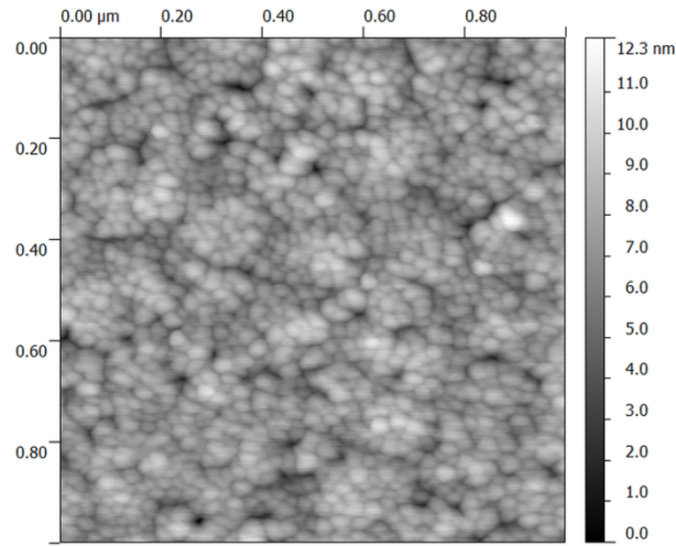
Figure 9: 1x1 μm AFM of p-type GaN:Mg film (RMS roughness = 1.27 nm).
