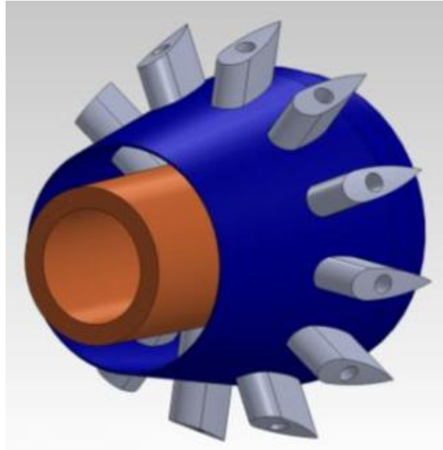
Figure 3.15: MD, support vanes and ID
