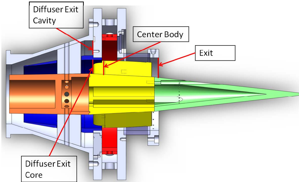
Figure 3.3: Mach number locations
