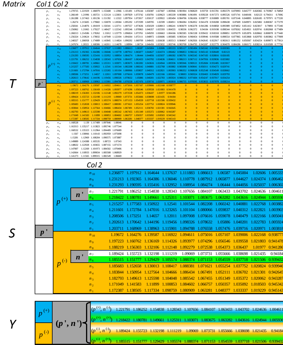
Figure 3.15. Trimming of the lookup table T to sub-matrix S , and finally a matrix of only nearest neighbors data, matrix Y . Only numeric entries comprise actual T , S , and Y .
