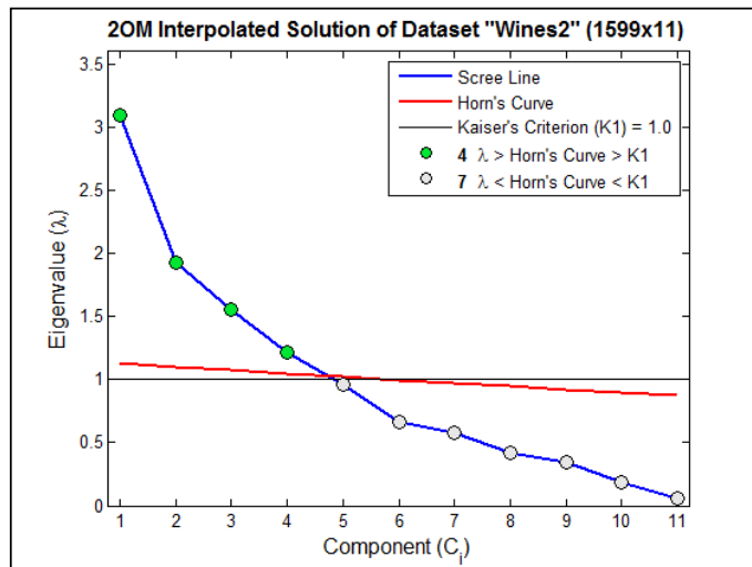
Figure AI10. Dataset Wine Quality (Cortez, Cerdeira, Almeida, Matos, & Reis, 2009)
