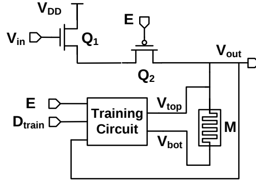
Figure 5. Synapse together with training circuit
