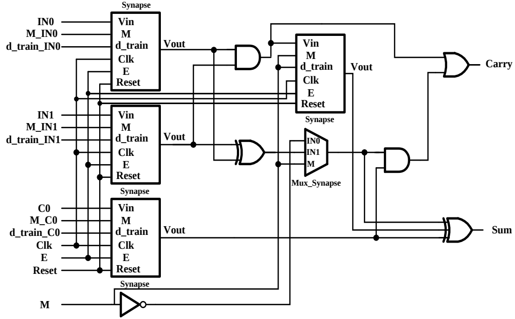
Figure 15. Schematic of the modified adder-subtractor block to realized Eq. (9c)
