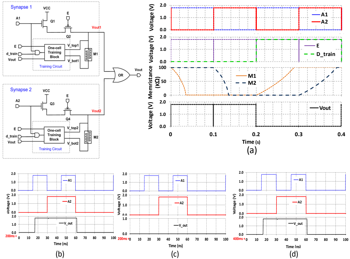
Figure 25. The 2-synapse training circuit an simulation results
