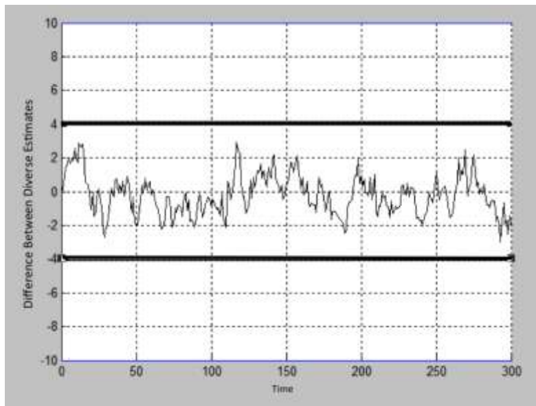
Figure 11. Simulation-based time-series of differences between the operator displayed and diversely redundant estimates of \underline{x}_1 , under normal system operation.
