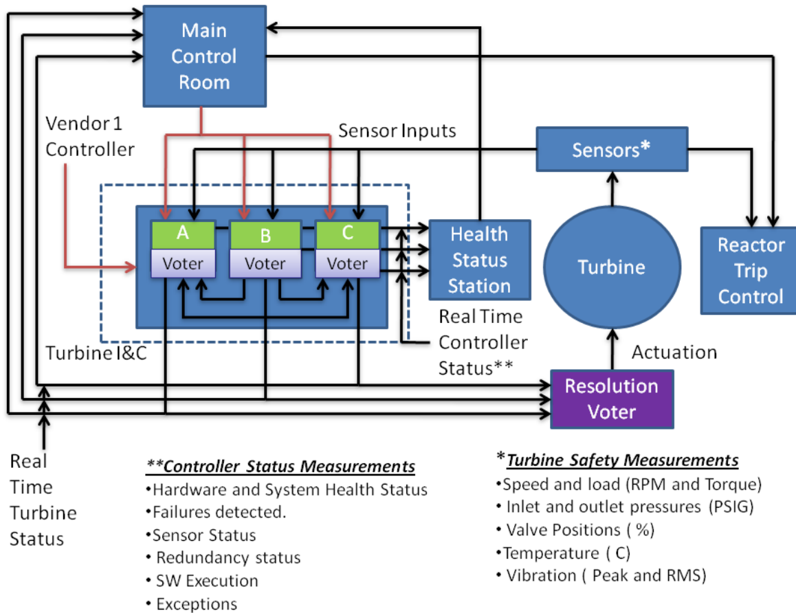
Figure 2: A high-level system diagram for a typical steam fed nuclear reactor powered turbine control system. The turbine controller is designed to meet high reliability and safety standards by employing redundancy and a resolution voter.
