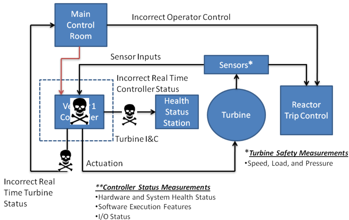
Figure 3: Illustration of a hypothetical cyber attack on a turbine control system. The controller is embedded with a Trojan horse that can modify, nullify, or replace information sent to the operators in the Main Control Room and the automatic monitoring station. The intended consequence of the attack would be to have the operator(s) believe that the turbine is operating sufficiently outside of specification so as to warrant a procedural action (e.g., shutdown of the turbine), which would induce a plant trip.
