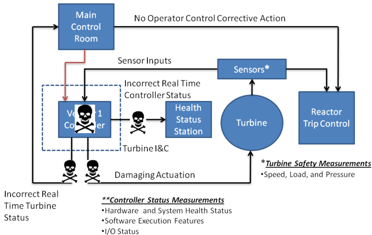
Figure 4: Illustration of a hypothetical cyber attack on a turbine control system. The controller is embedded with a Trojan horse that can modify, nullify, or replace information sent to the operators in the Main Control Room, Health Status Station, and the actuation commands sent to the Turbine. The consequence of a successful attack would be to create severe damage to the turbine, as well as to trip the reactor by sending disruptive control signals to damage the turbine and manipulating control information sent to the Main Control Room.
