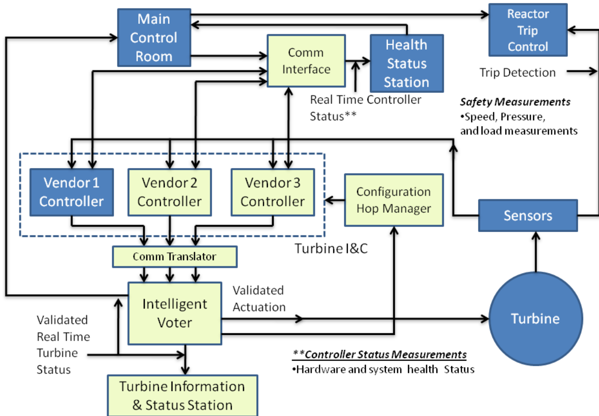
Figure 5: Possible System-Aware security architecture to address the threats illustrated in Figure 3 and Figure 4. This includes three controllers in the system architecture and an intelligent voting process to rapidly disable a differentiated controller from carrying out its turbine actuation functions.
