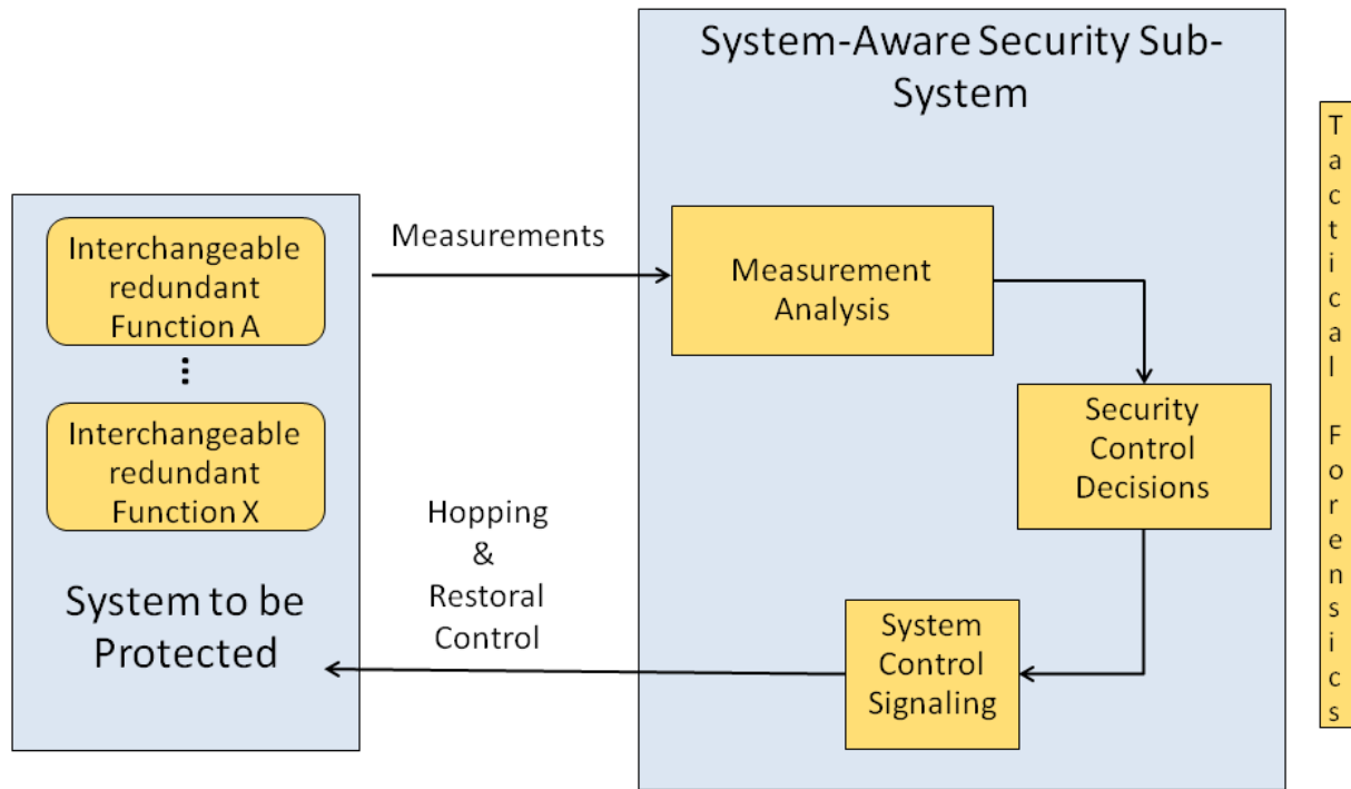
Figure 1: A high-level block diagram of the System-Aware Cyber Security Architecture, including measurement features for attack detection and tactical forensics, decision functions for system control, and signaling functions for managing system restoration and configuration hopping.
