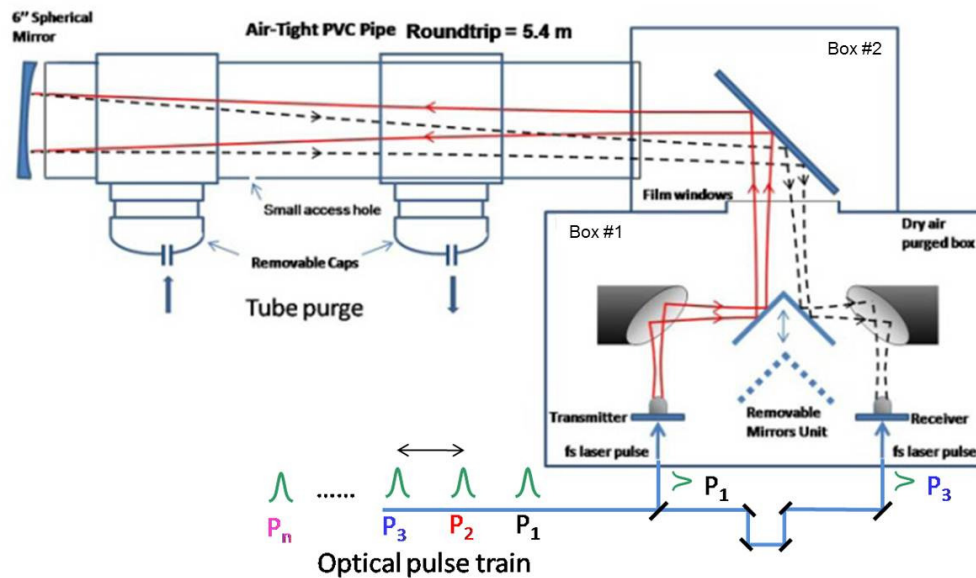
Fig. 2. Long-tube apparatus based on a standard THz-TDS spectrometer. A pair of removable mirrors deflects the THz beam out of the spectrometer and into Box #2. The beam then enters a 5.4 meter round trip path length enclosed tube for vapor measurements. The THz pulse returned to the receiver is gated by the 2 nd pulse (P3) down train from the pulse that excites the transmitter (P1).
