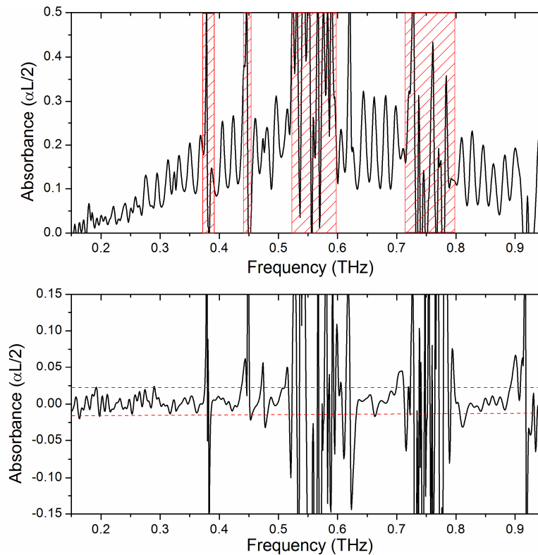
Fig. 9. (Top) Amplitude absorbance spectrum for \text{CH}_3\text{CN} vapor at 800 ppm in the 1.2 m (round-trip) sample chamber measured using the 170 meter long-path apparatus. The laboratory relative humidity was 50%. The hatched areas indicate regions of complete water vapor absorption. The curve is the average of six signal and reference measurements (Bottom) Noise baseline from the average of six pairs of reference measurements. The red horizontal bars provide a qualitative measure of the noise level in the amplitude absorbance.
