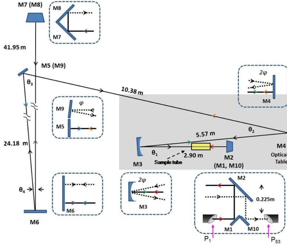
Fig. 3. Schematic from the top (x-z plane) of the 170 meter round trip long path apparatus consisting of 10 mirrors. Insets: Side view (y-z plane) of the mirrors. The solid lines show the path of the THz beam deflected out of and into the spectrometer by the mirror pair M1 and M10. The position of the THz-TDS spectrometer is shown in the inset and lies underneath M2. The THz pulse returned to the receiver is gated by the 52 nd pulse down the laser pulse train from the excitation pulse. The indicated angles are \theta_1 = 5.4^\circ , \theta_2 = 19^\circ , \theta_3 = 77^\circ , \theta_4 = 2.4^\circ , and \phi = 1.25^\circ .
