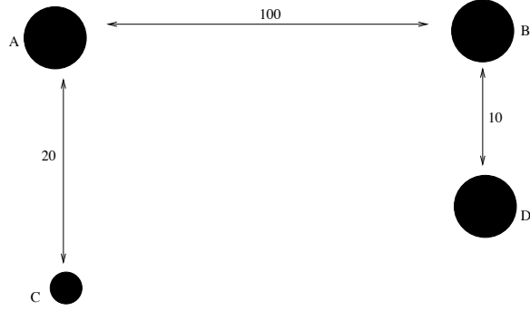
Figure 8.4: An example showing that the usual version of Single-Linkage fails. The instance is composed of 4 components, each with inner-distance \epsilon and outer-distance as described in the figure. However, components A, B and D each contain 100 points, whereas component C has only 10 points. The optimal 3-median clustering consists of 3 clusters: \{A, C\}, \{B\}, \{D\} and has cost \text{OPT} = 200 + 300\epsilon .
