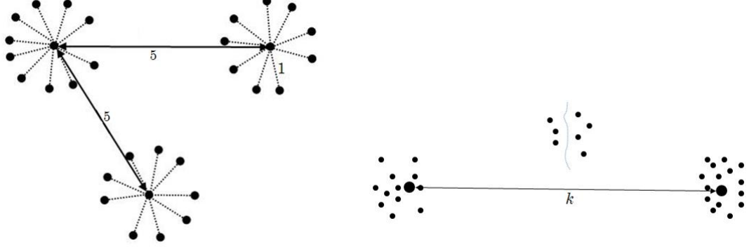
(a) Instance satisfying perturbation resilience but isn't weak-deletion stable. The distance of any point to its cluster center is 1 and distances between two different centers is 5 and remaining distances are short-path distances. With k clusters, each with \frac{n}{k} points, merging two clusters increases the cost by a sub-constant factor of O(1/k) .
