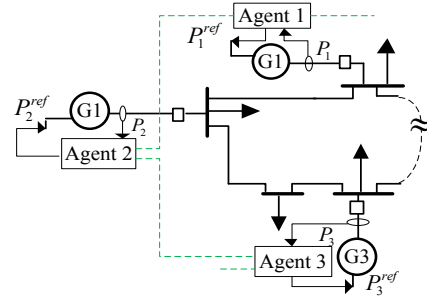
Fig. 1 Control system architecture
