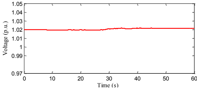
Fig. 11 Voltage response with the proposed solution
