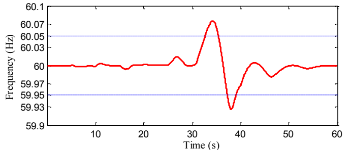
Fig. 10 Frequency response with the proposed solution
